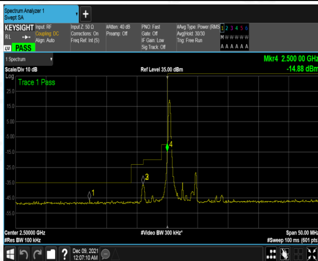
Band7-5MHz-QPSK-20775-1RB#24
