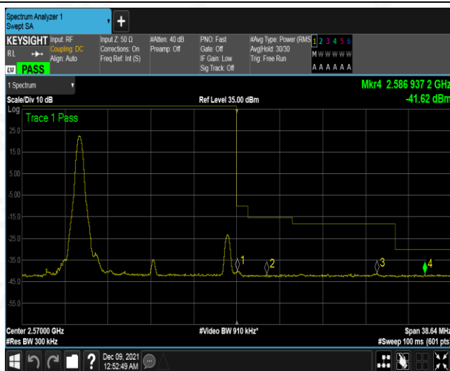
Band7-15MHz-QPSK-21375-1RB#74
