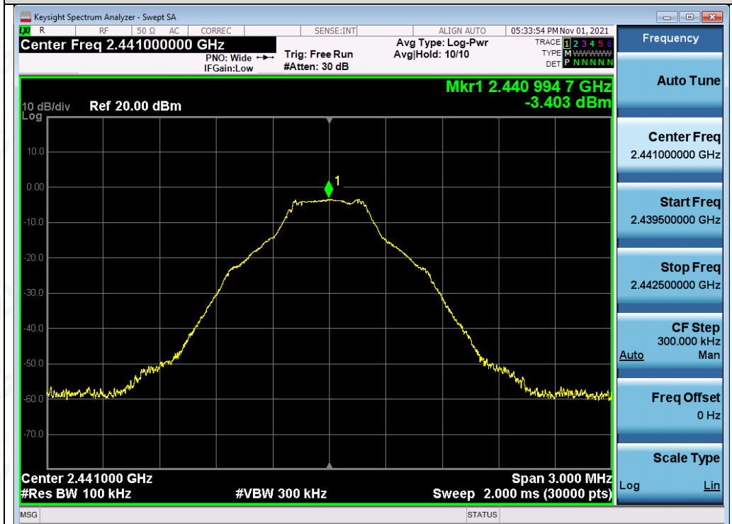
Test_Graph_BR_ANT1_2441_1Mbps_Reference Level
