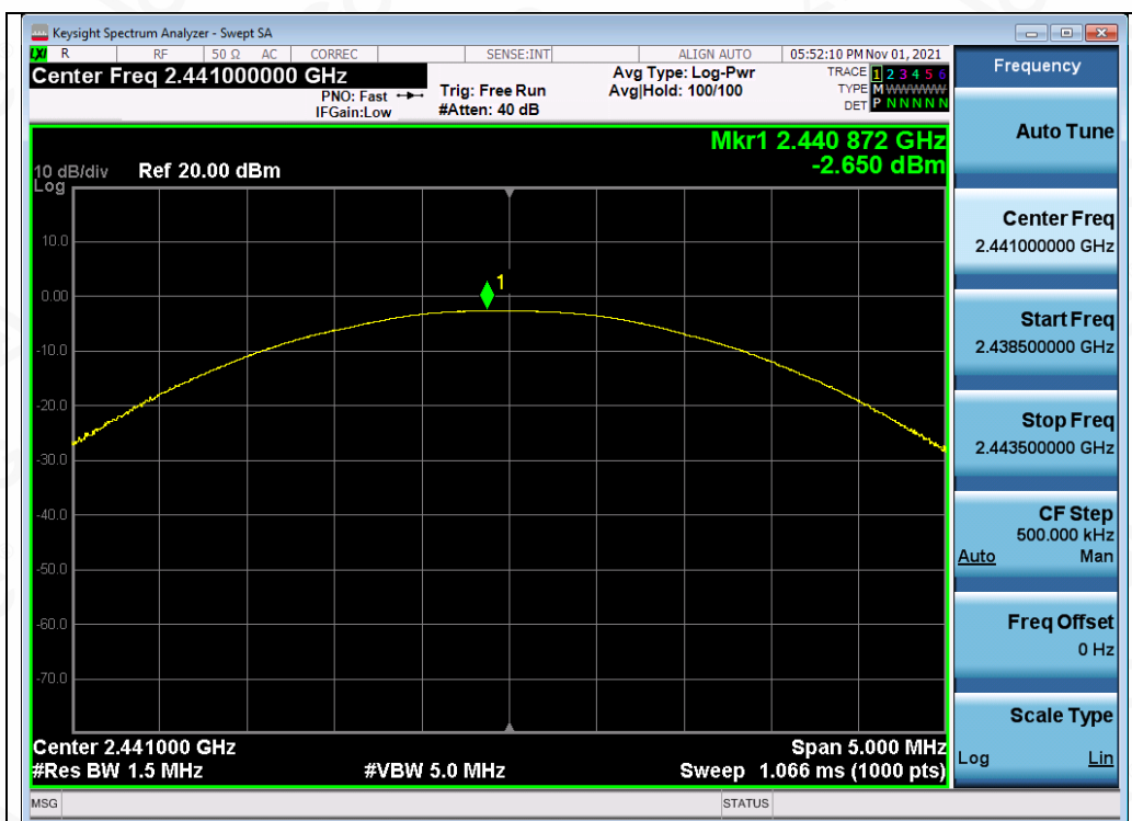
Test_Graph_EDR_ANT1_2441_3Mbps_Peak Power
