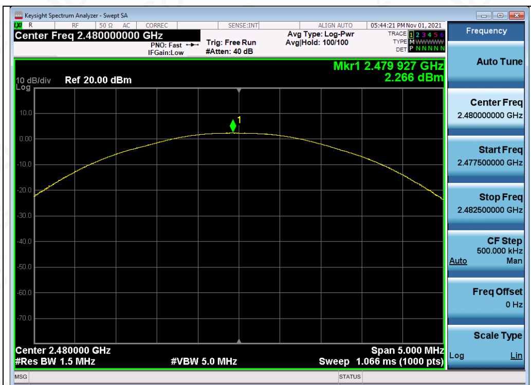
Test_Graph_EDR_ANT1_2480_2Mbps_Peak Power
