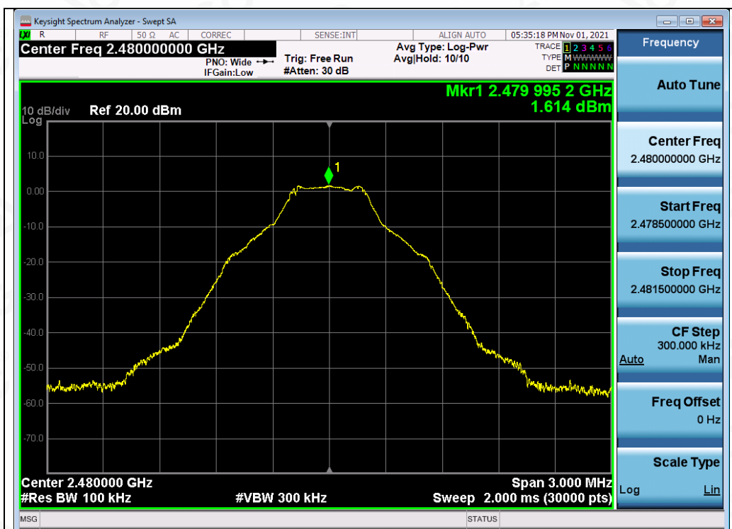
Test_Graph_BR_ANT1_2480_1Mbps_Reference Level
