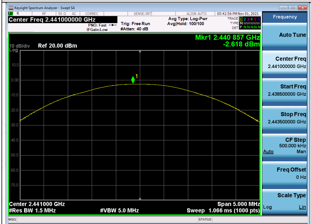
Test_Graph_EDR_ANT1_2441_2Mbps_Peak Power
