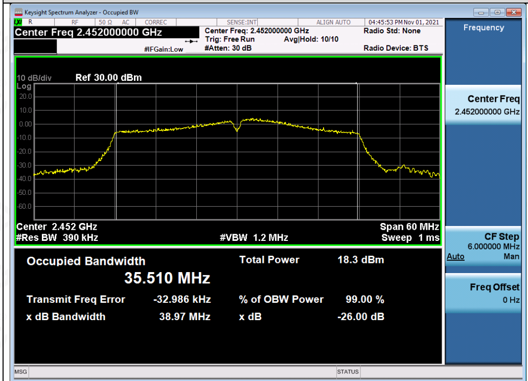
Test_Graph_802.11n40_ANT1_2452_MCS0_OBW
