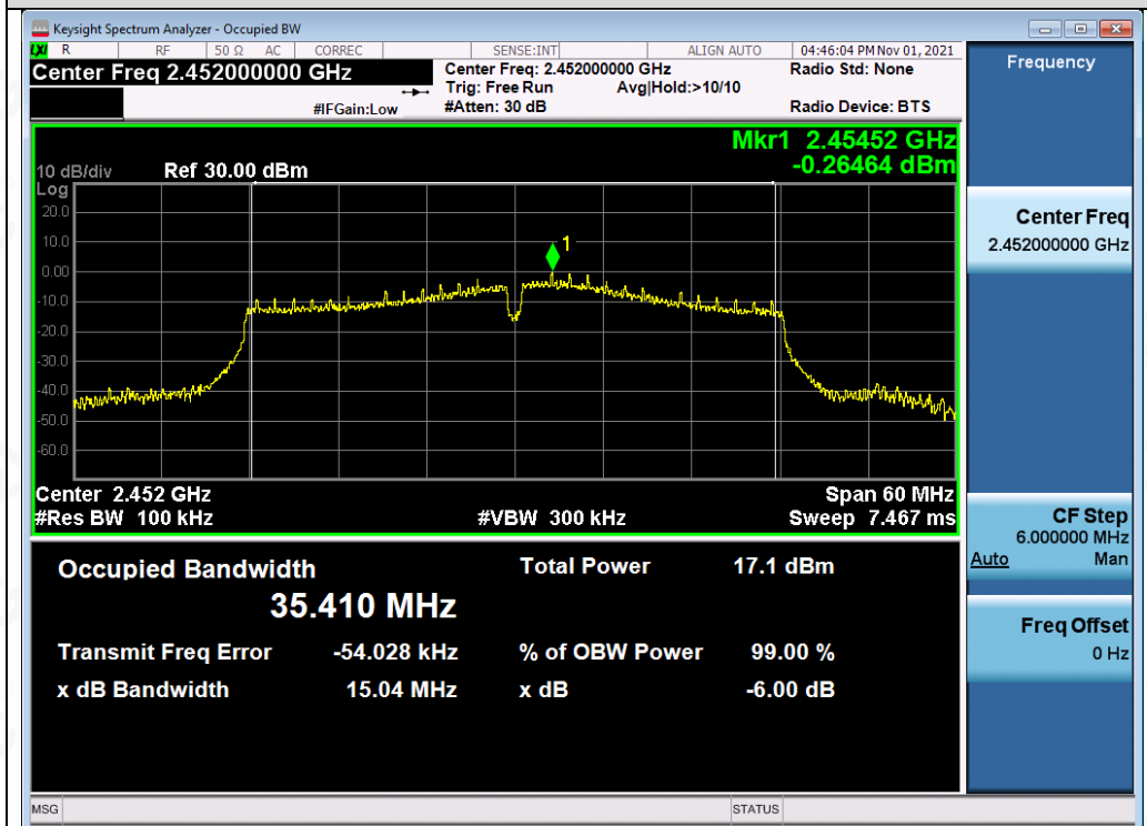
Test_Graph_802.11n40_ANT1_2452_MCS0_DTSBW
