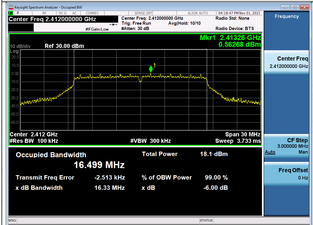
Test_Graph_802.11g_ANT1_2412_6Mbps_DTSBW
