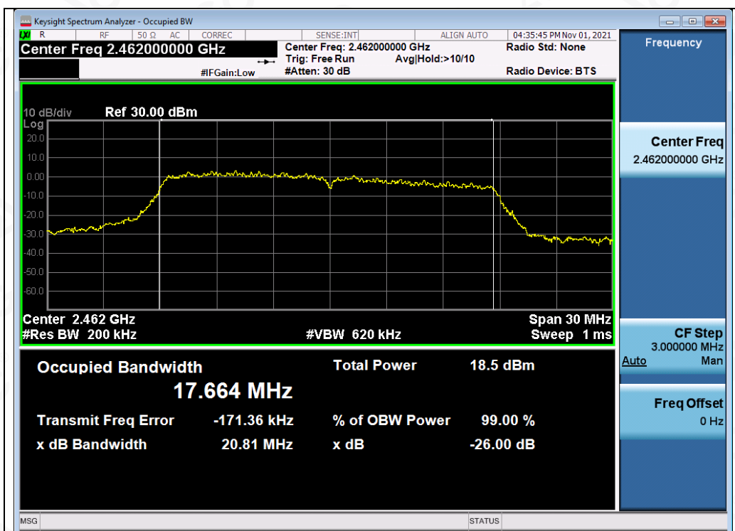
Test_Graph_802.11n20_ANT1_2462_MCS0_OBW
