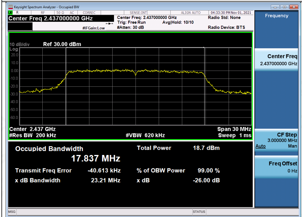
Test_Graph_802.11n20_ANT1_2437_MCS0_OBW
