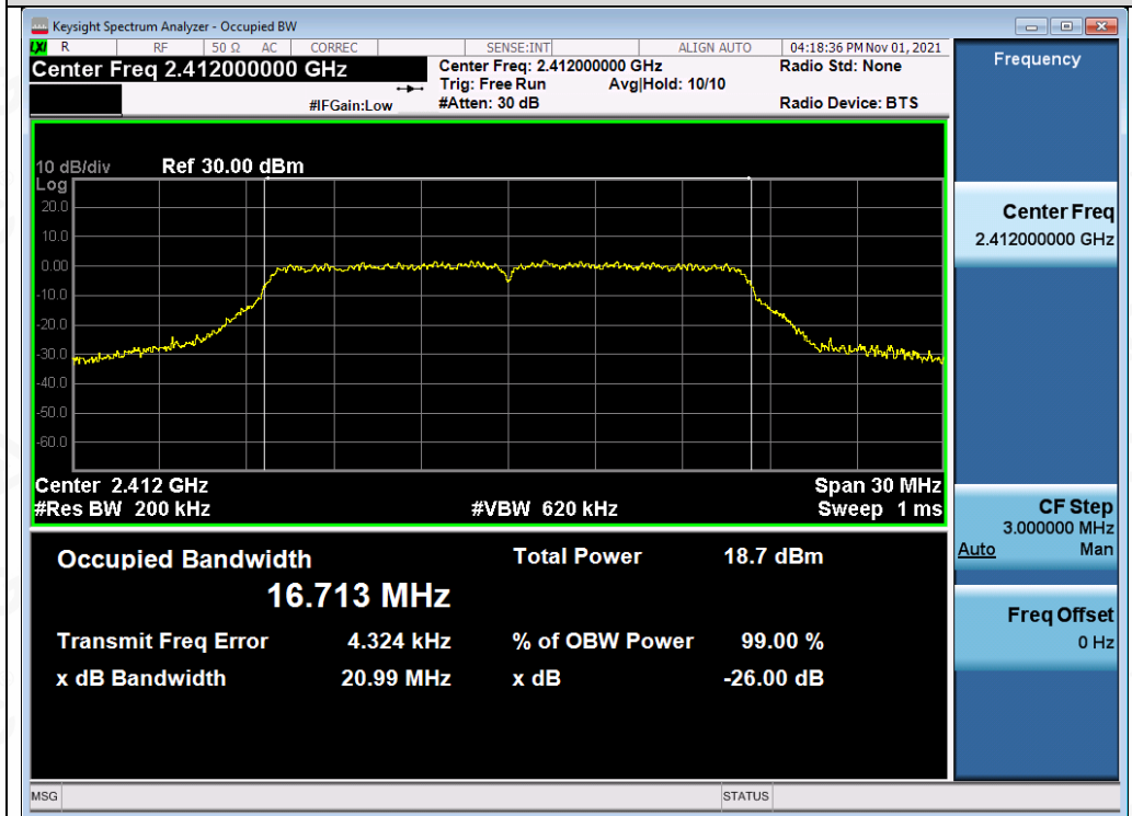
Test_Graph_802.11g_ANT1_2412_6Mbps_OBW
