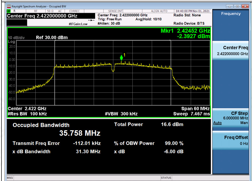
Test_Graph_802.11n40_ANT1_2422_MCS0_DTSBW
