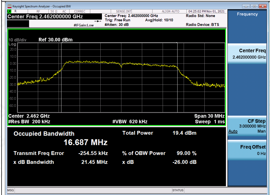
Test_Graph_802.11g_ANT1_2462_6Mbps_OBW
