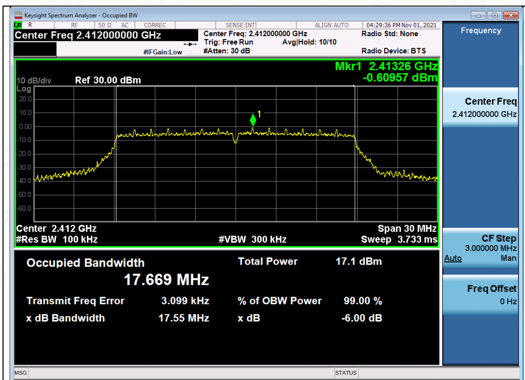
Test_Graph_802.11n20_ANT1_2412_MCS0_DTSBW
