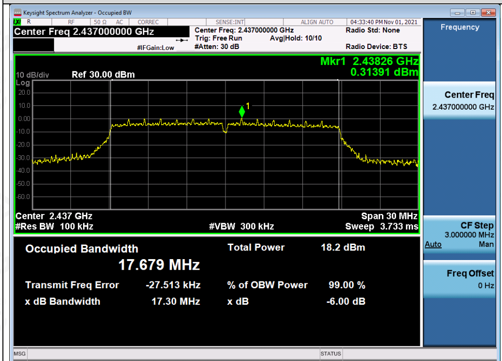
Test_Graph_802.11n20_ANT1_2437_MCS0_DTSBW
