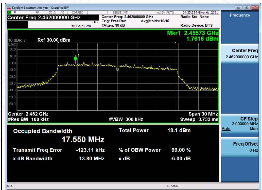
Test_Graph_802.11n20_ANT1_2462_MCS0_DTSBW
