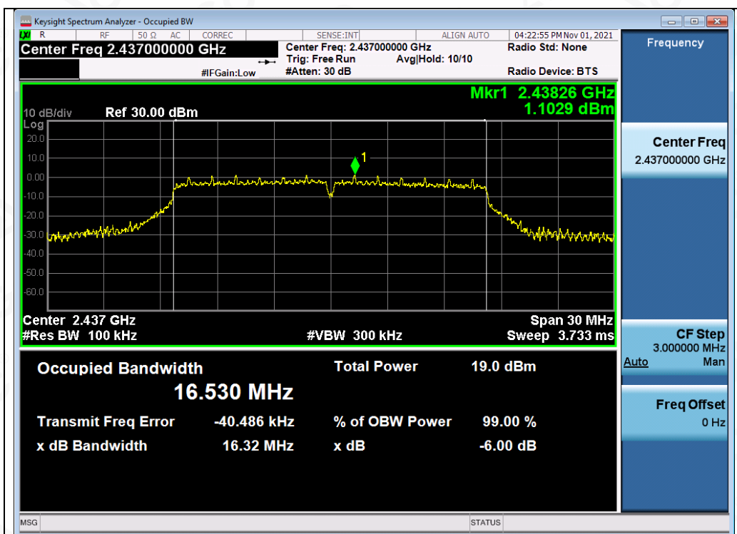
Test_Graph_802.11g_ANT1_2437_6Mbps_DTSBW
