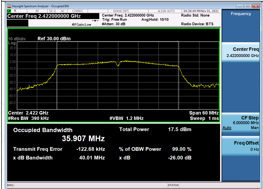
Test_Graph_802.11n40_ANT1_2422_MCS0_OBW
