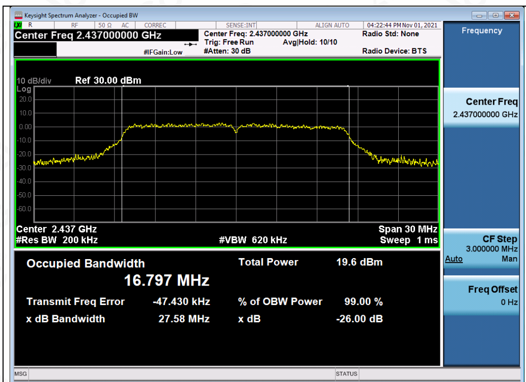
Test_Graph_802.11g_ANT1_2437_6Mbps_OBW
