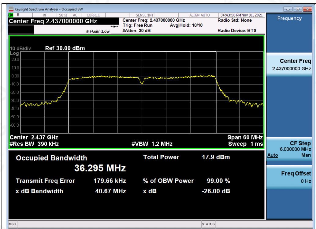
Test_Graph_802.11n40_ANT1_2437_MCS0_OBW
