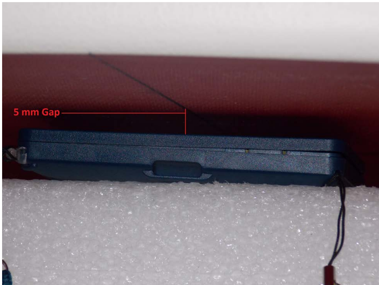
Test Position Side B with Lanyard 5 mm Gap
