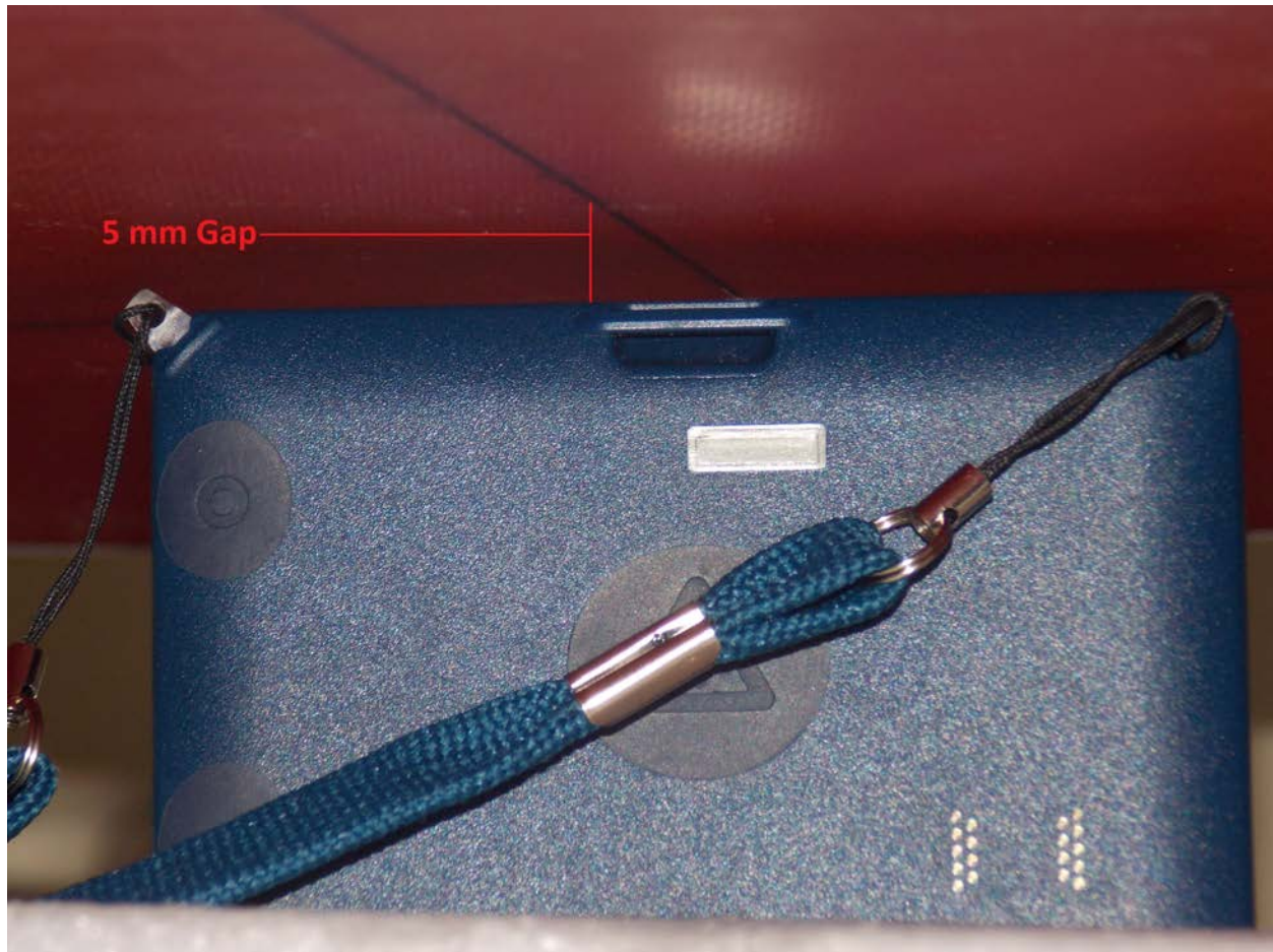
Test Position Side D with Lanyard 5 mm Gap
