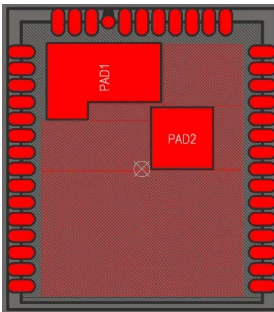
Figure 9: Landing Pads and Heat Sync Areas
