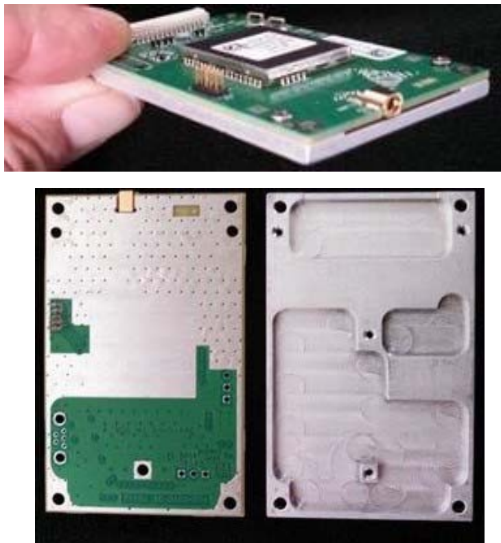
Figure 12: Carrier Board Heat Spreader
