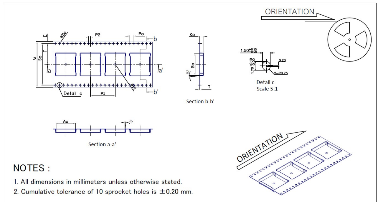
Figure 6: Tape and Reel Drawing
