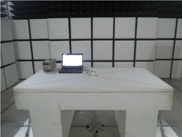
FCC_15_225 / RSS 210_NFC_Radiated_Setup
