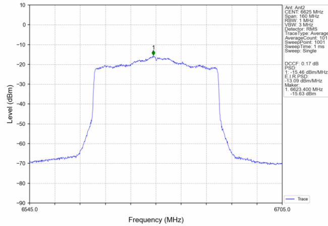
802.11ax(HEW80)_LCH_6625MHz_SU_/_MIMO_NTNV
