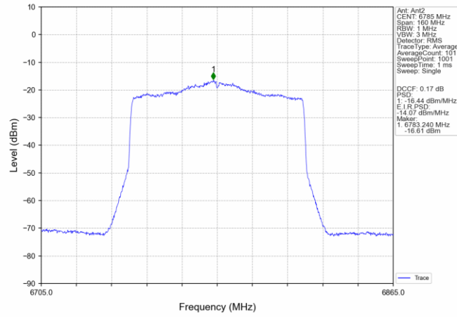
802.11ax(HEW80)_HCH_6785MHz_SU_ / _MIMO_NTNV
