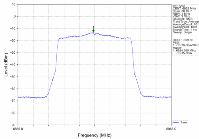
802.11ax(HEW40)_LCH_6925MHz_SU_ / _MIMO_NTNV
