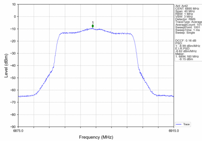
802.11ax(HEW20)_LCH_6895MHz_SU_ / _MIMO_NTNV
