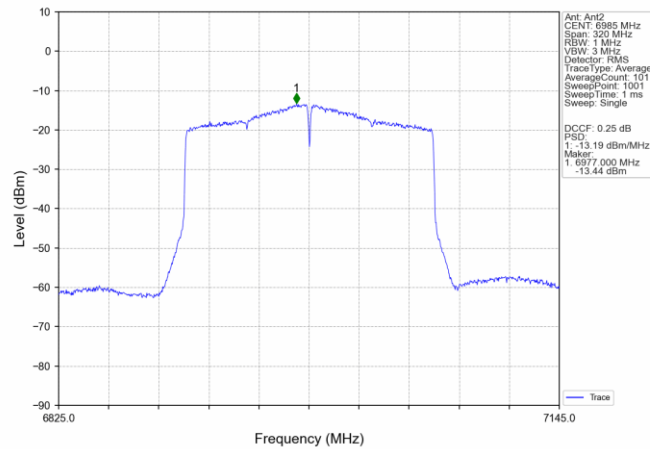
802.11ax(HEW160)_MCH_6985MHz_SU_ / _Ant2_NTNV
