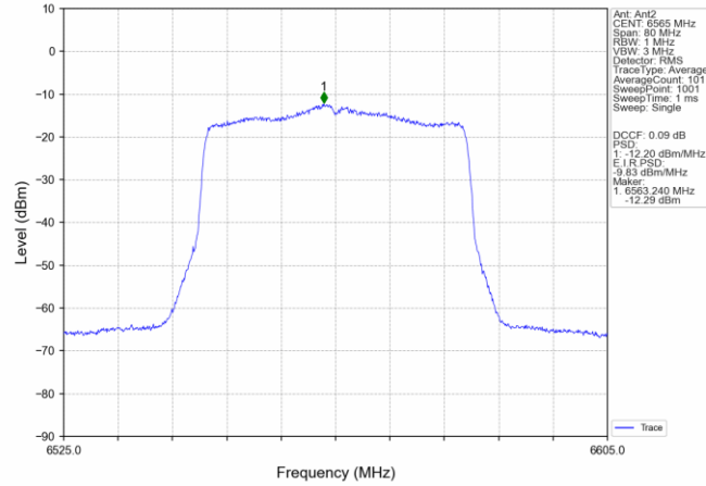
802.11ax(HEW40)_LCH_6565MHz_SU_/_MIMO_NTNV
