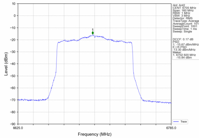
802.11ax(HEW80)_MCH_6705MHz_SU_/_MIMO_NTNV
