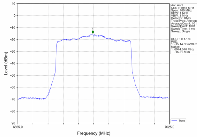
802.11ax(HEW80)_LCH_6945MHz_SU_ / _MIMO_NTNV
