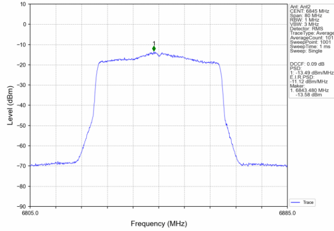
802.11ax(HEW40)_HCH_6845MHz_SU_ / _MIMO_NTNV
