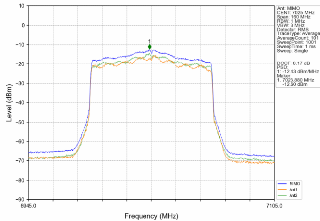
802.11ax(HEW80)_HCH_7025MHz_SU_ / _MIMO_NTNV
