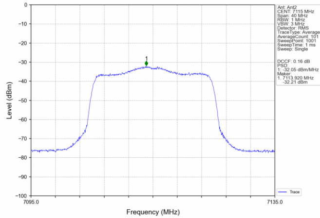
802.11ax(HEW20)_HCH_7115MHz_SU_ / _MIMO_NTNV
