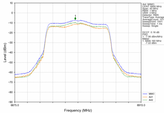
802.11ax(HEW20)_LCH_6895MHz_SU_ / _MIMO_NTNV
