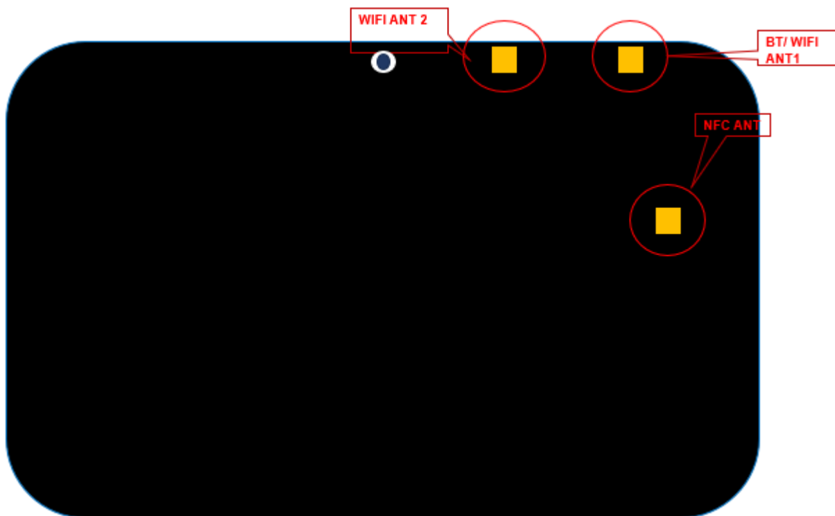
Front view
