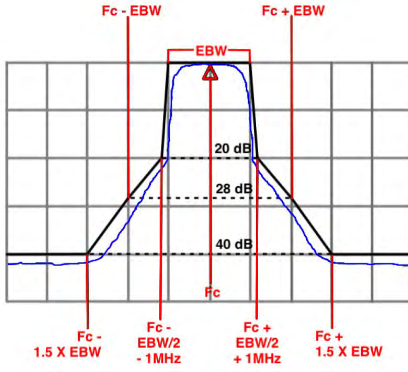
Generic Emission Mask
