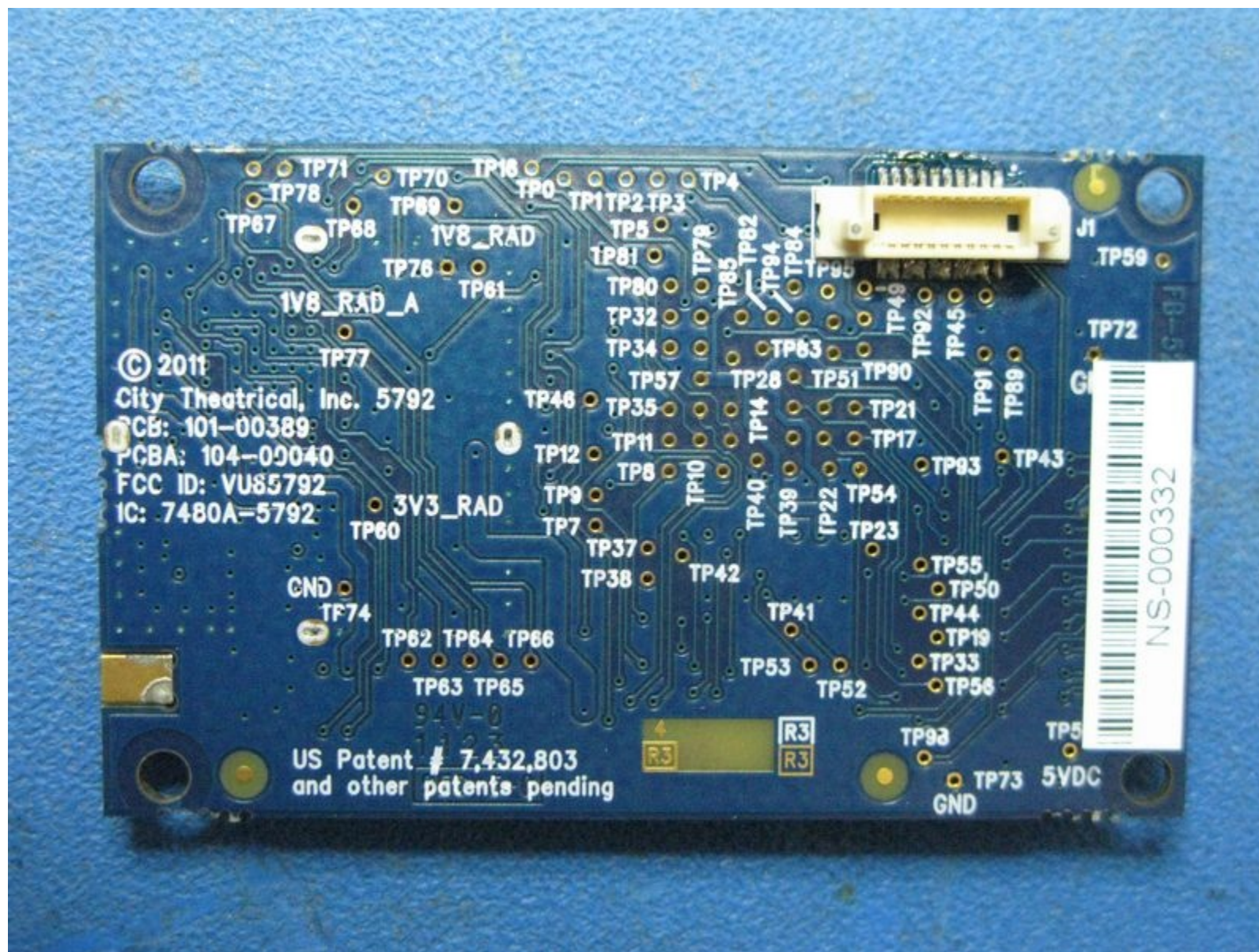
City Theatrical 5792 Radio Module bottom side
