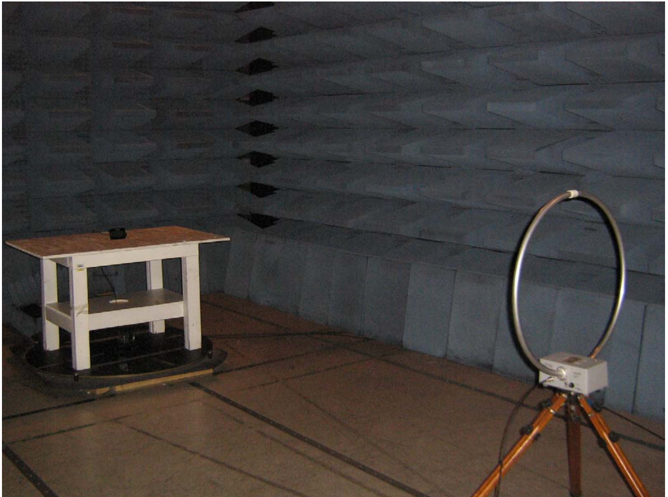
Typical Low frequency measurement test setup
