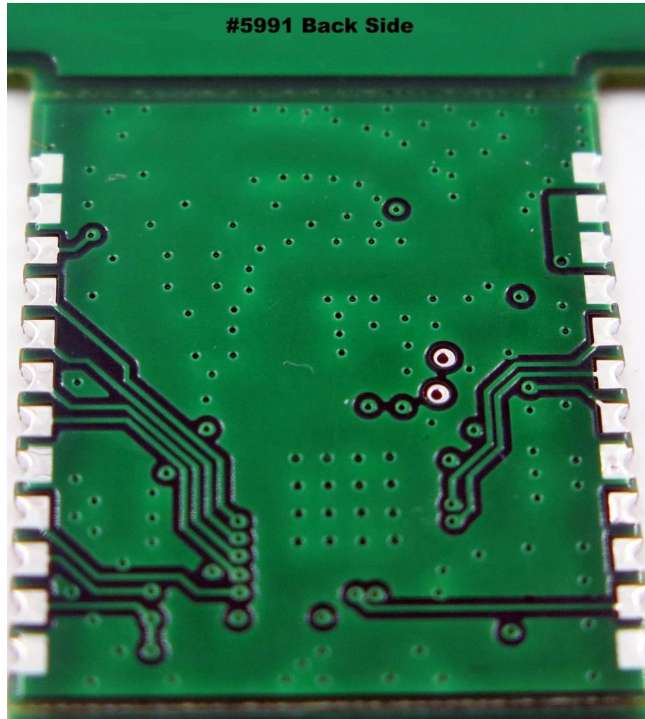
Fig. 2 Back View
