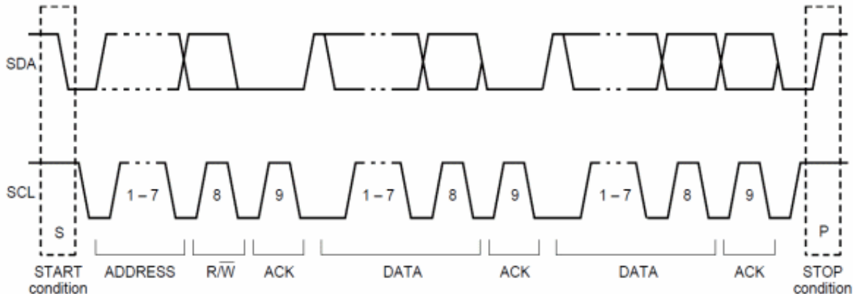
Figure 9: I2C Specification
