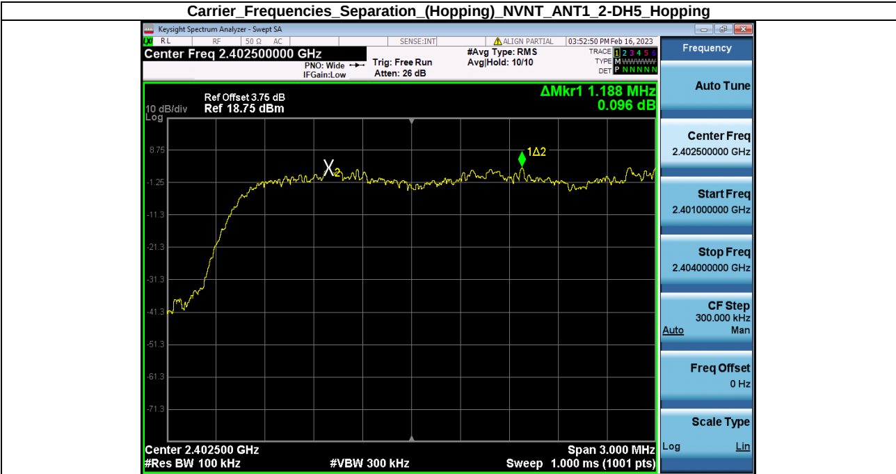
Carrier_Frequencies_Separation_(Hopping)_NVNT_ANT1_2-DH5_Hopping
