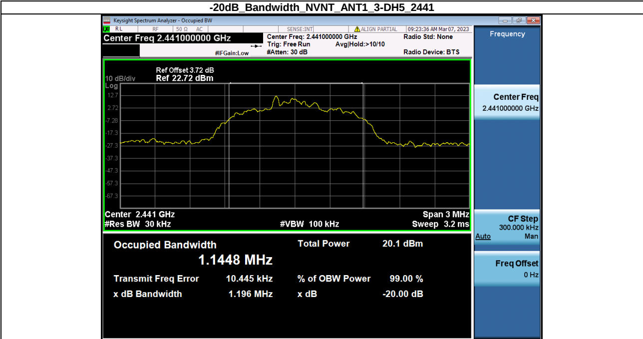
-20dB_Bandwidth_NVNT_ANT1_3-DH5_2441 -20dB_Bandwidth_NVNT_ANT1_3-DH5_2480
