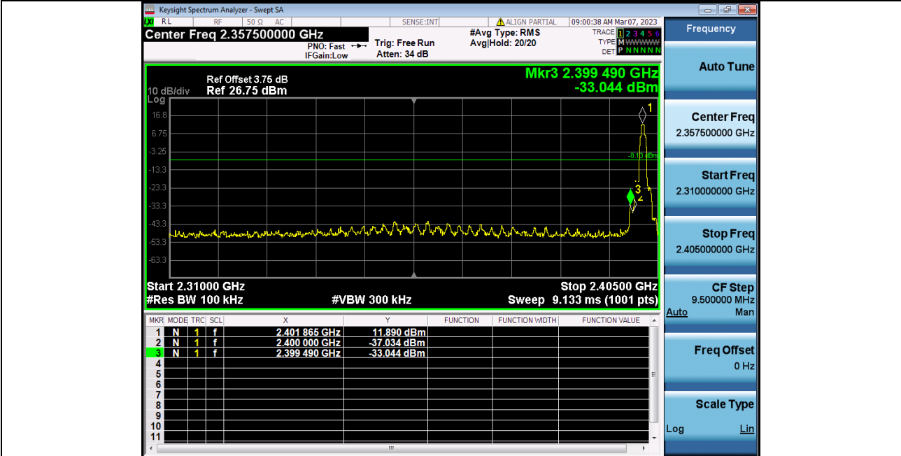
2_Bandedge_NVNT_ANT1_2-DH5_2402
