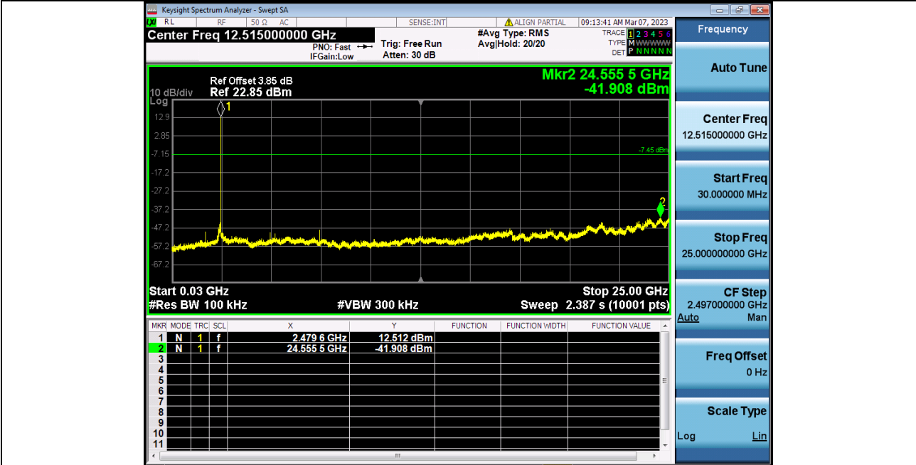
2_Spurious_Emissions_NVNT_ANT1_2-DH5_2480
