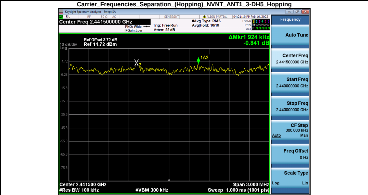
Carrier_Frequencies_Separation_(Hopping)_NVNT_ANT1_3-DH5_Hopping
