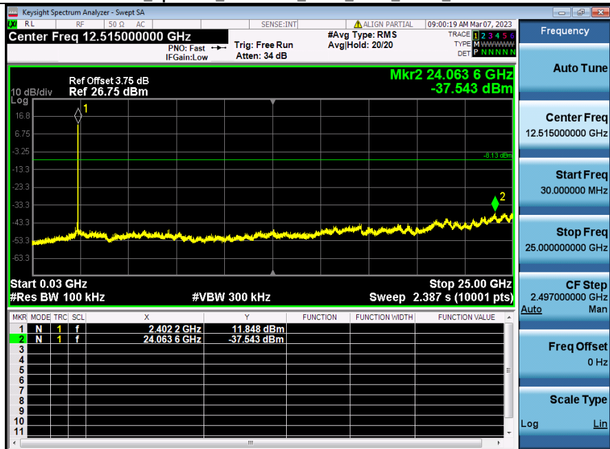
2_Spurious_Emissions_NVNT_ANT1_2-DH5_2402
