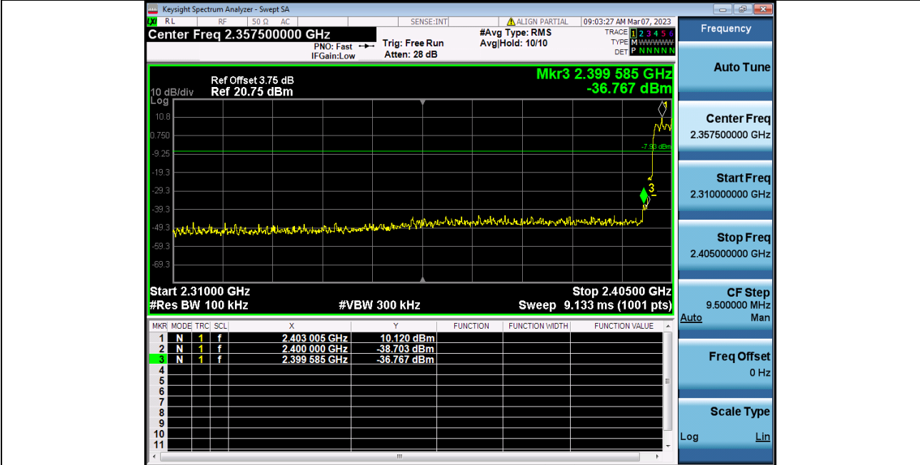
2_Band_Edge_(Hopping)_NVNT_ANT1_2-DH5_Hopping
