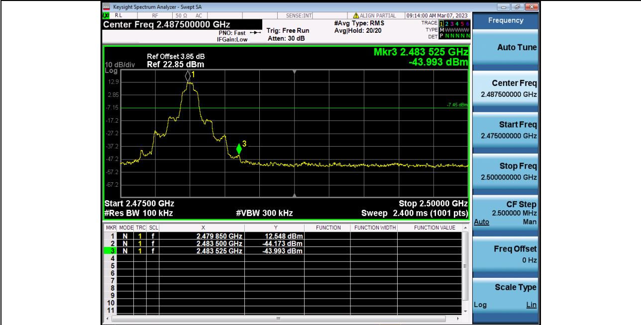
2_Bandedge_NVNT_ANT1_2-DH5_2480
