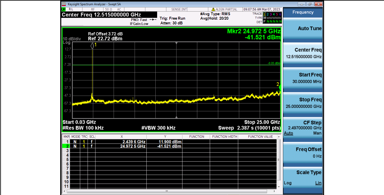
2_Spurious Emissions_NVNT_ANT1_2-DH5_2441
