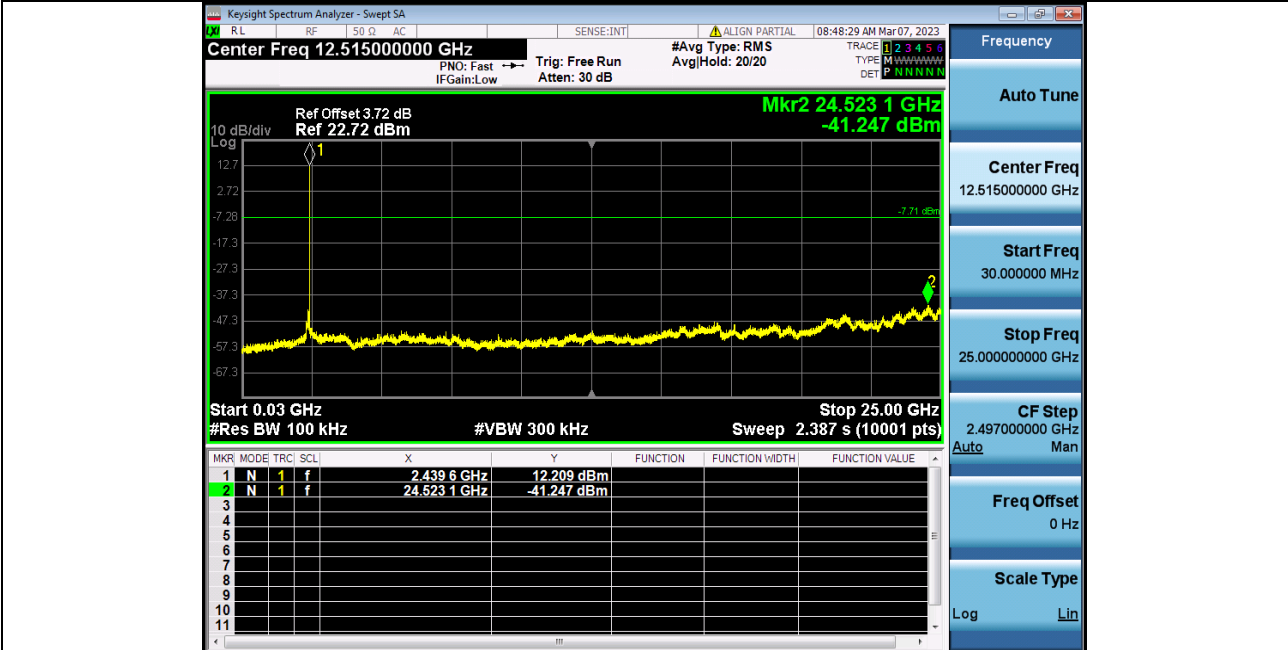
2_Spurious_Emissions_NVNT_ANT1_1-DH5_2441
