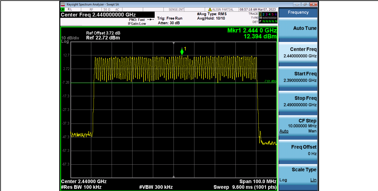
2_Band_Edge_(Hopping)_NVNT_ANT1_1-DH5_Hopping
