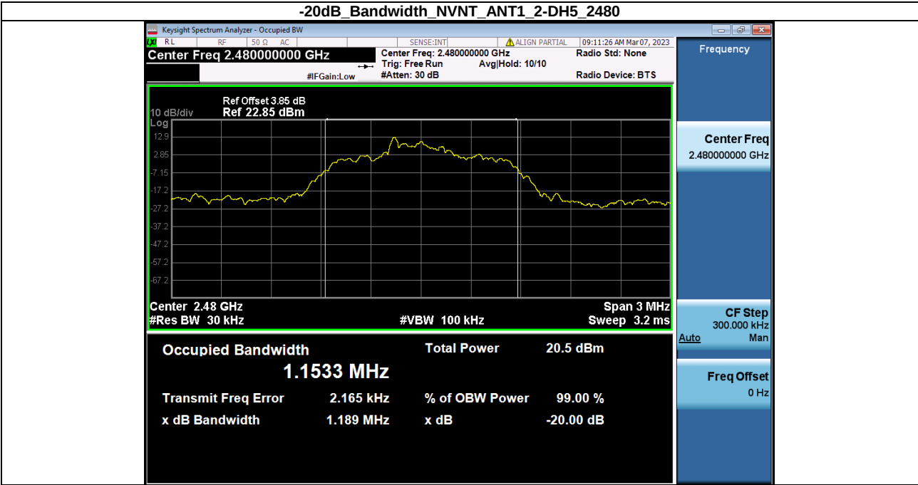
-20dB_Bandwidth_NVNT_ANT1_2-DH5_2480 -20dB_Bandwidth_NVNT_ANT1_3-DH5_2402
