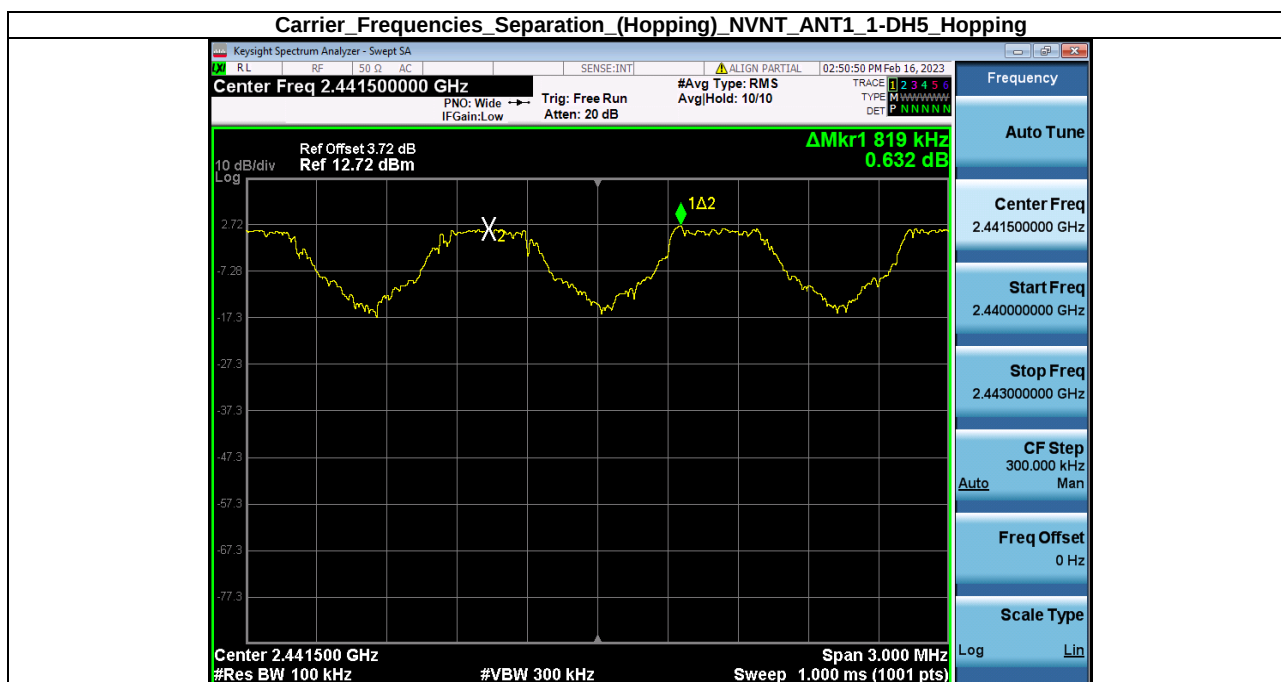
Carrier_Frequencies_Separation_(Hopping)_NVNT_ANT1_1-DH5_Hopping
