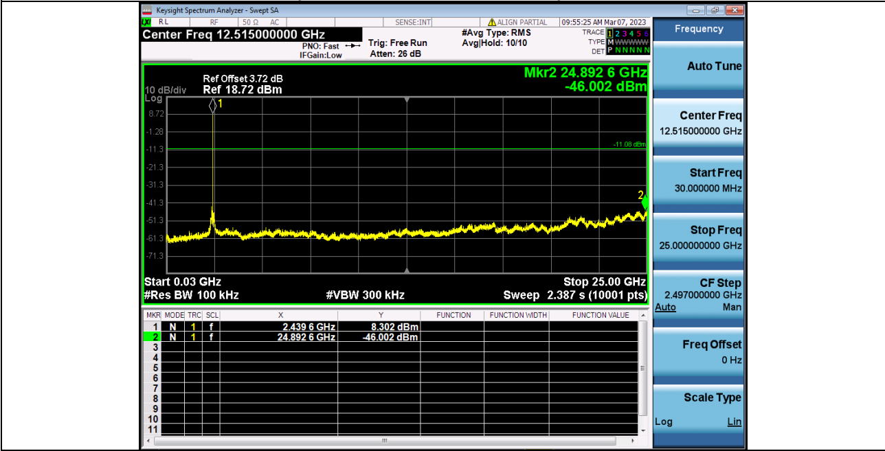
2_Spurious_Emission_NVNT_ANT1_1Mbps_2440
