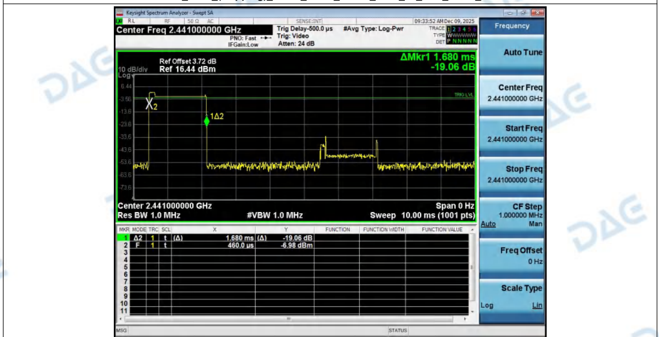
Dwell_Time_(Hopping)_NVNT_ANT1_2-DH3_2441_00_Accumulated
