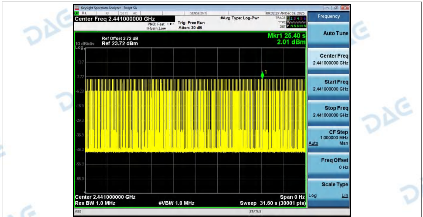
Dwell_Time_(Hopping)_NVNT_ANT1_2-DH3_2441_00_One_Burst_Time
