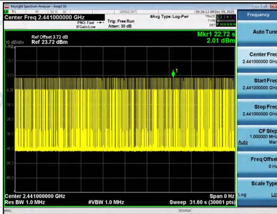
Dwell_Time_(Hopping)_NVNT_ANT1_3-DH3_2441_00_One_Burst_Time
