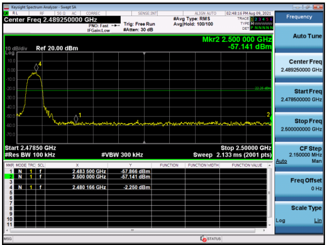
Channel 78 / 2480 MHz – Non-Hopping
