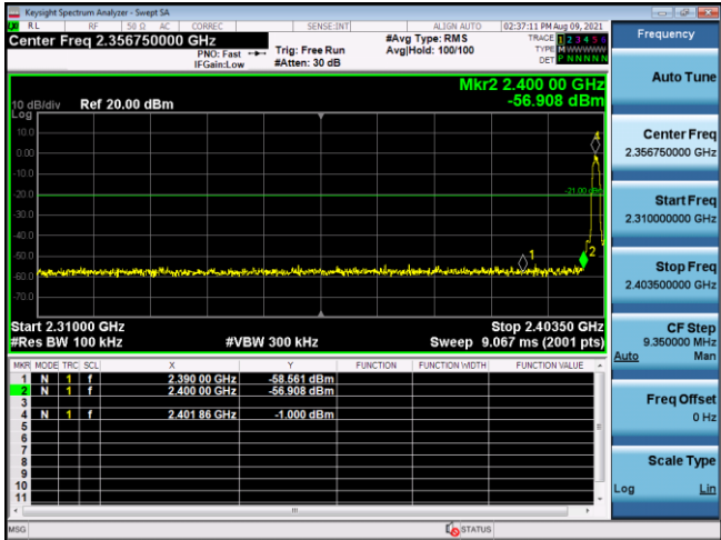
Channel 0 / 2402 MHz – Non-Hopping
