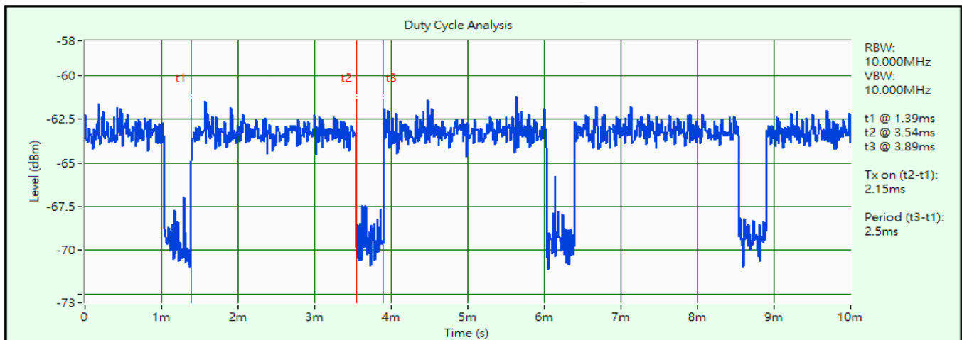
Time-domain plot for Bluetooth transmission signal
