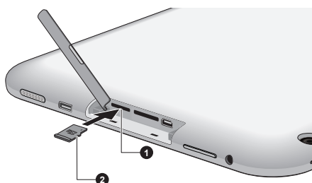
Figure 7-1 Inserting a memory media
