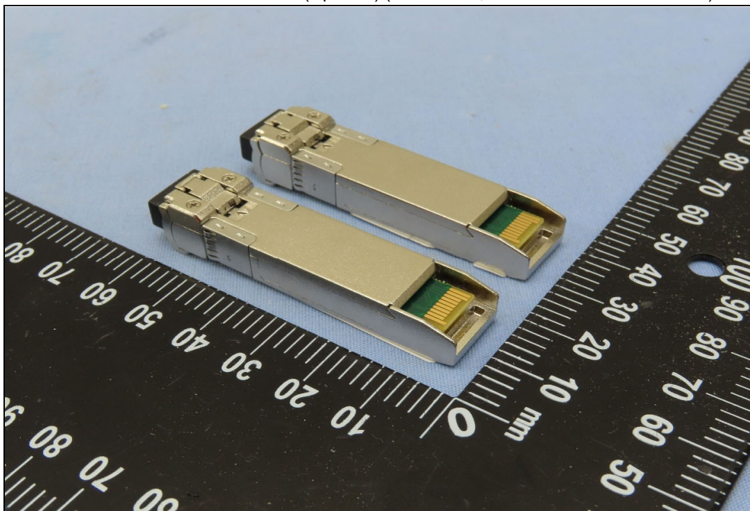
10G SFP+ LR 10km Transceiver (Optional) (Brand: JPC, Model: TNP58260BGIB10-A)
