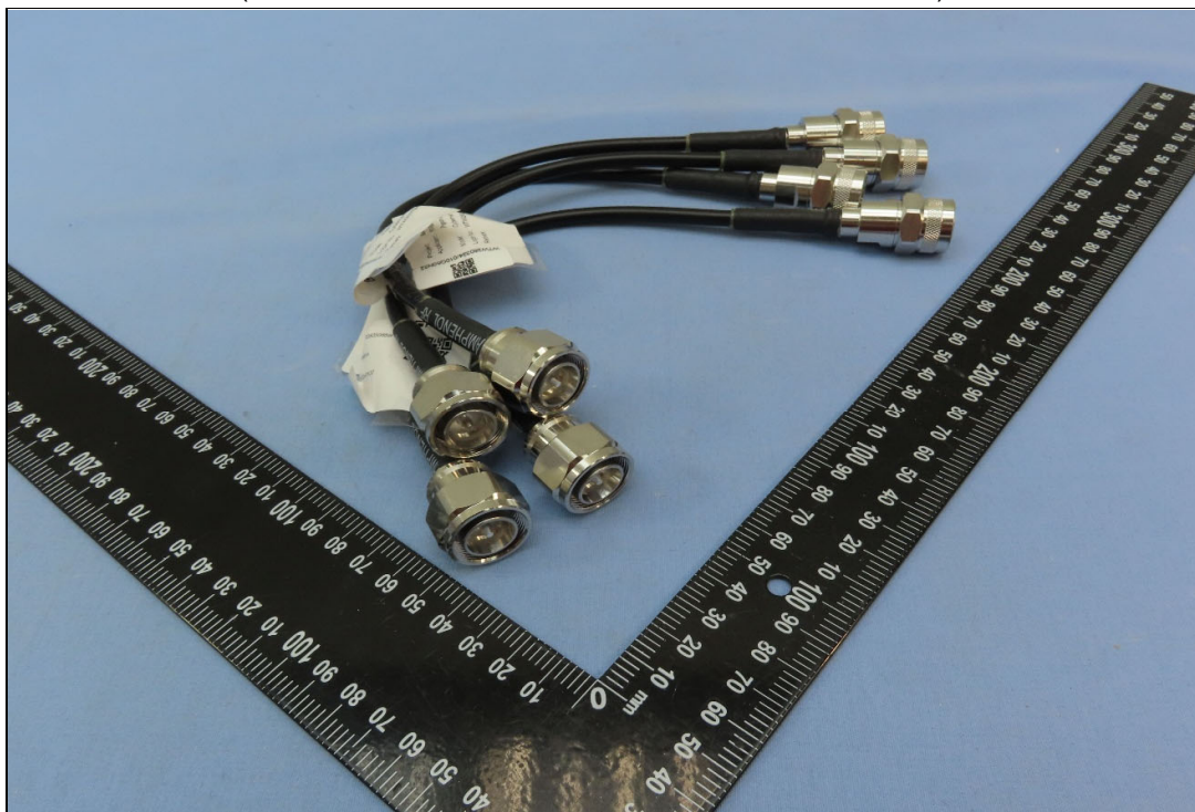
Cable (Brand: AMPHENOL, Model: NM-LMR240-4310M001-25), 185mm
