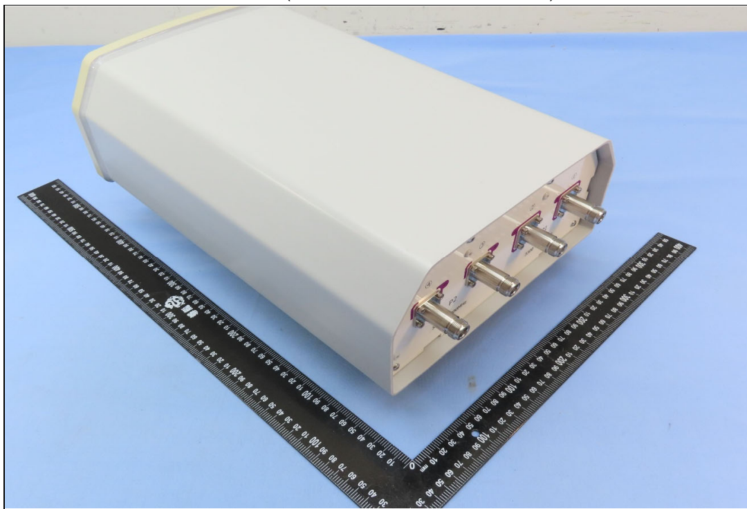
Ant. No. 3 (Brand: WHAYU, Model: 2F04X6B)
