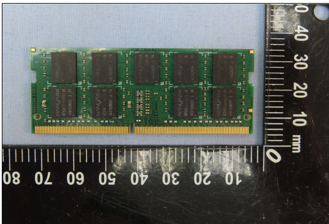
EUT (Brand: PEGATRON, Model: PS2400-4816)
