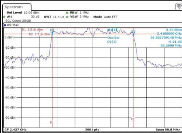
11N2.4G-40M – F5 [Port 1]
