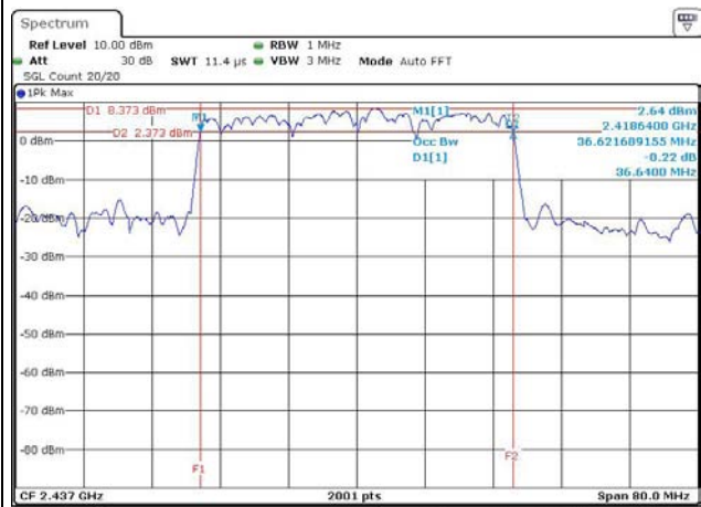
11N2.4G-40M – F2 [Port 1]
