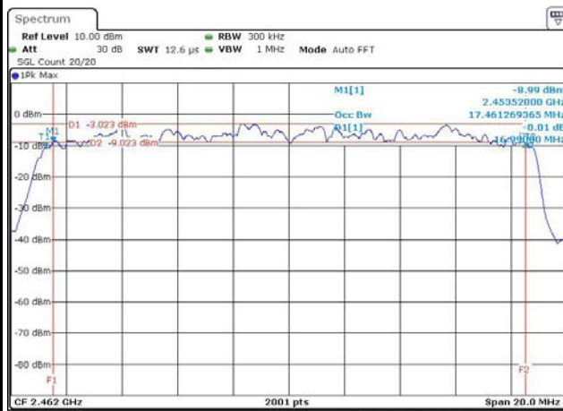
11N2.4G-20M – F3 [Port 1]
