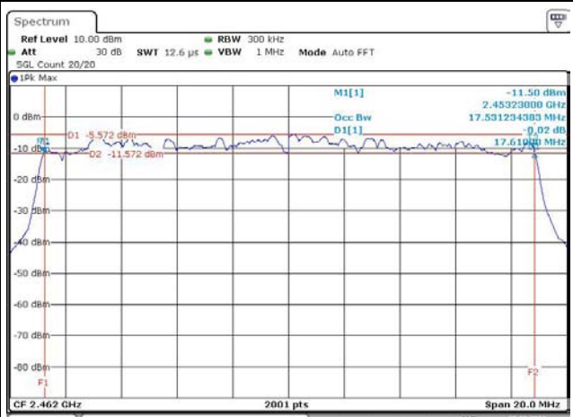
11N2.4G-20M – F3 [Port 2]
