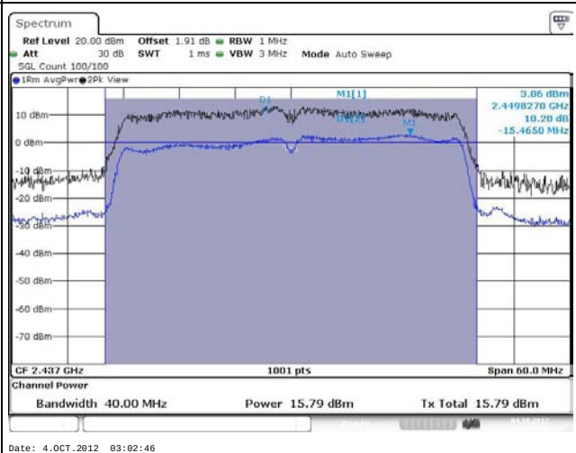
11N2.4G-40M – F2 [Port 1]
