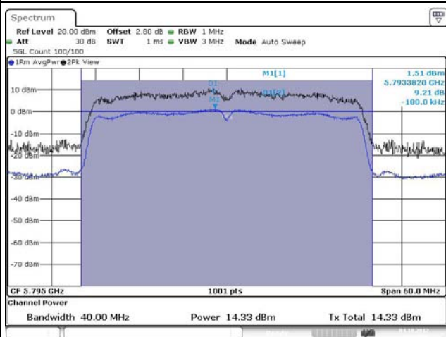
11N5.8G-40M – F5 [Port 2]
