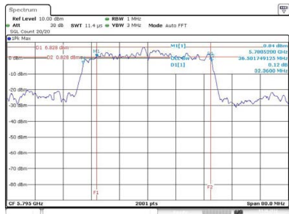
11N5.8G-40M – F5 [Port 2]
