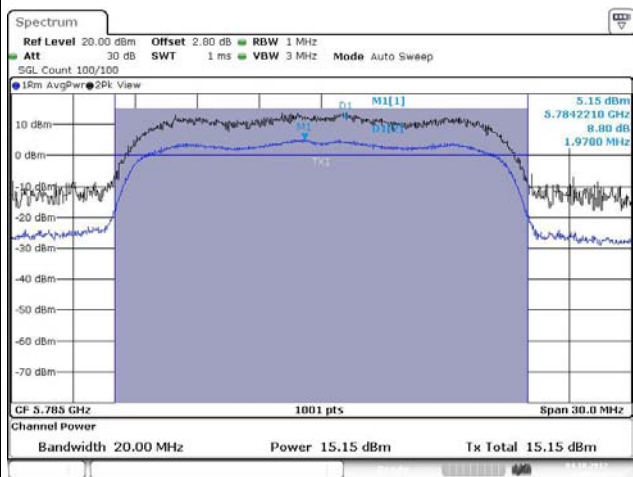
11N5.8G-20M – F2 [Port 2]
