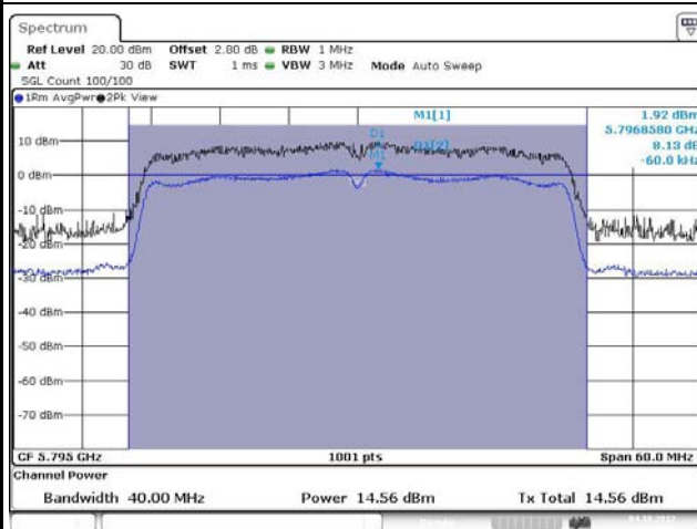
11N5.8G-40M – F5 [Port 1]
