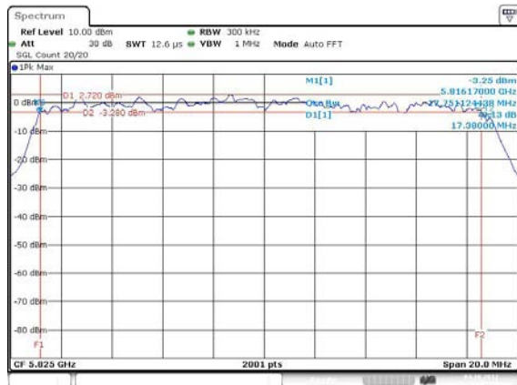
11N5.8G-20M – F3 [Port 1]
