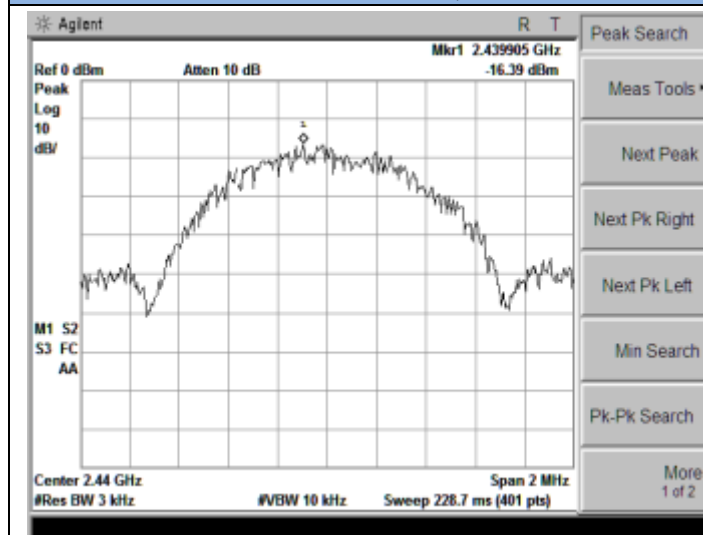
BT V4.0-Middle Channel, 2440MHz
