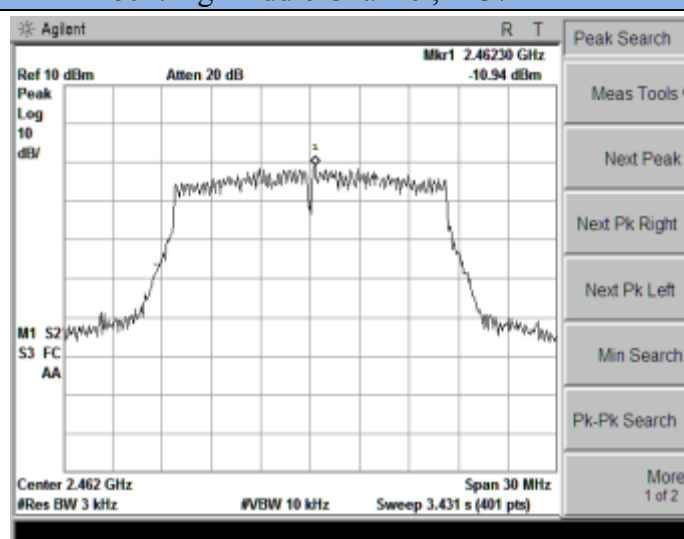
802.11g-High Channel, 2462MHz
