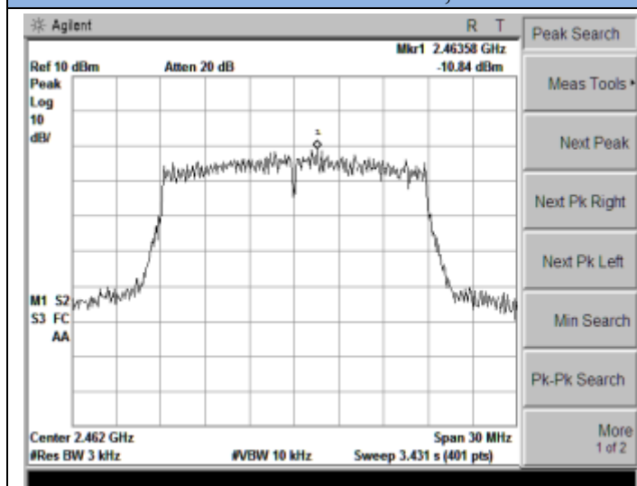
802.11n-HT20-High Channel, 2462MHz
