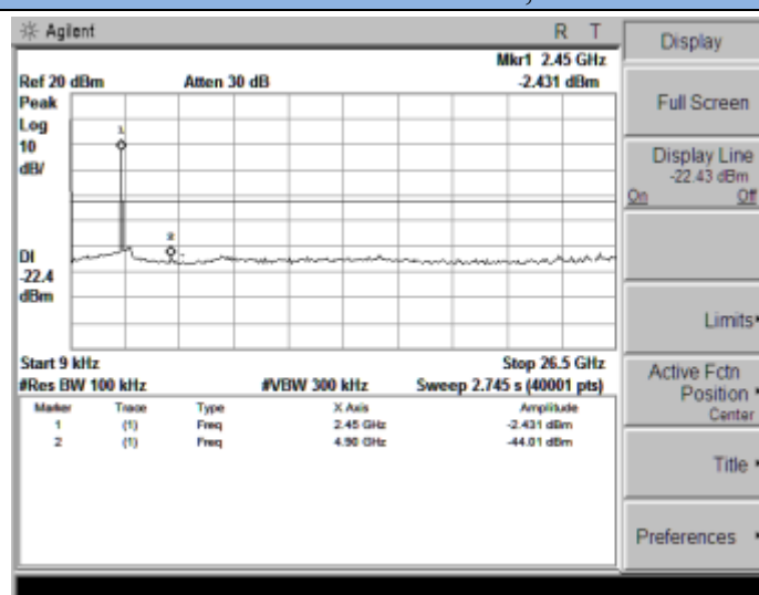
802.11n-HT40-High Channel, 2452MHz
