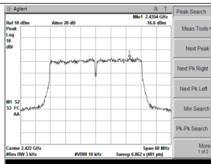
802.11n-HT40-Low Channel, 2422MHz
