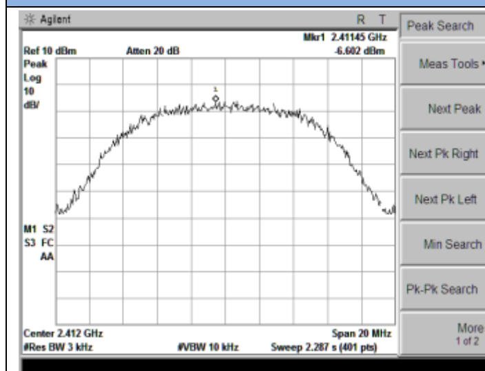
802.11b-Low Channel, 2412MHz
