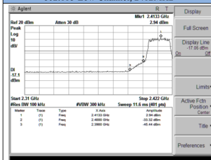
802.11g-Low Channel, 2412MHz
