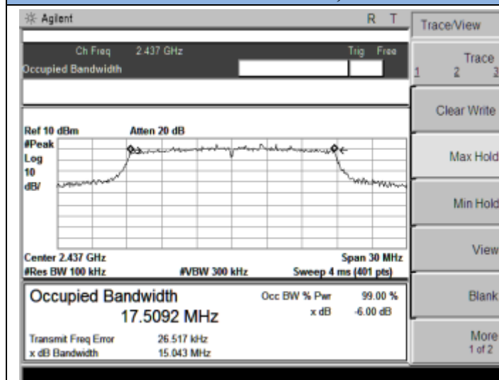
802.11n-HT20-Middle Channel, 2437MHz
