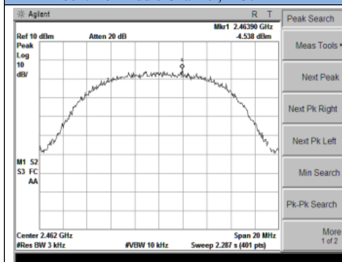
802.11b-High Channel, 2462MHz
