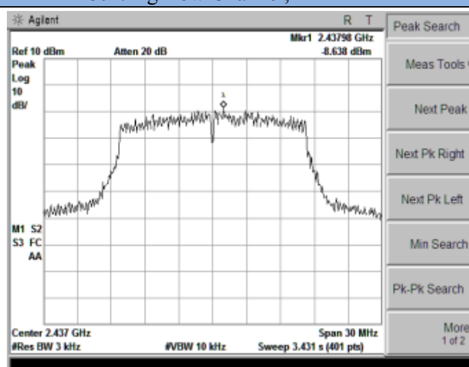
802.11g-Middle Channel, 2437MHz
