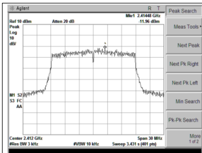
802.11n-HT20-Low Channel, 2412MHz
