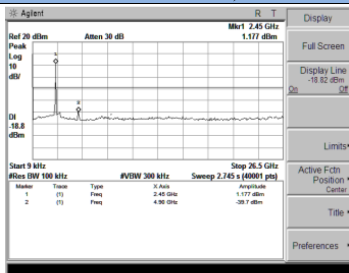
802.11n-HT40-Middle Channel, 2437MHz
