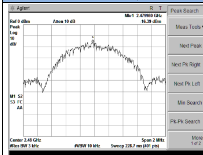
BT V4.0-High Channel, 2480MHz
