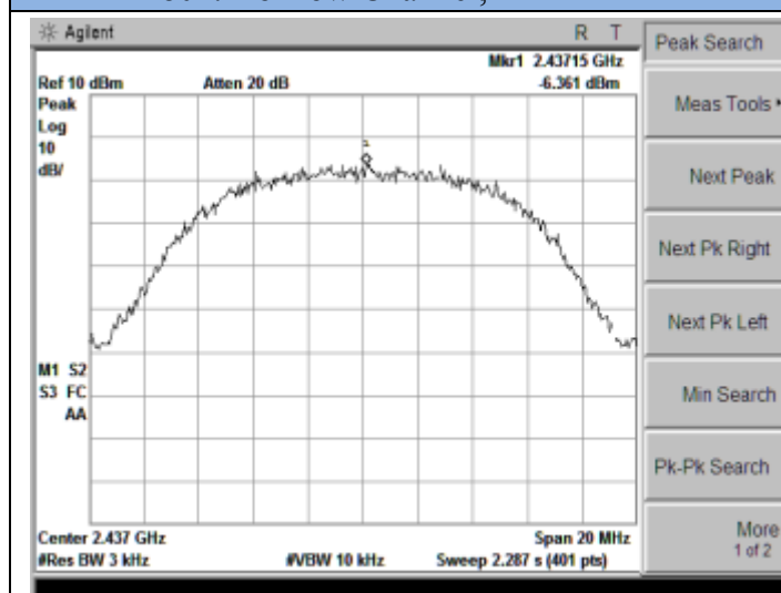
802.11b-Middle Channel, 2437MHz
