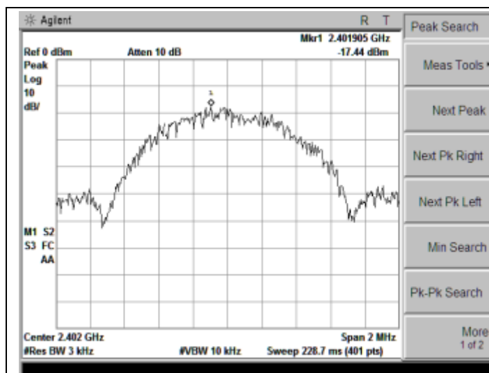
BT V4.0-Low Channel, 2402MHz
