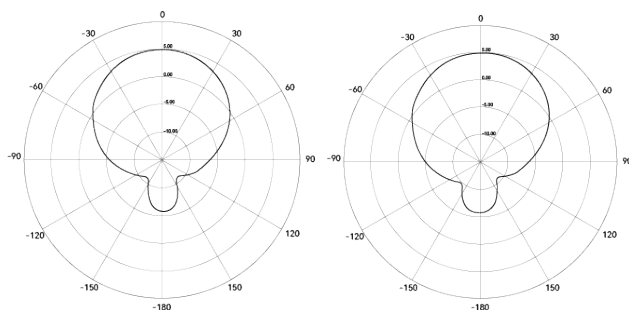
Antenna E-plane orientation diagram
