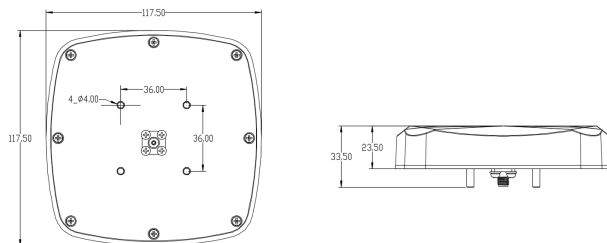
Appearance dimension drawing of XC-AF802-BEN-A type antenna
