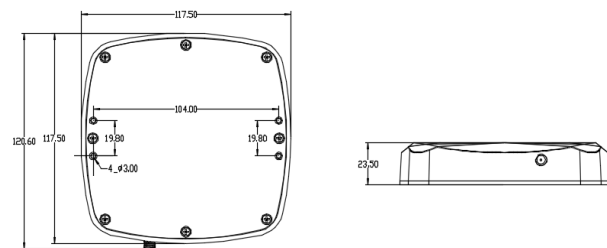
Appearance dimension drawing of XC-AF802-BEN-B type antenna
