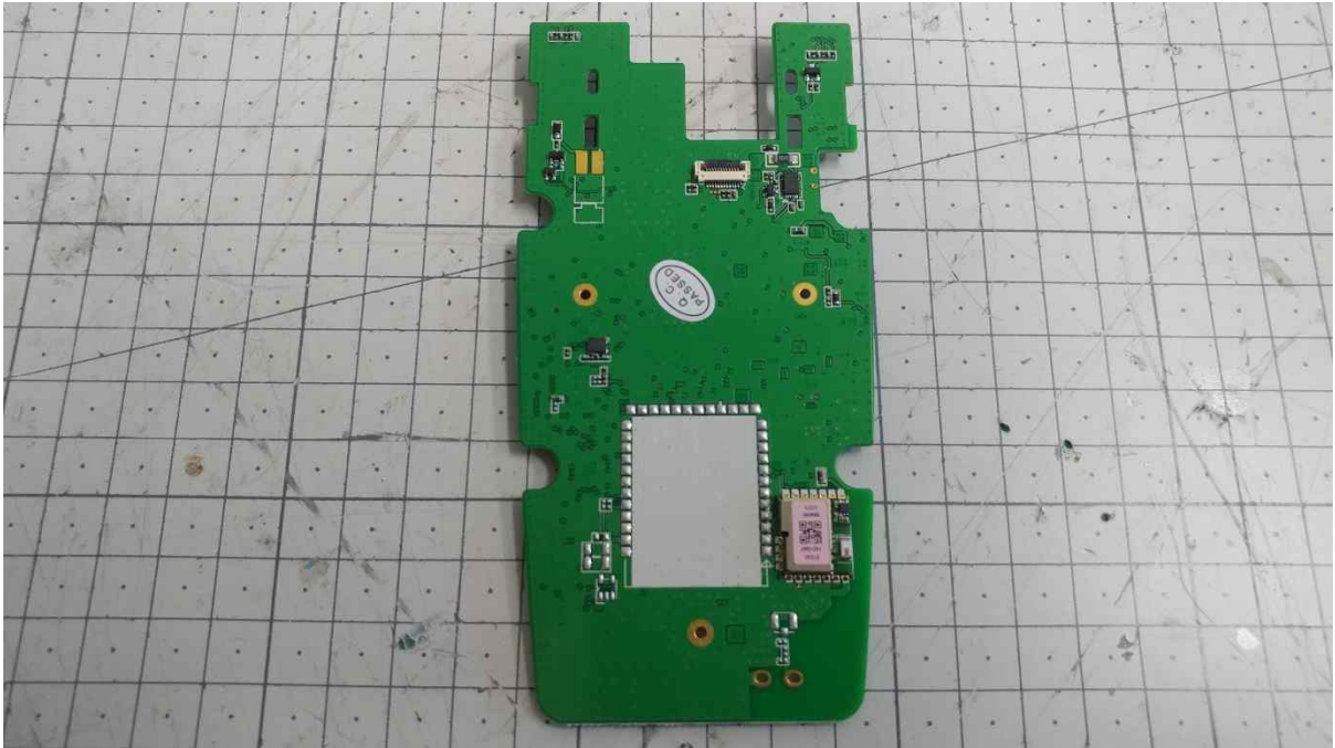
Main Board Rear
