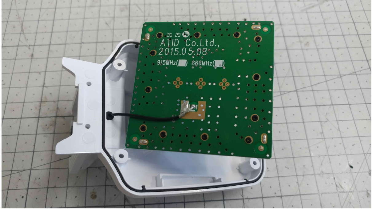
RFID Antenna Board Rear
