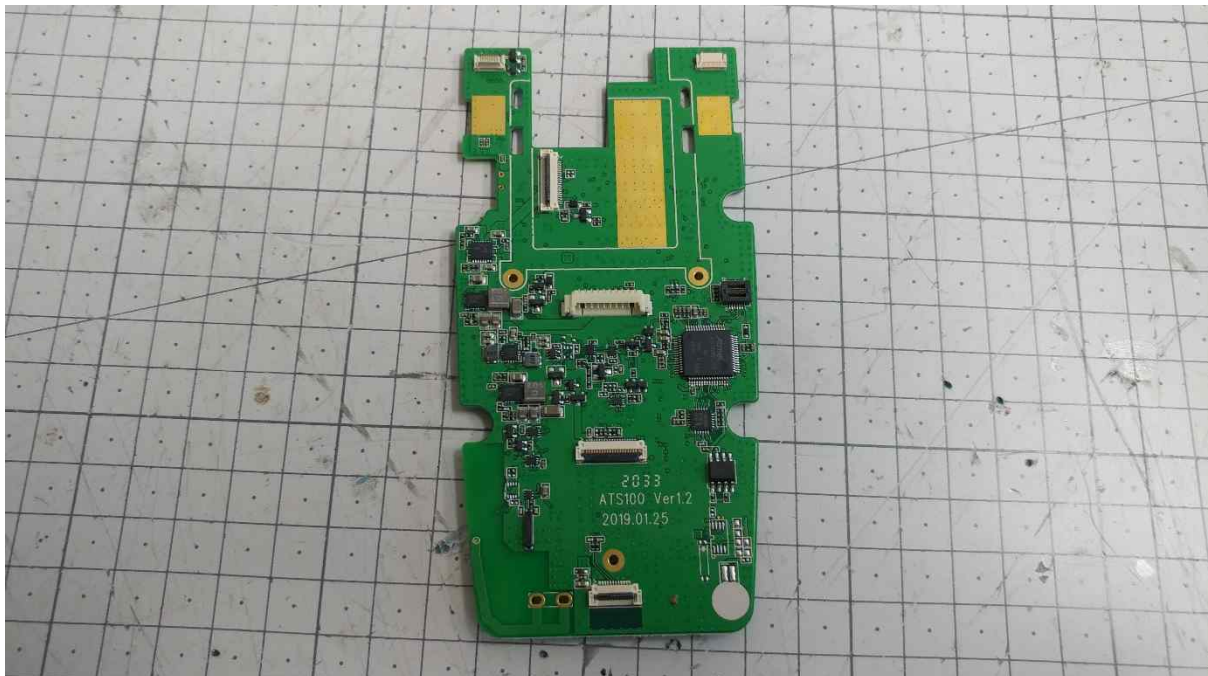
Main Board Front
