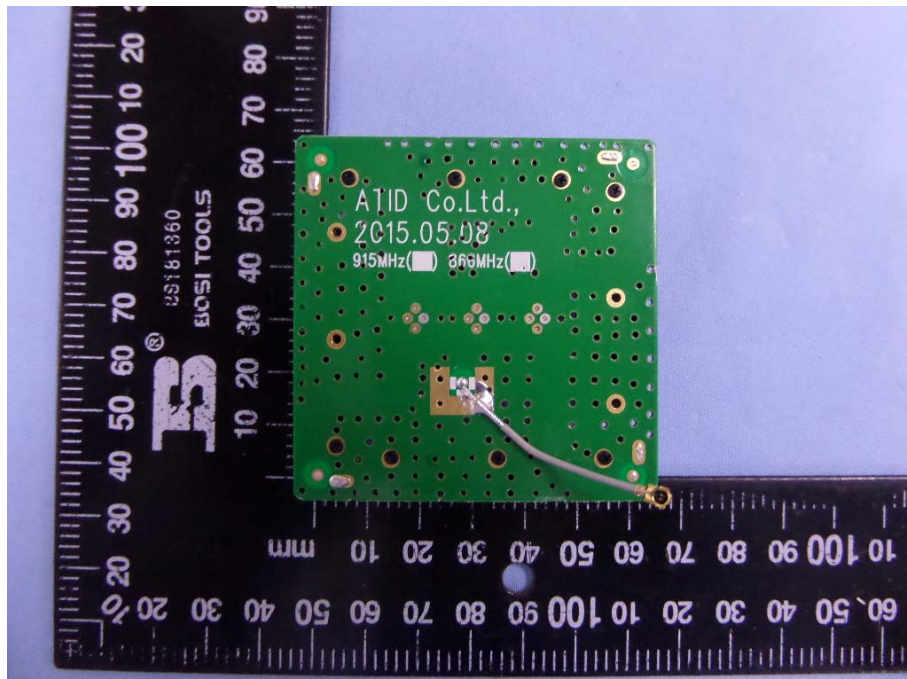
Solder Board-Component View 12 (UHF Antenna)
