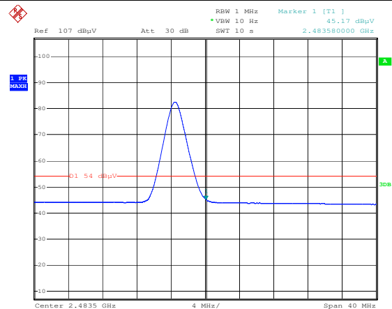
Band Edge, Right Side (Peak) Note: F1 is frequency 2483.5MHz
