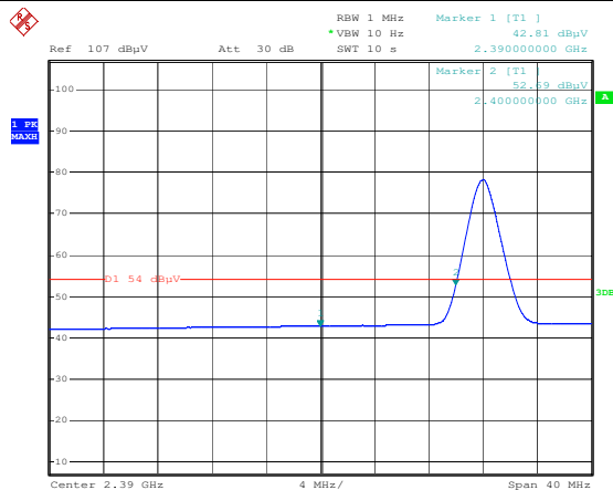
Band Edge, Left Side (Peak) Note: F1 is frequency 2390MHz; F2 is frequency 2400MHz
