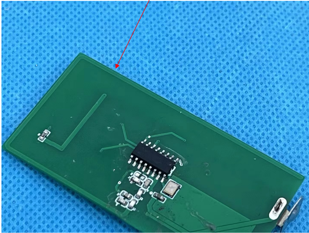
SRD Antenna
