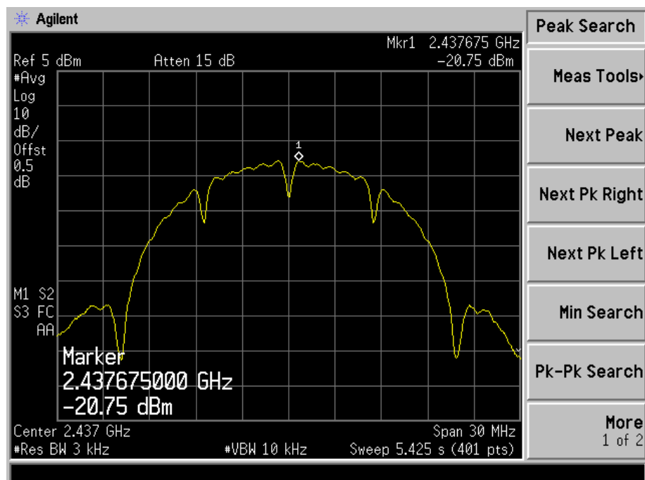
802.11b-Middle Channel
