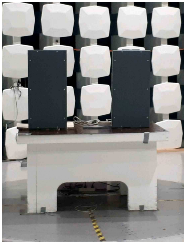
Radiated Emissions Below 30 MHz – front view
