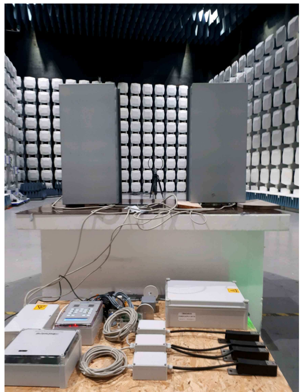
Radiated Emissions Below 30 MHz – back view
