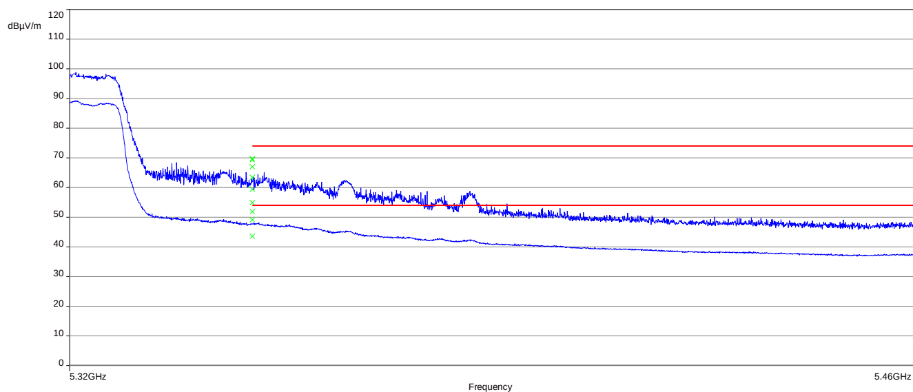
Plot 23: upper band edge; U-NII-2A; middle channel; ac80-mode
