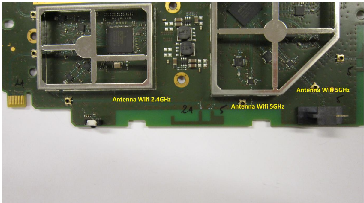
Antenna Wifi (Front)
