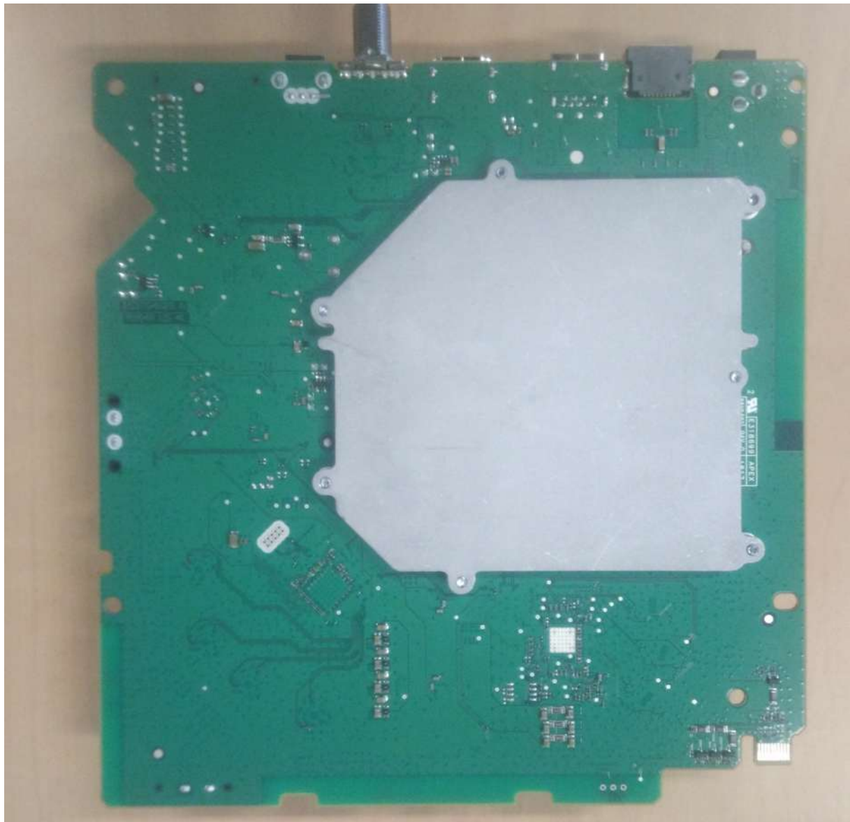
Main Board face 2 with Shielding
