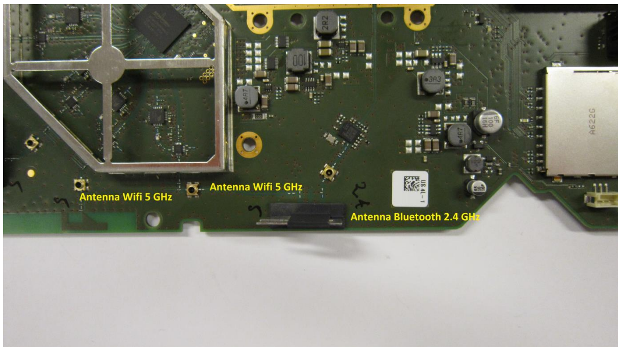
Antenna Wifi-BT 2.4GHz (Right)
