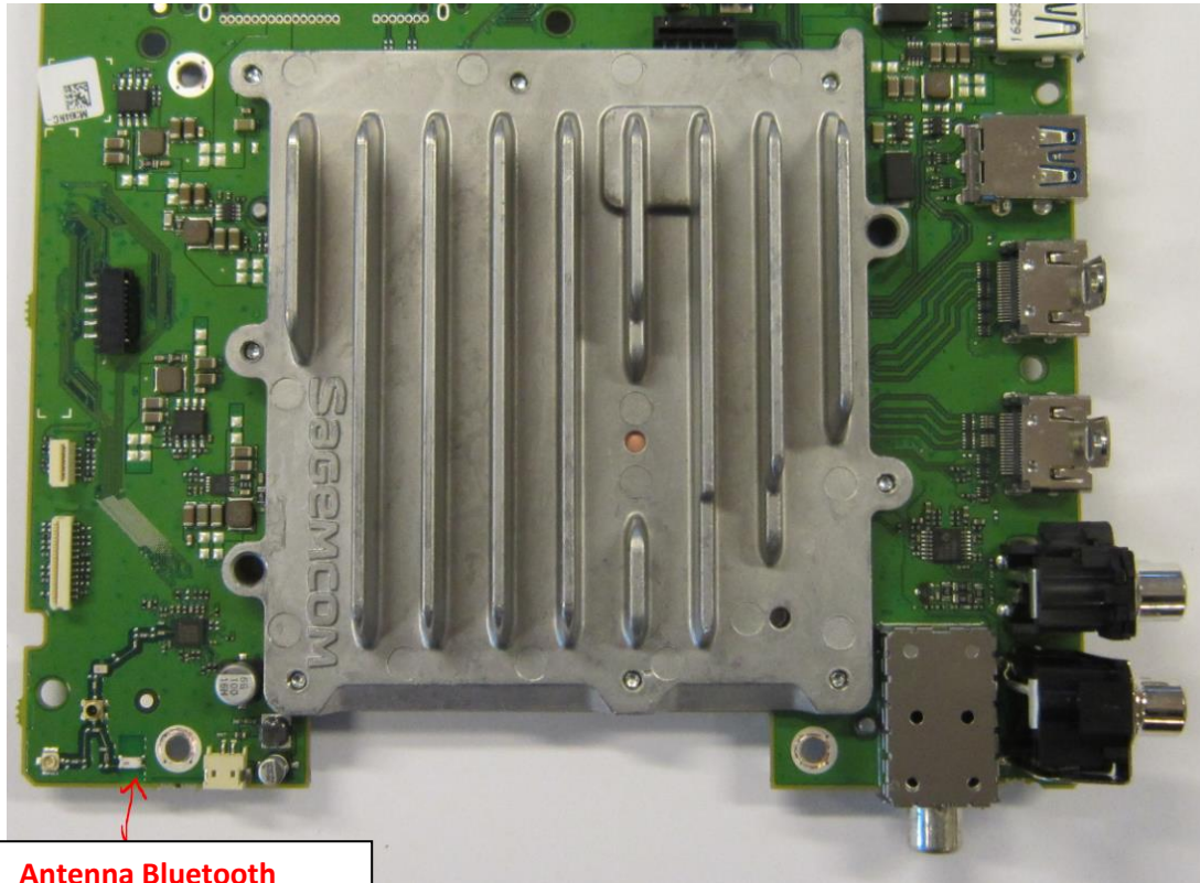
Antenna Bluetooth
