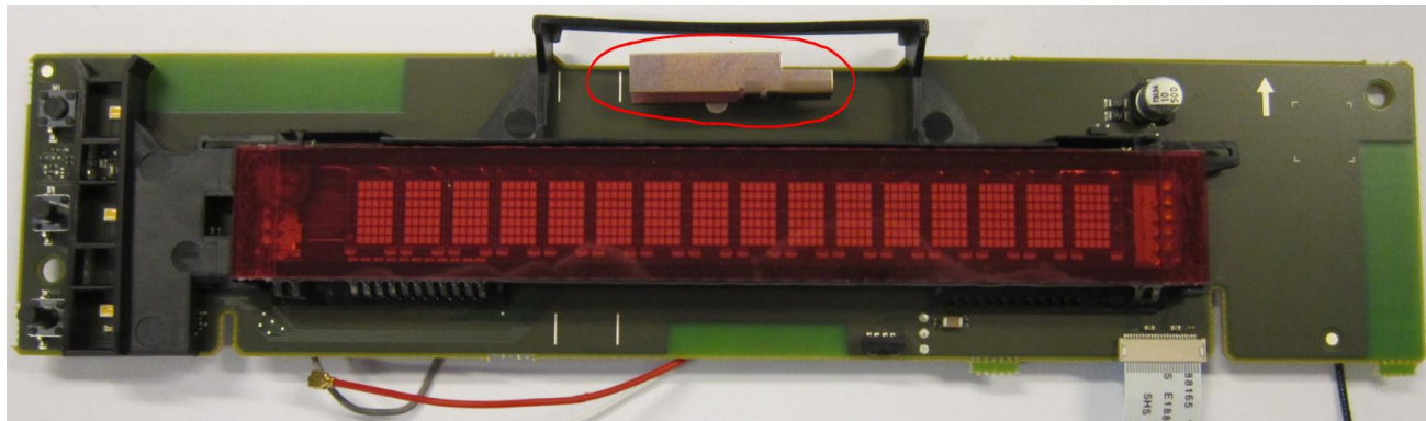
Antenna Wi-Fi Dual Band
