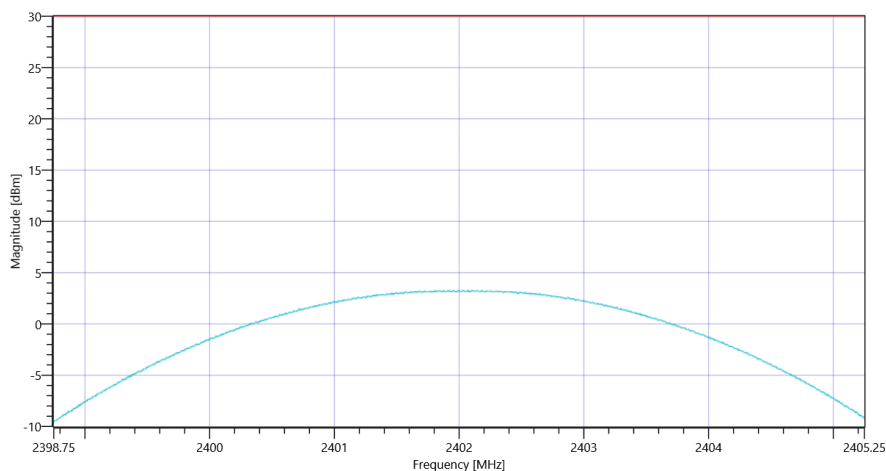
FCC 15.247 # Maximum peak conducted output power FHSS ~ BT Classic EDR Pi-4QPSK
