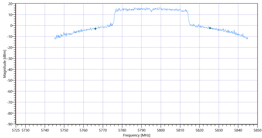
FCC 15.407, ISSED RSS247 # Bandwidths 99PCT and 26dB ~ WLAN5Gx ax-HE40 U-NII-3
