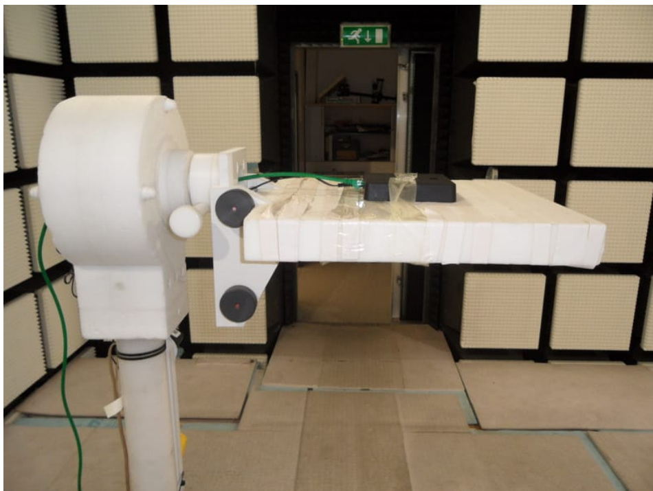
Photo 6: RSE >1 GHz
