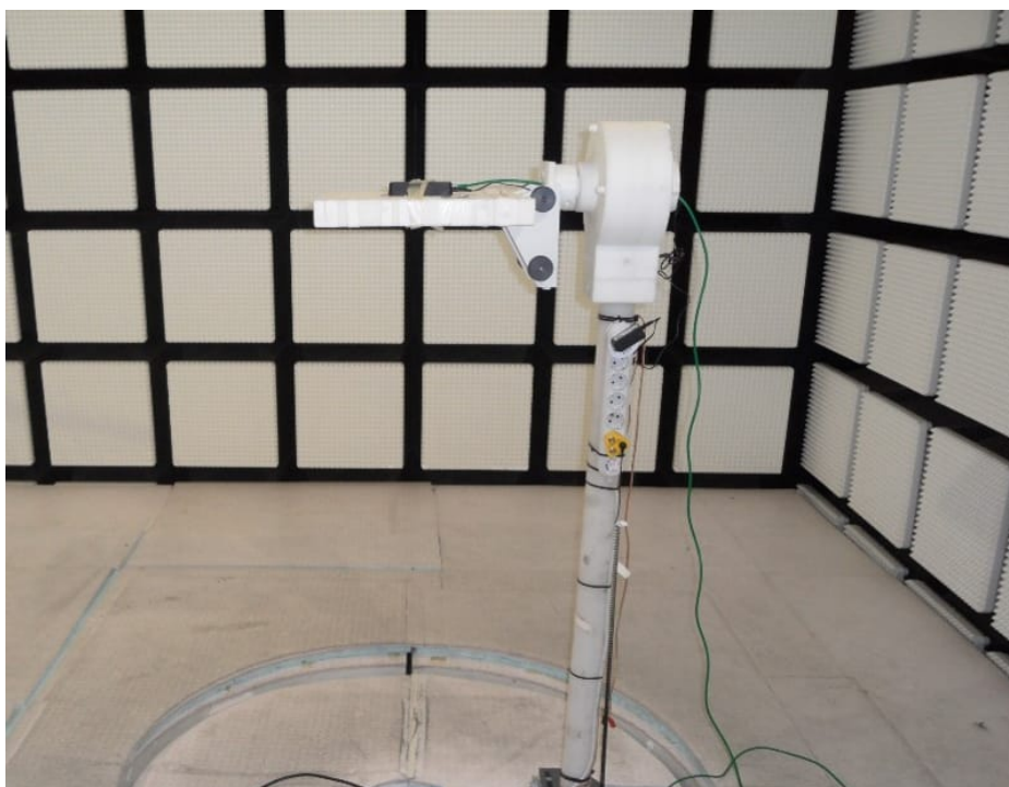
Photo 4: RSE >1 GHz
