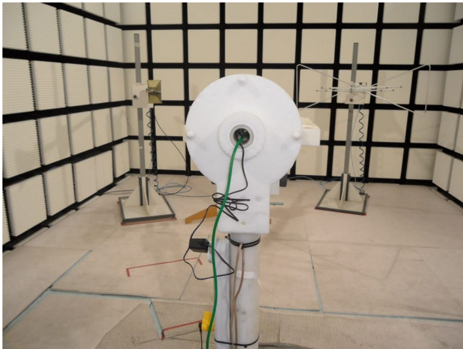
Photo 5: RSE >1 GHz
