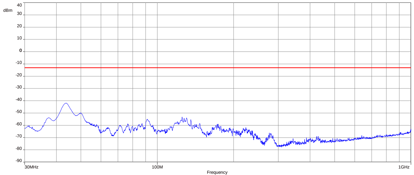
Plot 11: BPSK - Middle channel (30 MHz – 1 GHz)
