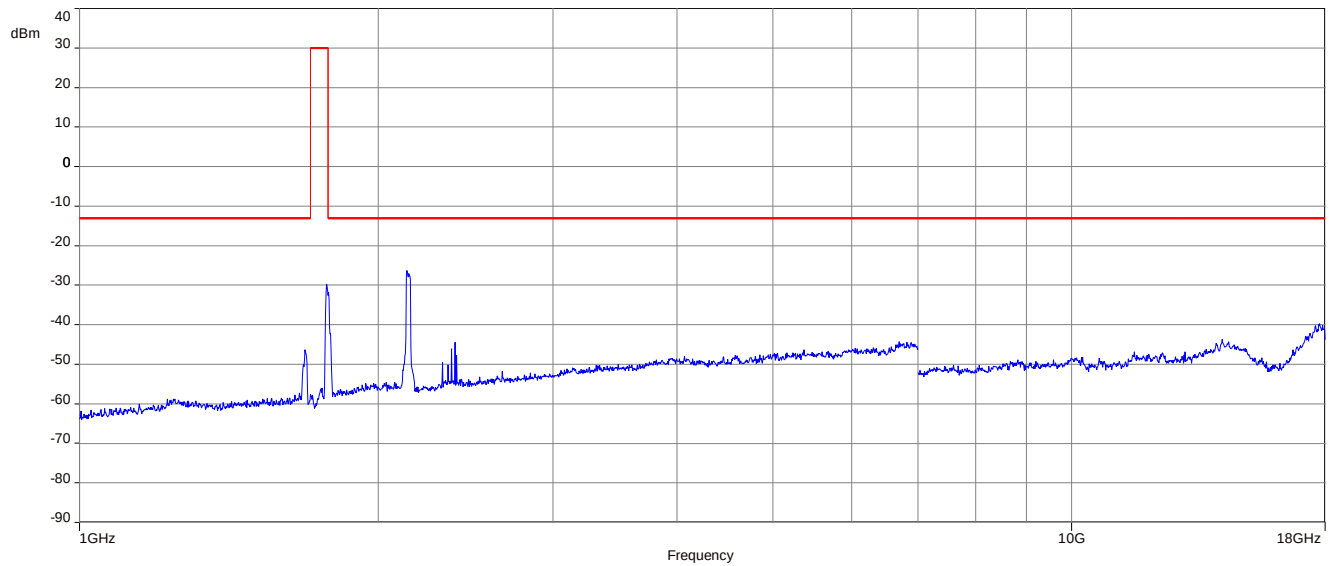
Plot 9: 64-QAM - Middle channel (1 GHz – 18 GHz)
