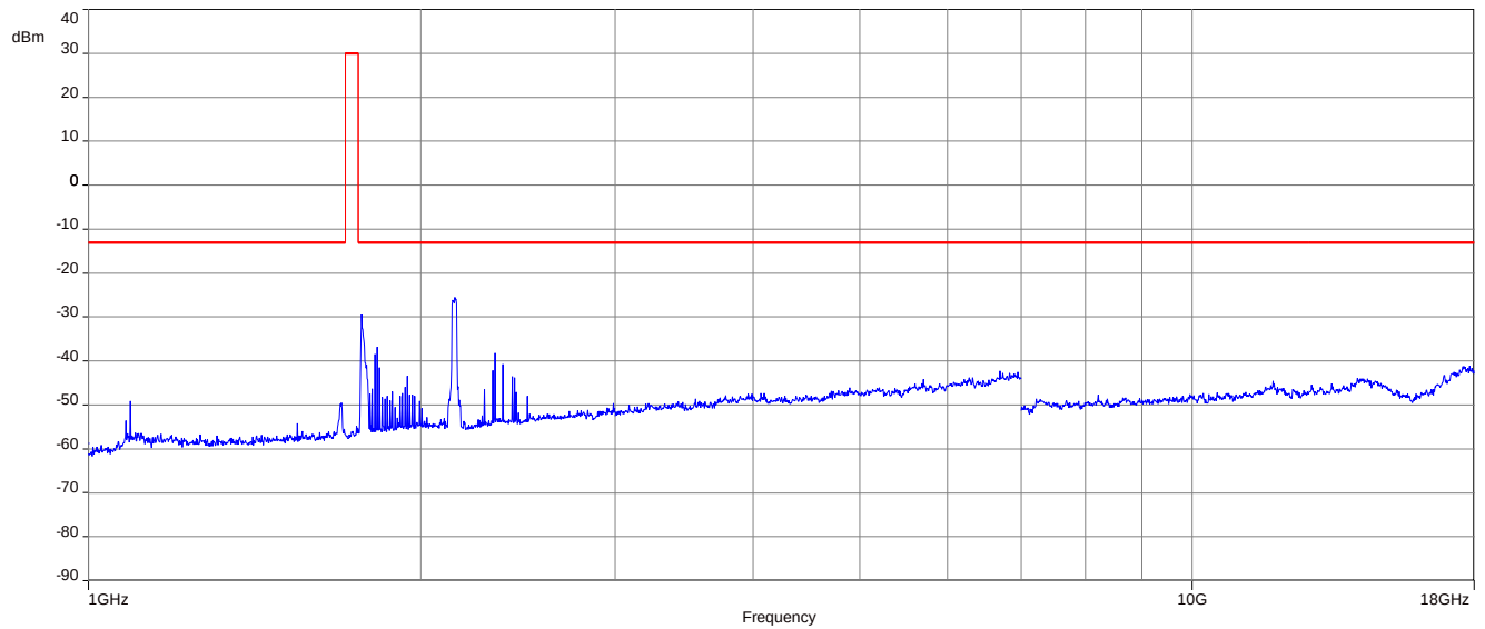
Plot 15: 256-QAM - Middle channel (1 GHz – 18 GHz)
