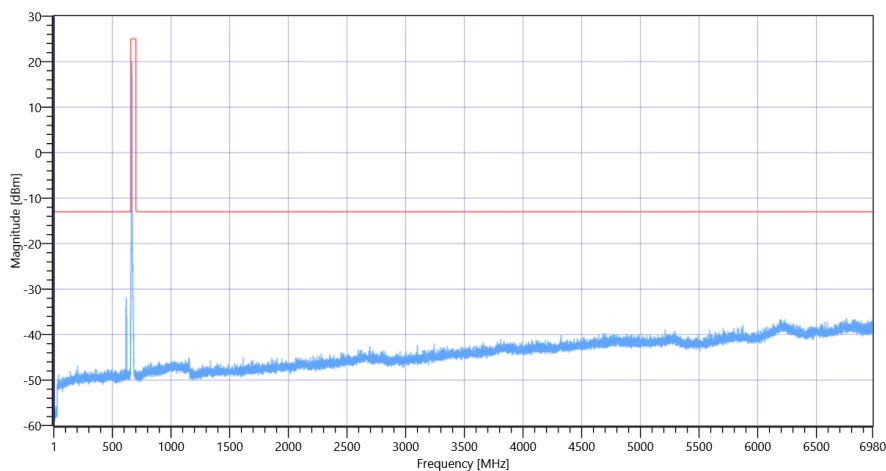
FCC, ISSED # TX Emissions conducted ~ NR Band_71 Ant-1 SCS-15 665.5 MHz
