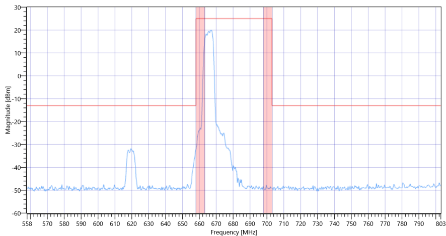
FCC, ISSED # TX Emissions conducted ~ NR Band_71 Ant-1 SCS-15 665.5
