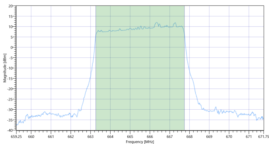
FCC, ISED # Bandwidth 99PCT and 26dB ~ NR Band_71 Ant-1 SCS-15 26dB
