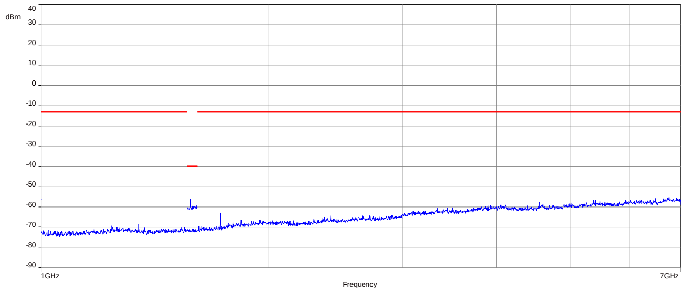
Plot 3: BPSK - Middle channel (1 GHz – 7 GHz)
