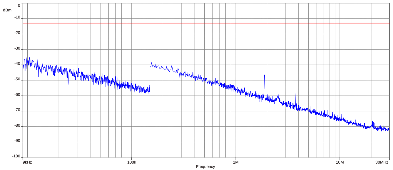
Plot 4: QPSK - Middle channel (9 kHz - 30 MHz)
