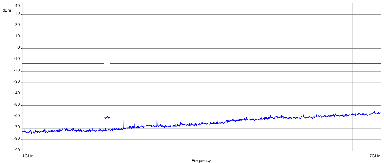
Plot 6: QPSK - Middle channel (1 GHz – 7 GHz)
