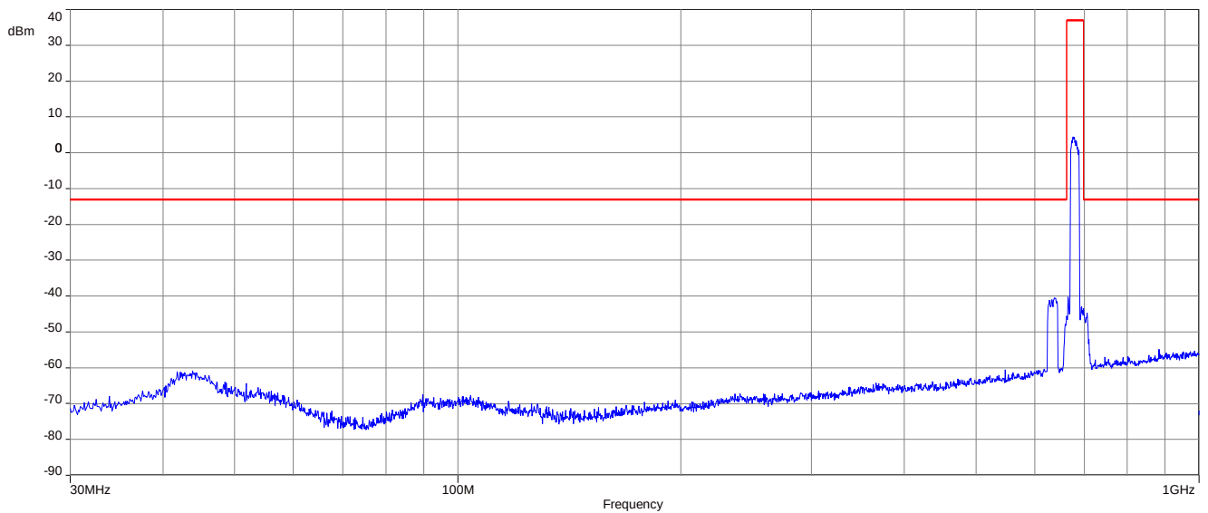
Plot 2: BPSK - Middle channel (30 MHz – 1 GHz)
