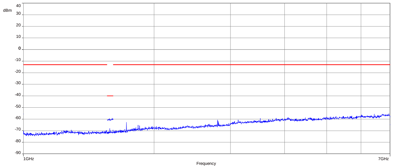
Plot 6: 64-QAM - Middle channel (1 GHz – 7 GHz)
