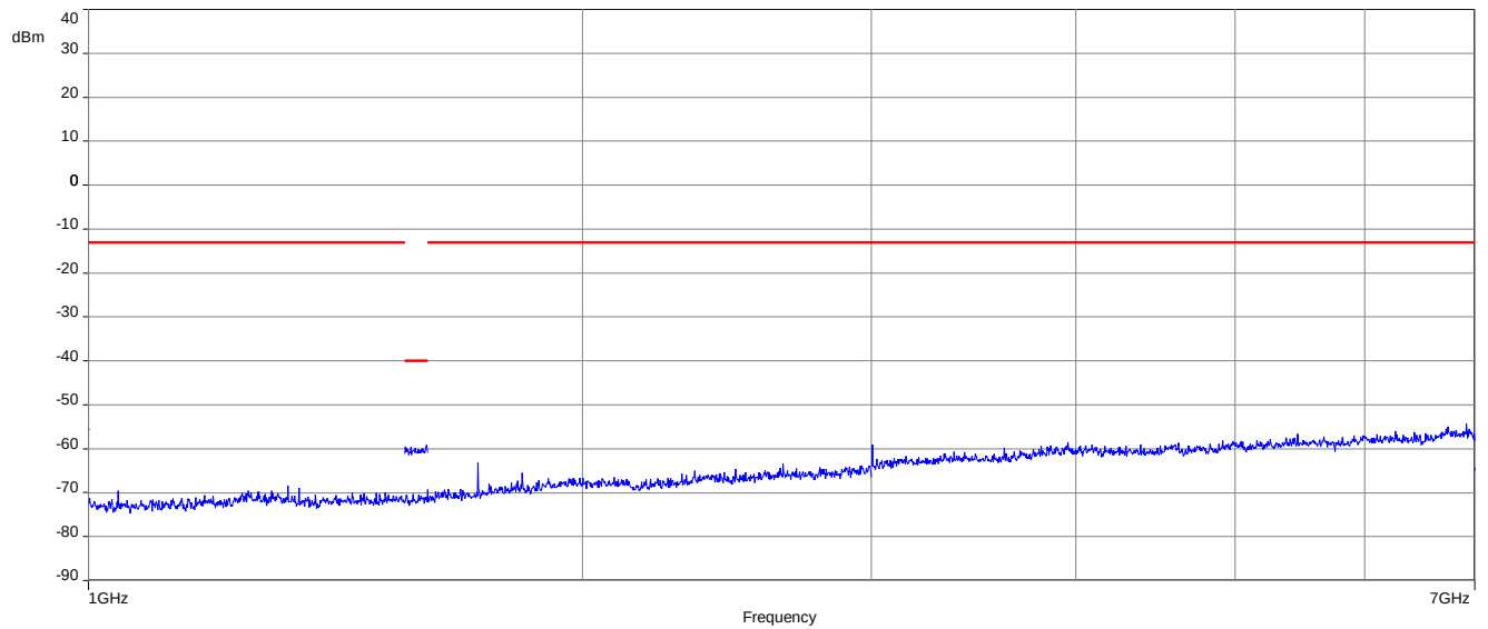
Plot 3: 16-QAM - Middle channel (1 GHz – 7 GHz)
