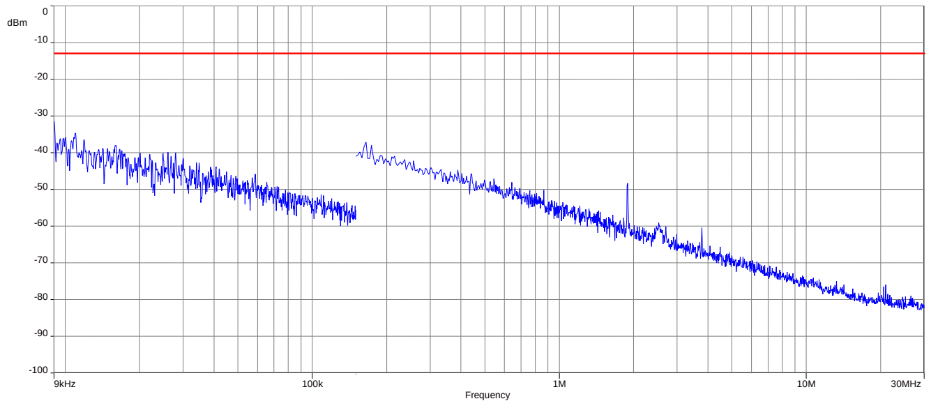
Plot 1: 16-QAM - Middle channel (9 kHz - 30 MHz)
