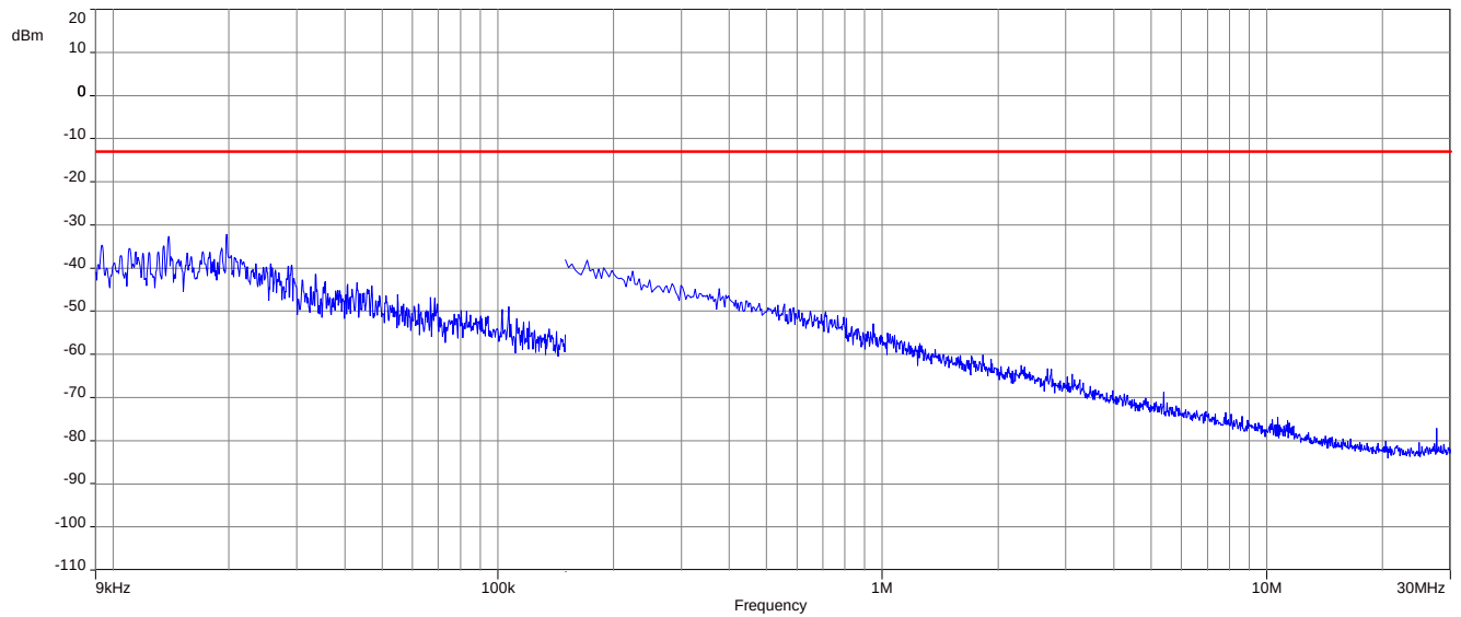
Plot 7: 256-QAM - Middle channel (9 kHz - 30 MHz)
