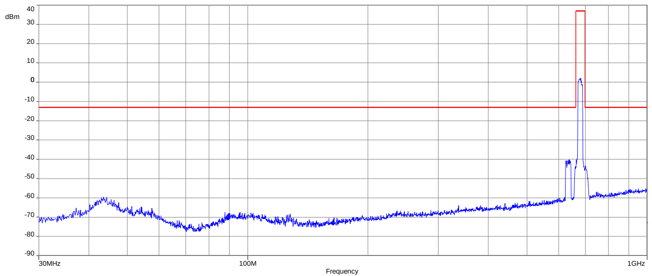
Plot 2: 16-QAM - Middle channel (30 MHz – 1 GHz)
