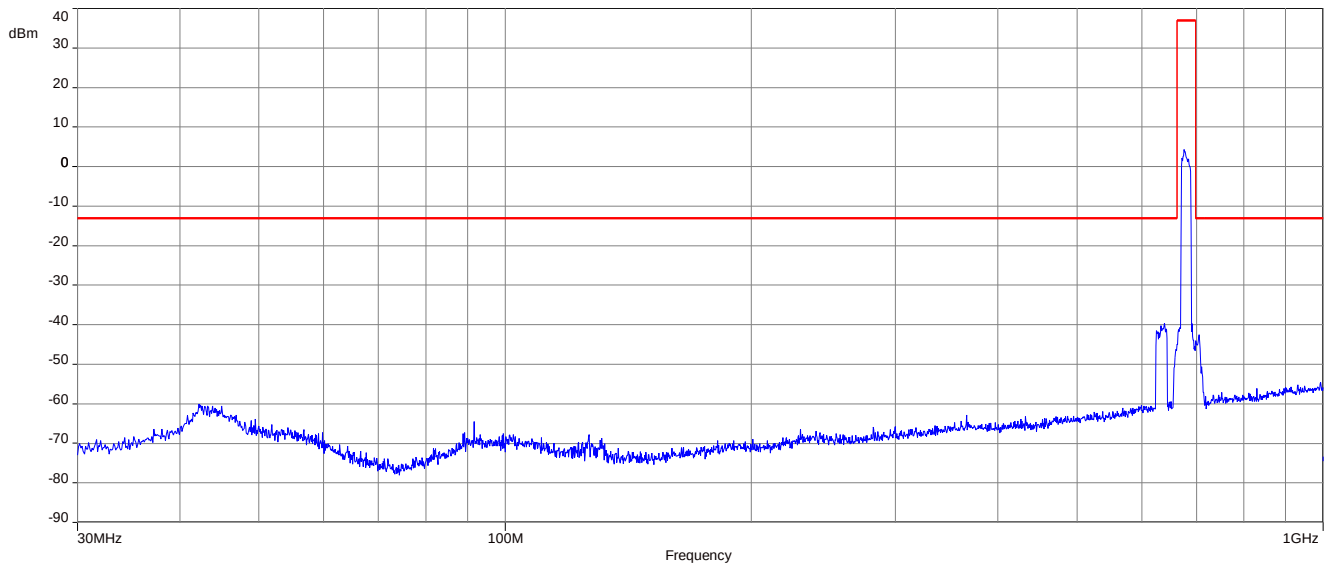
Plot 5: QPSK - Middle channel (30 MHz – 1 GHz)
