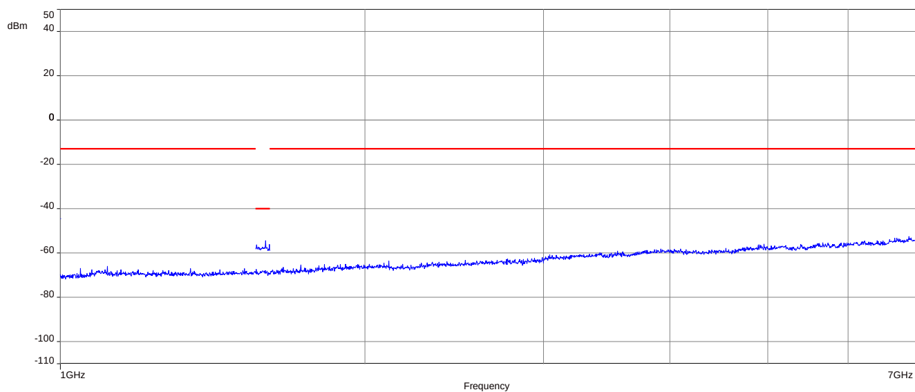
Plot 9: 256-QAM - Middle channel (1 GHz – 7 GHz)
