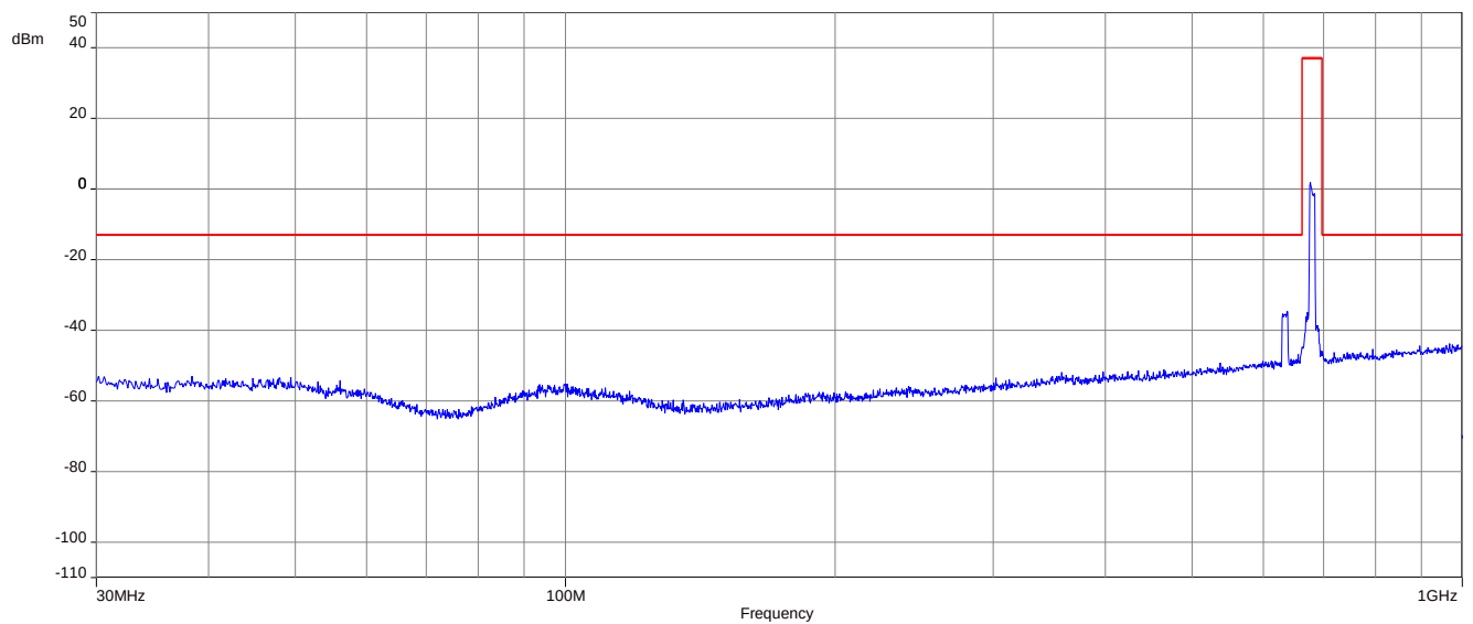
Plot 8: 256-QAM - Middle channel (30 MHz – 1 GHz)
