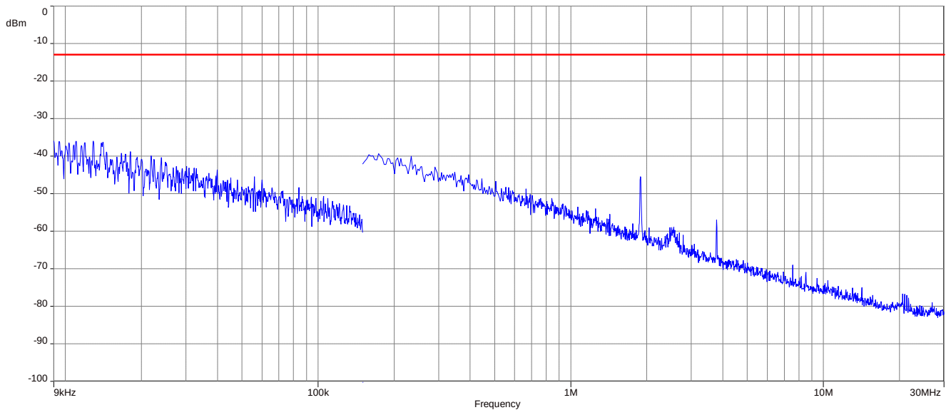
Plot 1: BPSK - Middle channel (9 kHz - 30 MHz)
