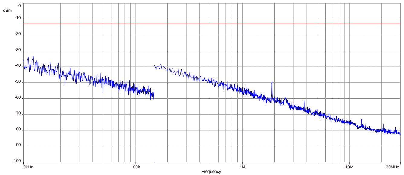
Plot 4: 64-QAM - Middle channel (9 kHz - 30 MHz)
