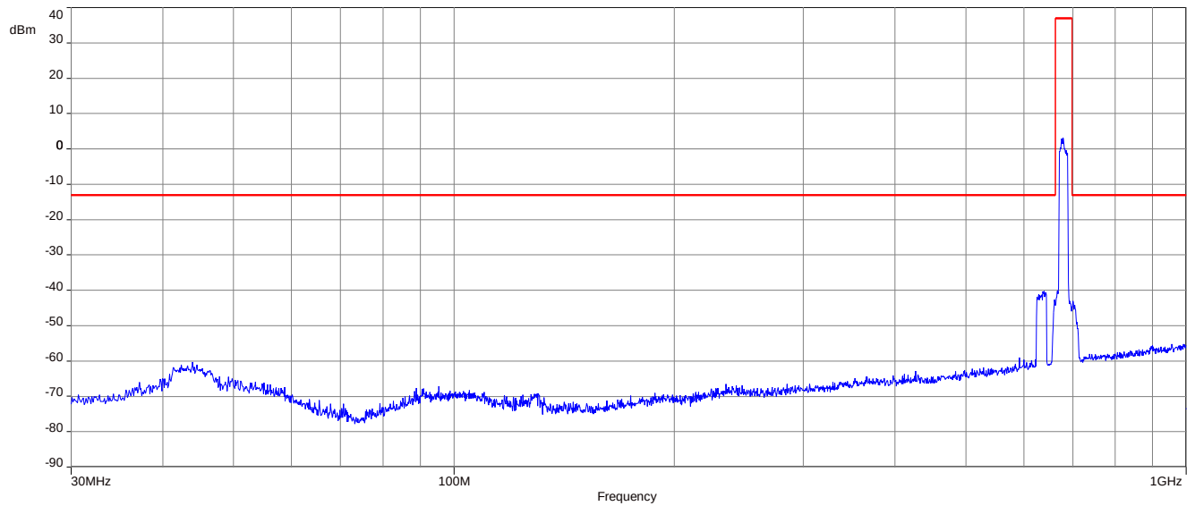
Plot 5: 64-QAM - Middle channel (30 MHz – 1 GHz)
