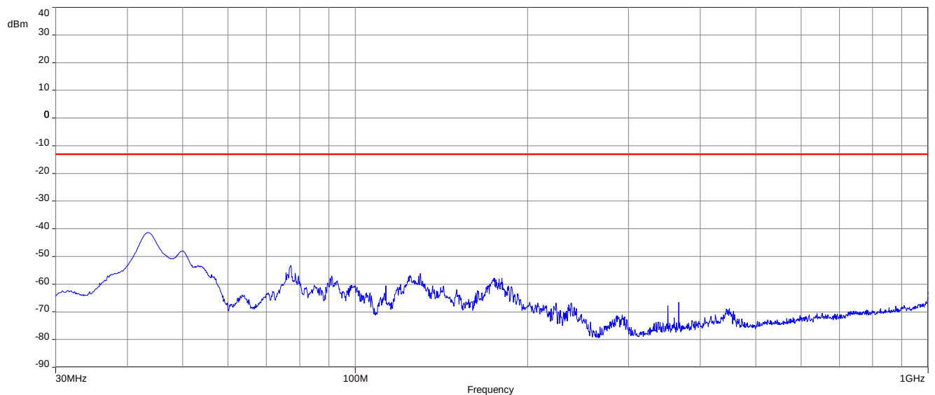
Plot 2: 16-QAM - lowest channel (30 MHz – 1 GHz)
