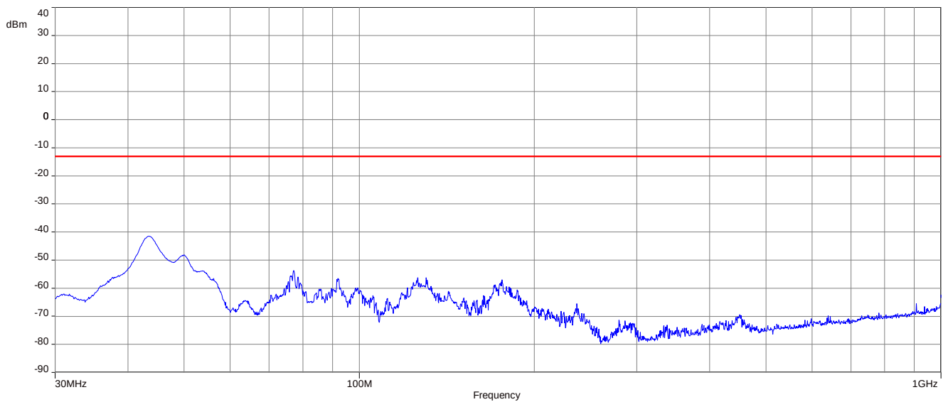
Plot 10: 16-QAM - mid channel (30 MHz – 1 GHz)
