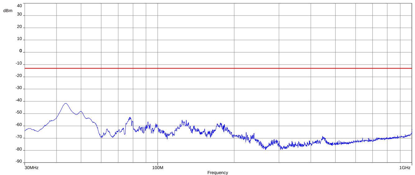
Plot 2: BPSK - lowest channel (30 MHz – 1 GHz)
