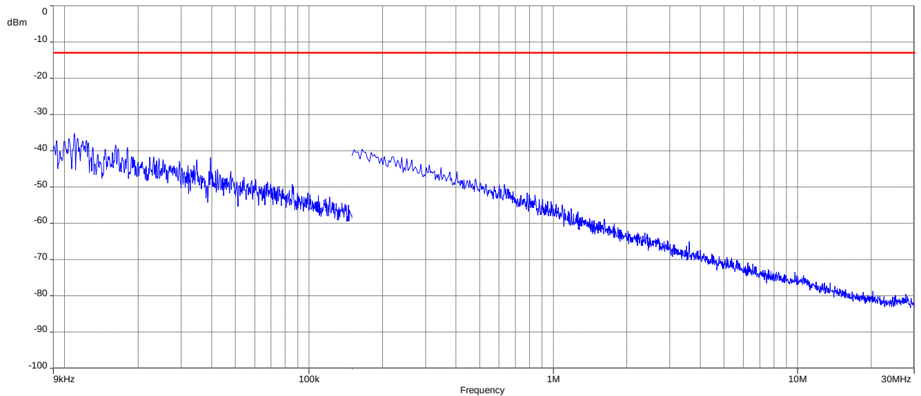
Plot 1: BPSK - mid channel (9 kHz - 30 MHz)
