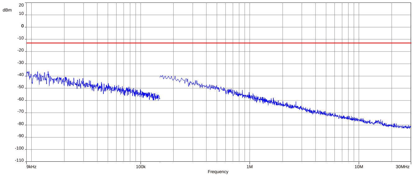
Plot 17: 256-QAM - mid channel (9 kHz - 30 MHz)
