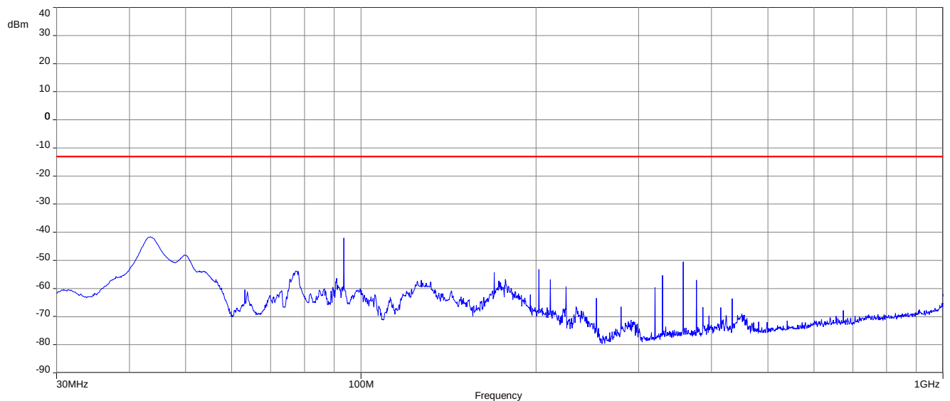
Plot 14: 64-QAM - mid channel (30 MHz – 1 GHz)
