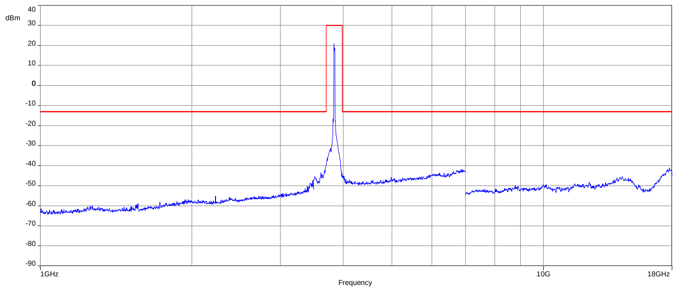
Plot 3: BPSK - lowest channel (1 GHz – 18 GHz)
