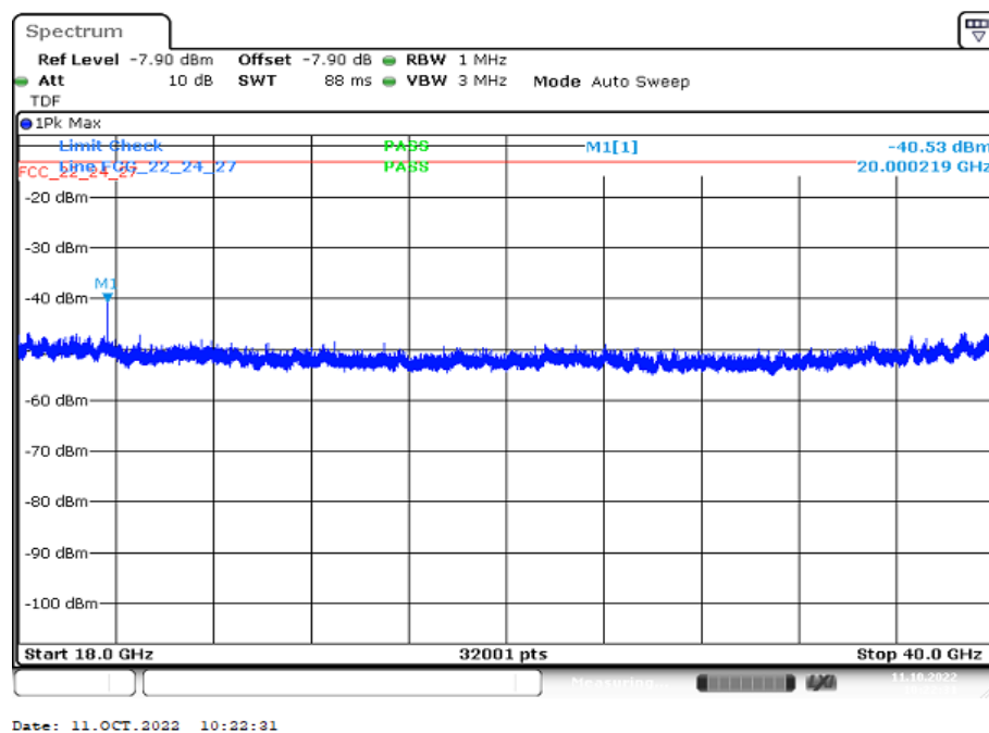
Plot 4: BPSK - mid channel (18 GHz – 40 GHz)
