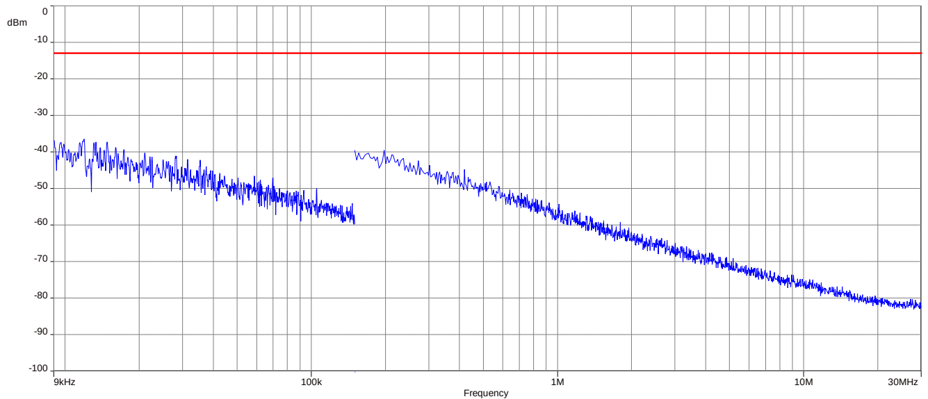
Plot 1: BPSK - lowest channel (9 kHz - 30 MHz)
