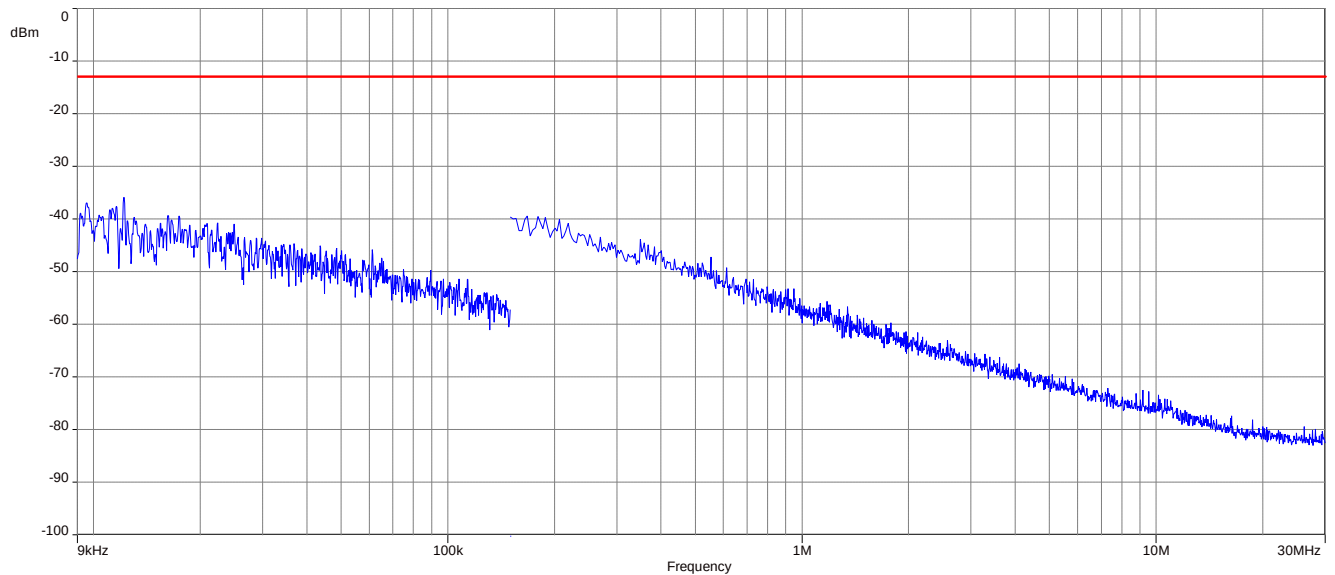
Plot 1: 16-QAM - lowest channel (9 kHz - 30 MHz)
