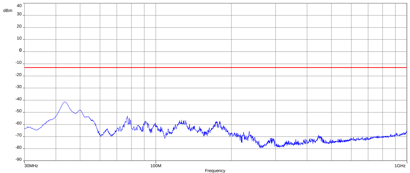
Plot 2: BPSK - mid channel (30 MHz – 1 GHz)
