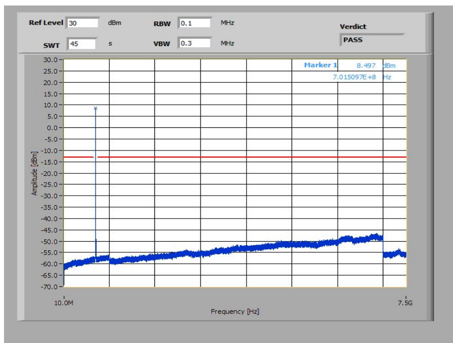
Plot 4: 3 MHz – QPSK - Lowest Channel (10 MHz – 7.5 GHz)
