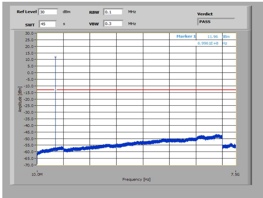
Plot 1: 1.4 MHz – QPSK - Lowest Channel (10 MHz – 7.5 GHz)
