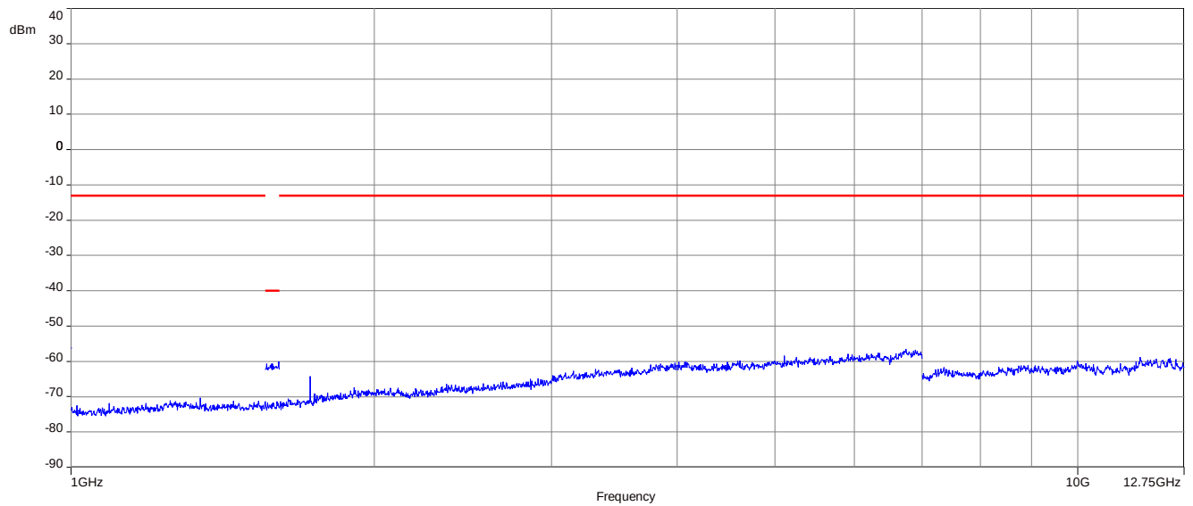
Plot 3: QPSK - Middle channel (1 GHz – 12.75 GHz)
