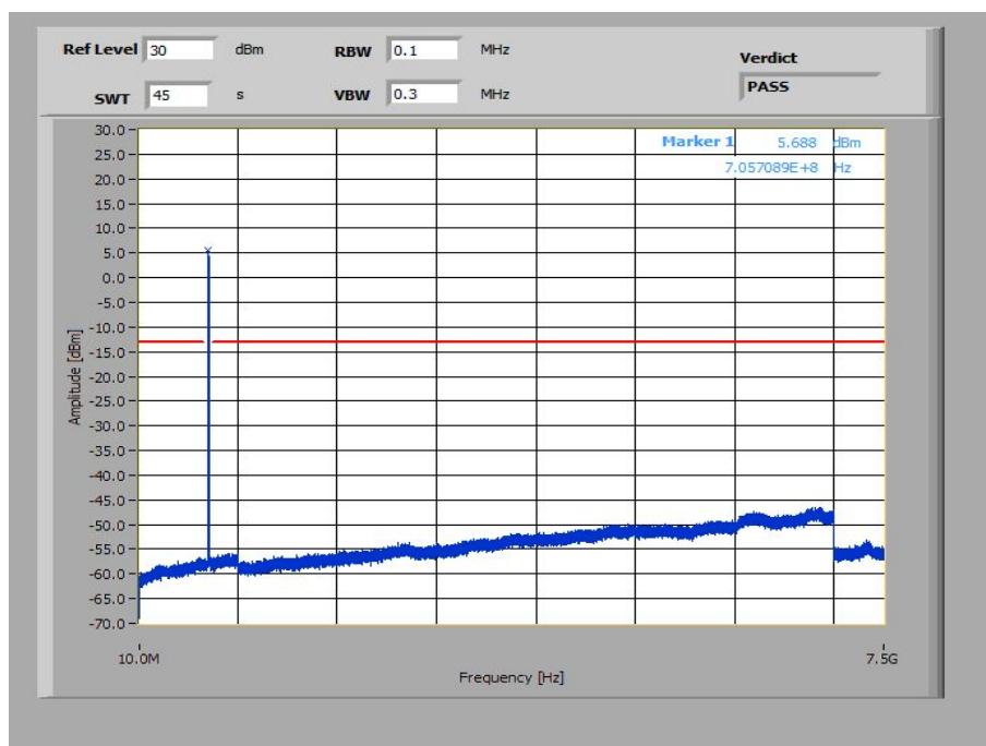
Plot 20: 5 MHz – 16-QAM - Middle Channel (10 MHz – 7.5 GHz)
