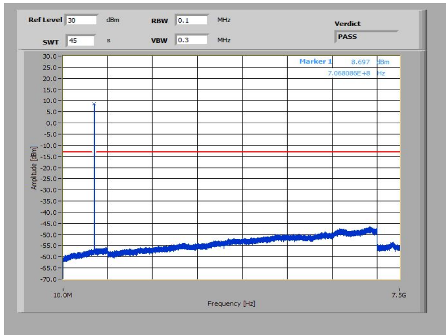
Plot 5: 3 MHz – QPSK - Middle Channel (10 MHz – 7.5 GHz)
