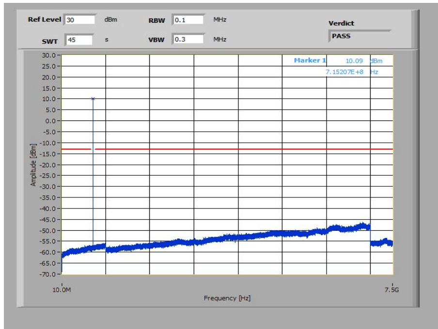
Plot 27: 1.4 MHz – 64-QAM - Highest Channel (10 MHz – 7.5 GHz)
