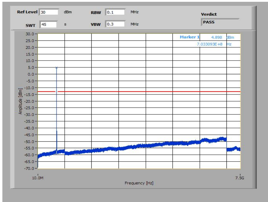
Plot 31: 5 MHz – 64-QAM - Lowest Channel (10 MHz – 7.5 GHz)
