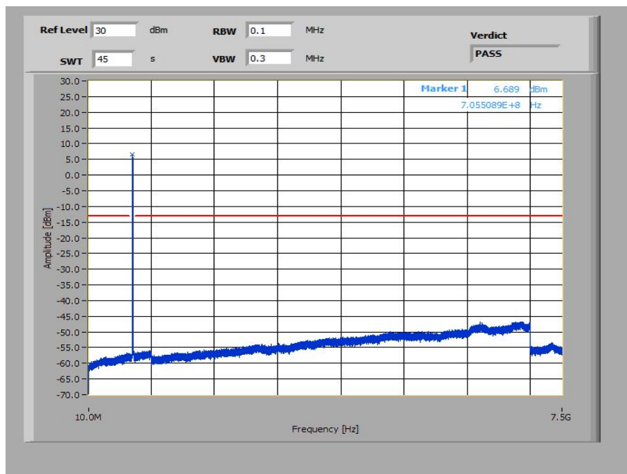
Plot 8: 5 MHz – QPSK - Middle Channel (10 MHz – 7.5 GHz)
