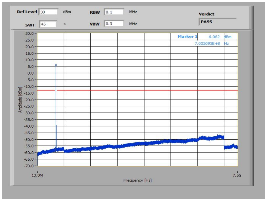
Plot 19: 5 MHz – 16-QAM - Lowest Channel (10 MHz – 7.5 GHz)
