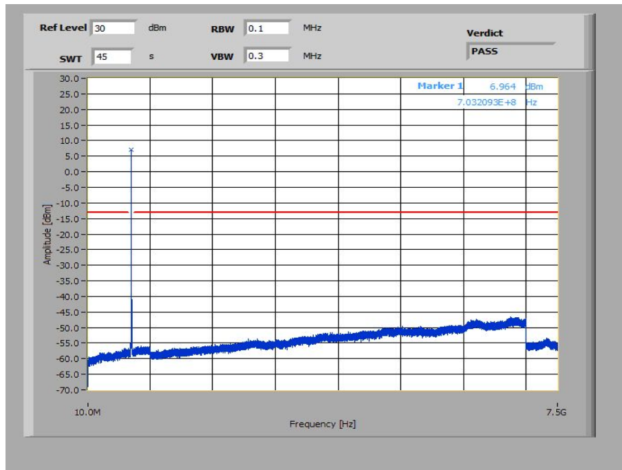
Plot 7: 5 MHz – QPSK - Lowest Channel (10 MHz – 7.5 GHz)
