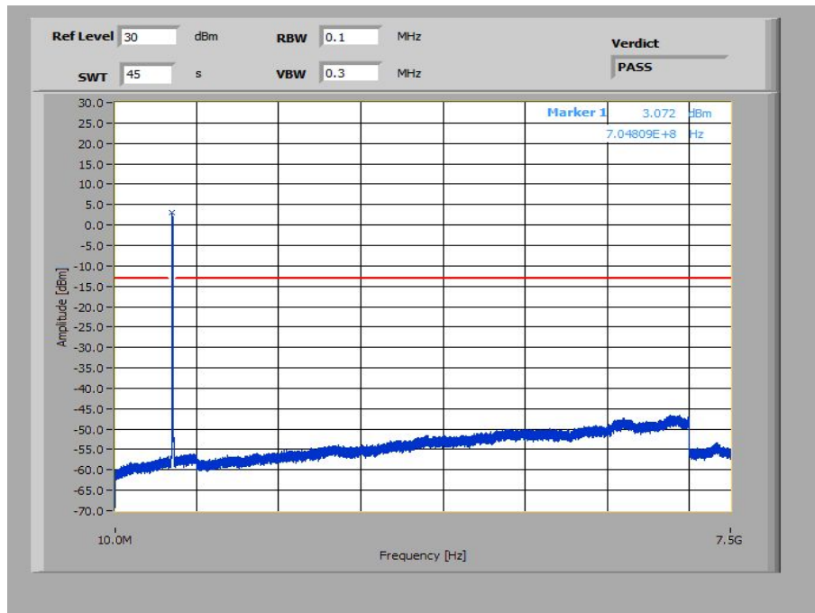
Plot 23: 10 MHz – 16-QAM - Middle Channel (10 MHz – 7.5 GHz)
