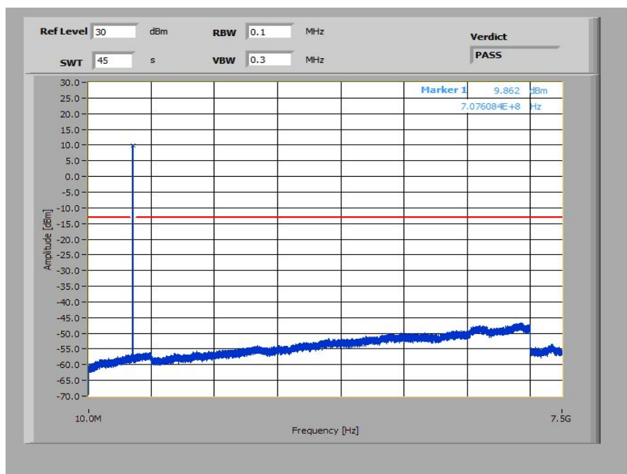
Plot 26: 1.4 MHz – 64-QAM - Middle Channel (10 MHz – 7.5 GHz)
