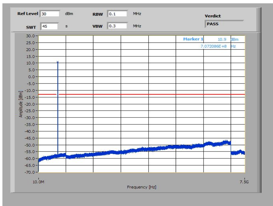
Plot 14: 1.4 MHz – 16-QAM - Middle Channel (10 MHz – 7.5 GHz)
