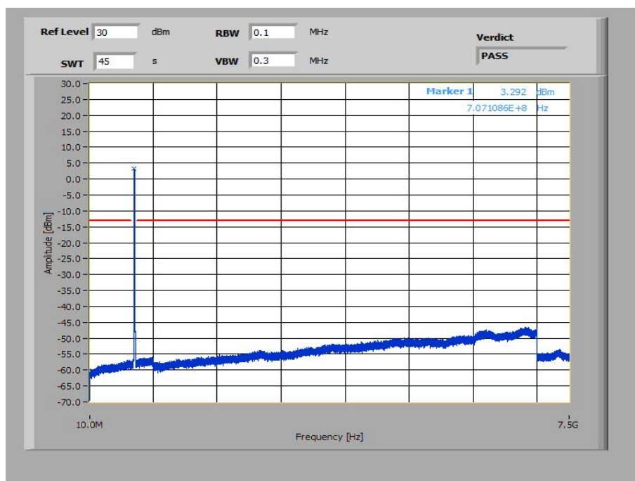
Plot 24: 10 MHz – 16-QAM - Highest Channel (10 MHz – 7.5 GHz)
