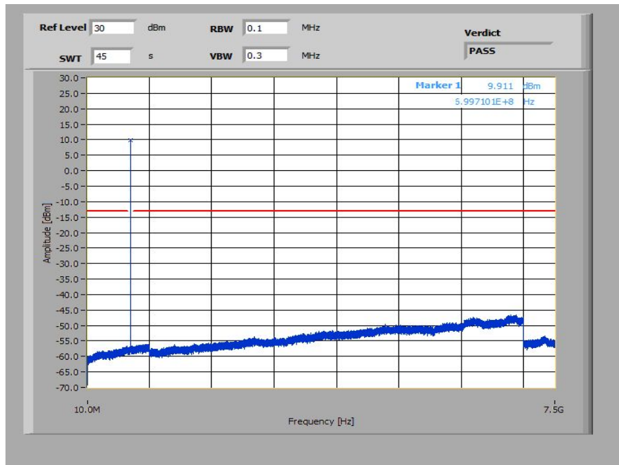
Plot 25: 1.4 MHz – 64-QAM - Lowest Channel (10 MHz – 7.5 GHz)
