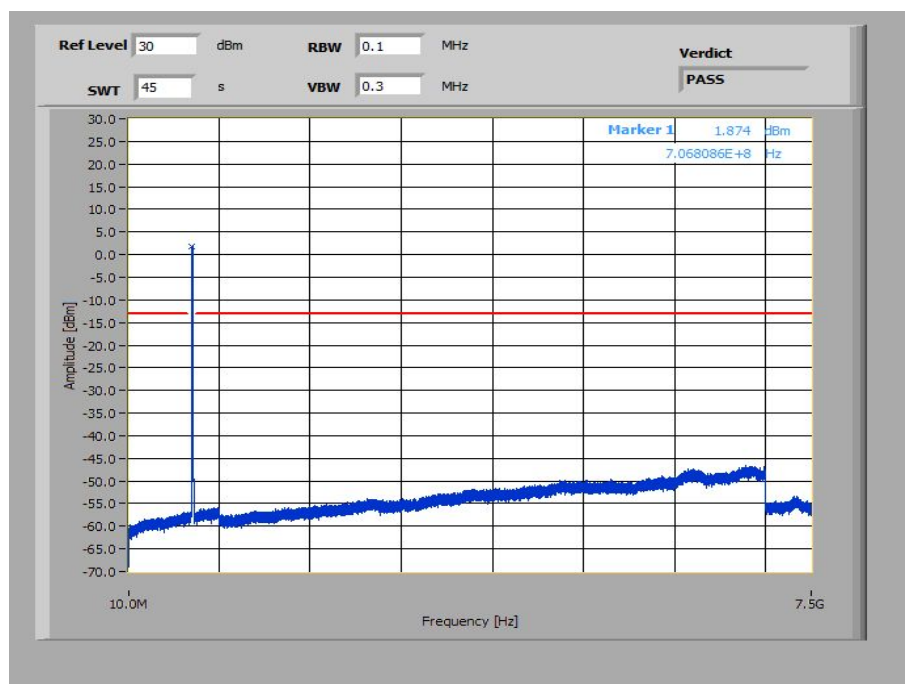
Plot 36: 10 MHz – 64-QAM - Highest Channel (10 MHz – 7.5 GHz)
