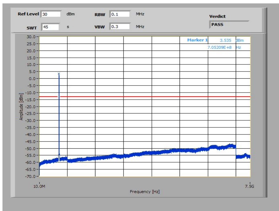
Plot 10: 10 MHz – QPSK - Lowest Channel (10 MHz – 7.5 GHz)
