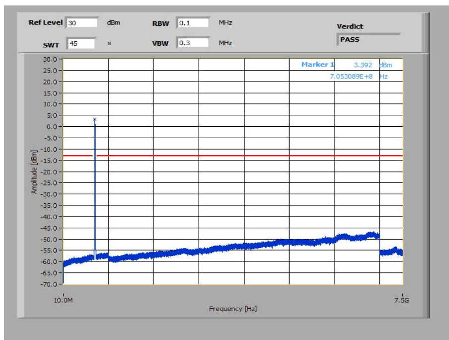
Plot 22: 10 MHz – 16-QAM - Lowest Channel (10 MHz – 7.5 GHz)
