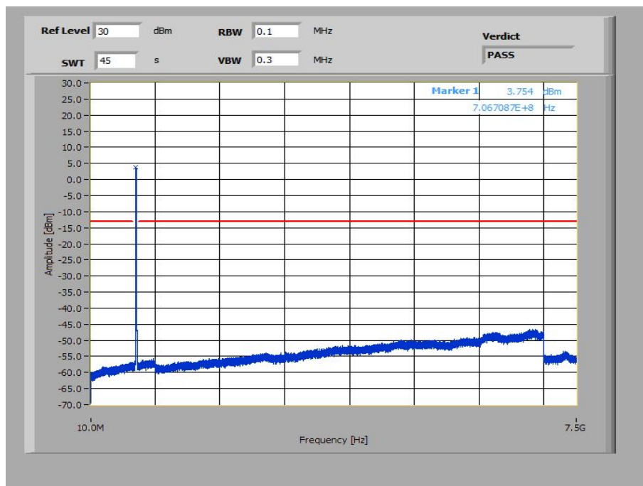
Plot 12: 10 MHz – QPSK - Highest Channel (10 MHz – 7.5 GHz)
