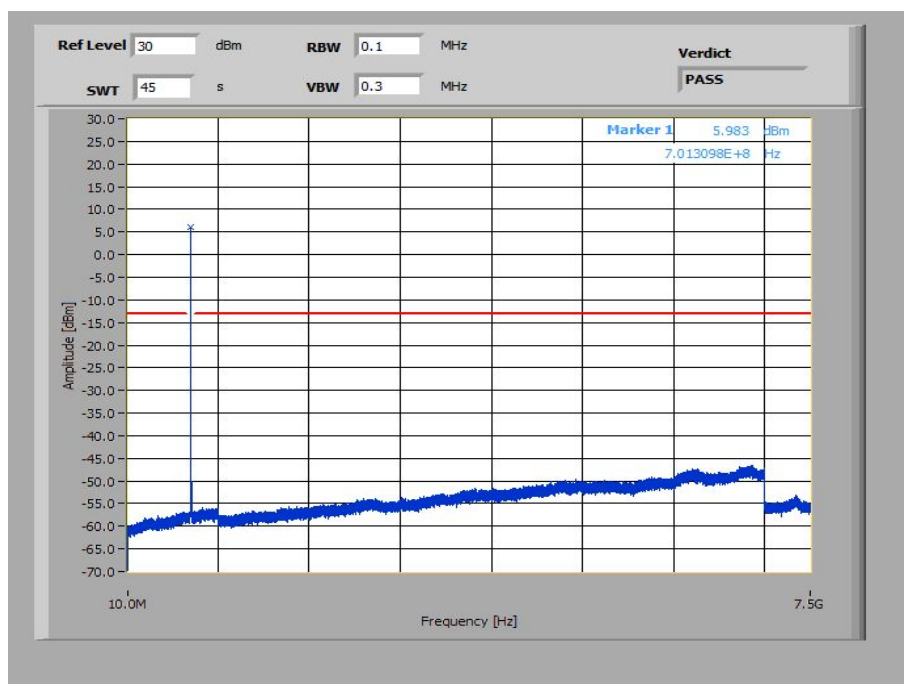
Plot 28: 3 MHz – 64-QAM - Lowest Channel (10 MHz – 7.5 GHz)
