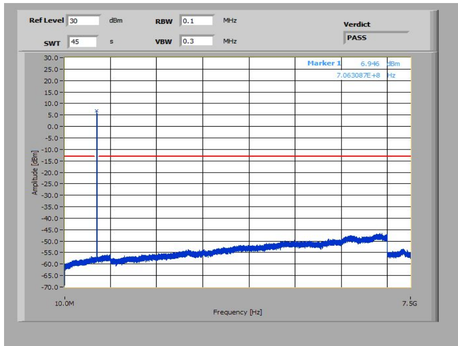
Plot 29: 3 MHz – 64-QAM - Middle Channel (10 MHz – 7.5 GHz)
