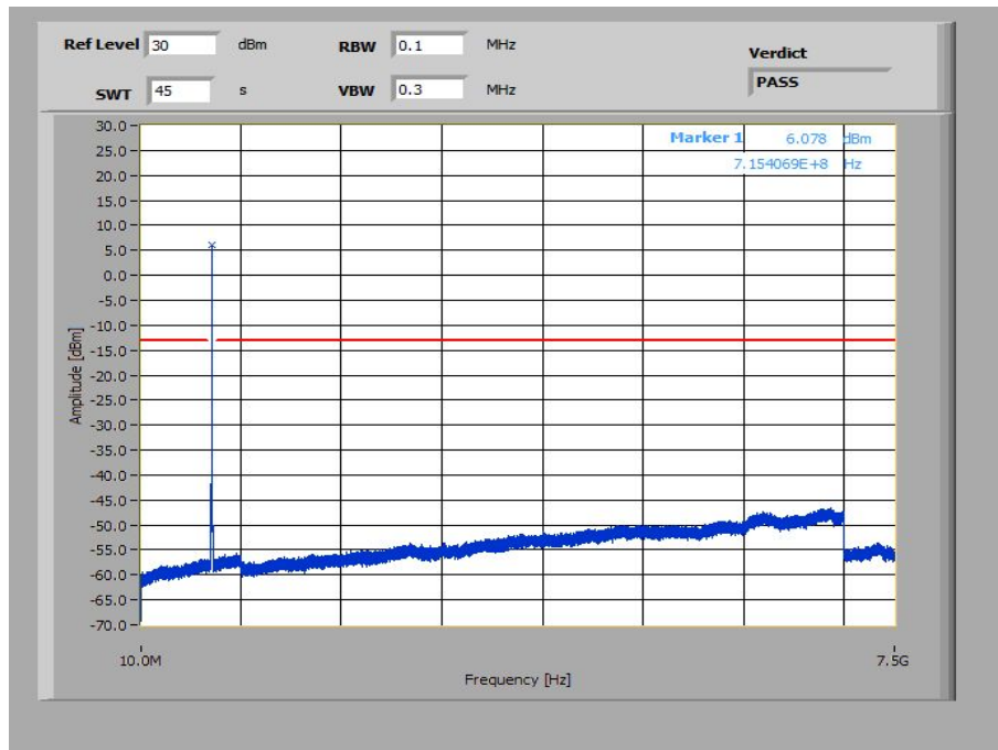
Plot 21: 5 MHz – 16-QAM - Highest Channel (10 MHz – 7.5 GHz)
