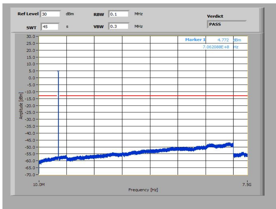
Plot 32: 5 MHz – 64-QAM - Middle Channel (10 MHz – 7.5 GHz)
