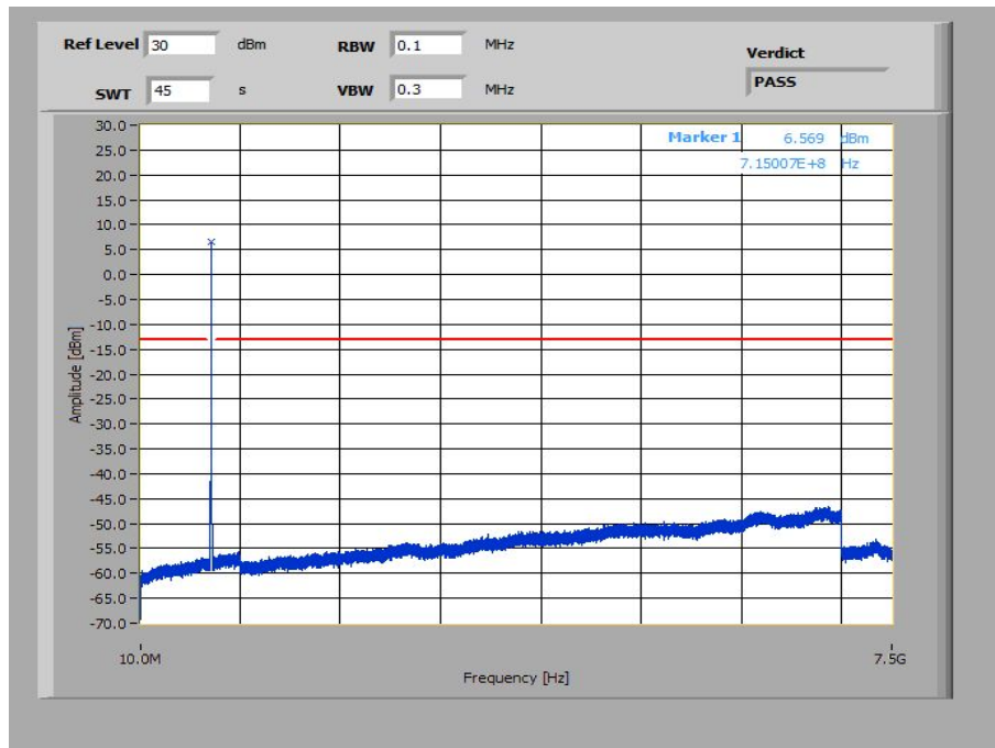
Plot 9: 5 MHz – QPSK - Highest Channel (10 MHz – 7.5 GHz)
