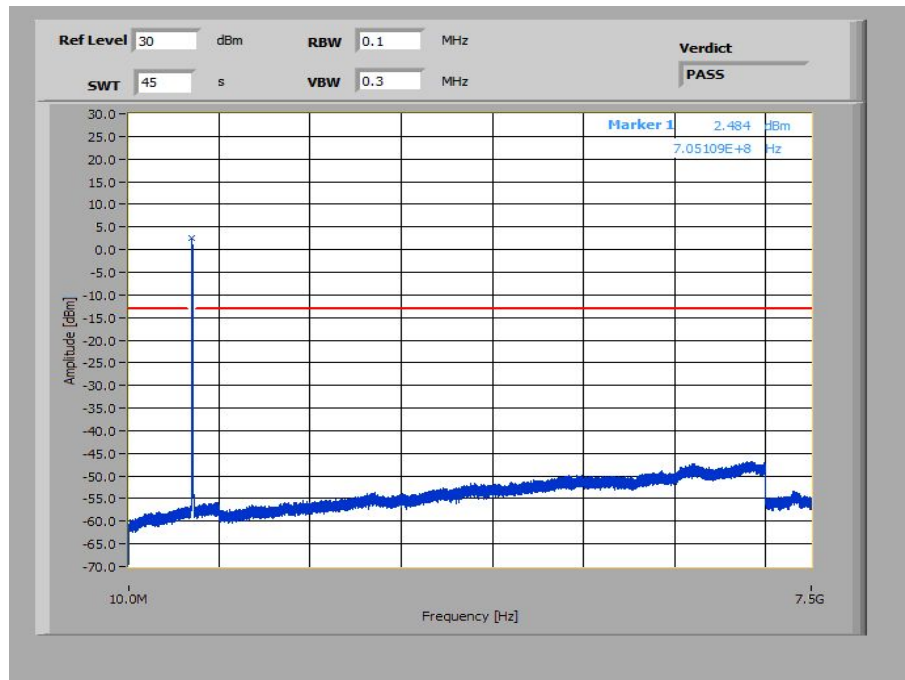
Plot 35: 10 MHz – 64-QAM - Middle Channel (10 MHz – 7.5 GHz)
