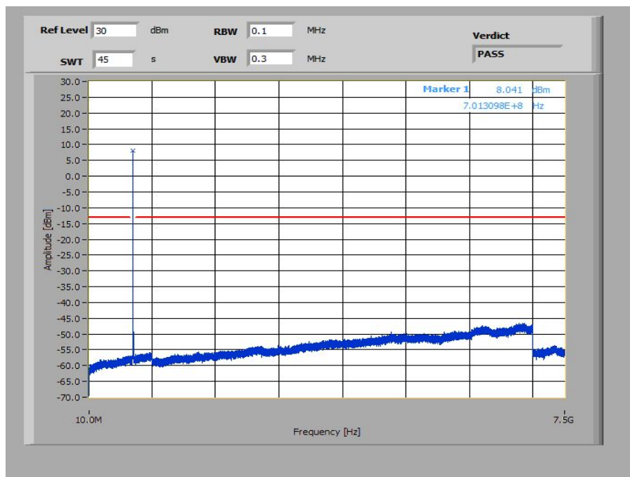
Plot 16: 3 MHz – 16-QAM - Lowest Channel (10 MHz – 7.5 GHz)
