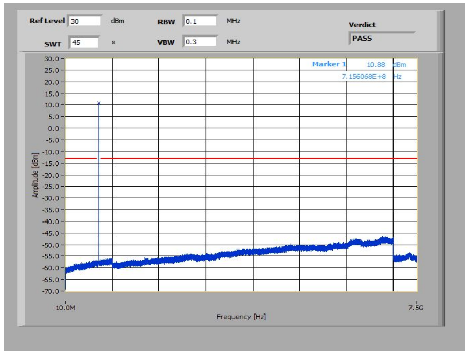
Plot 15: 1.4 MHz – 16-QAM - Highest Channel (10 MHz – 7.5 GHz)
