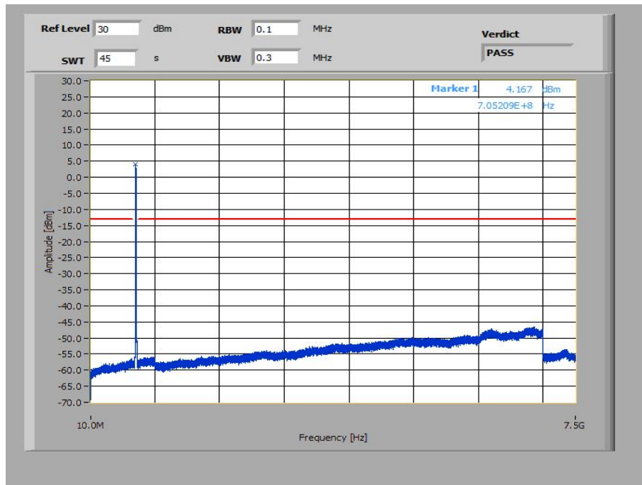
Plot 11: 10 MHz – QPSK - Middle Channel (10 MHz – 7.5 GHz)
