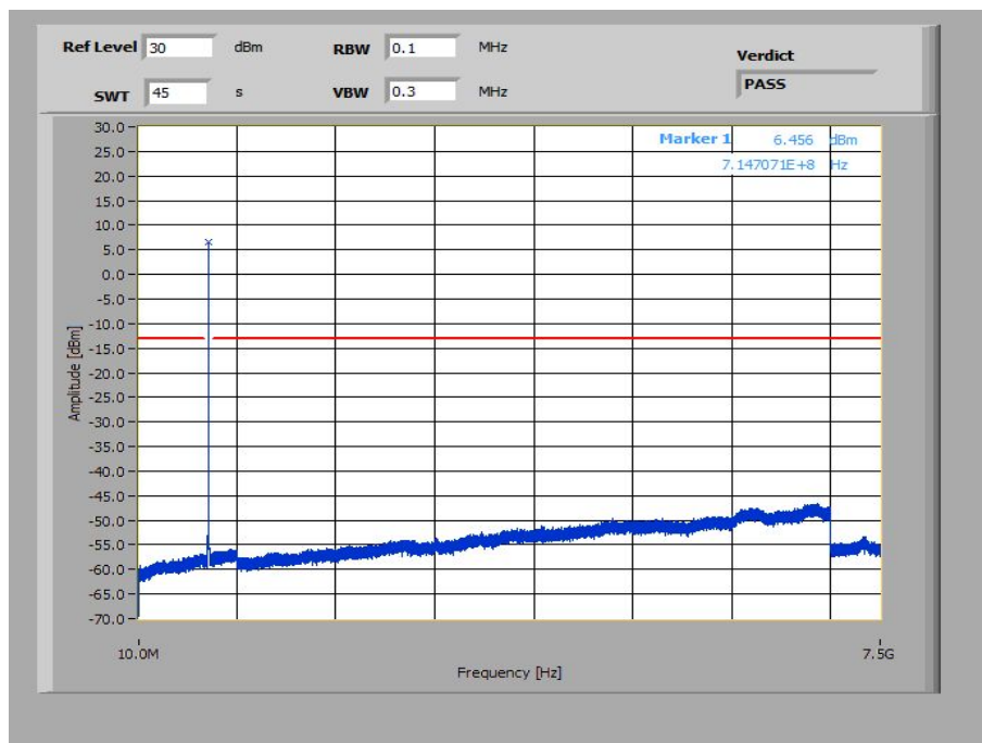
Plot 30: 3 MHz – 64-QAM - Highest Channel (10 MHz – 7.5 GHz)
