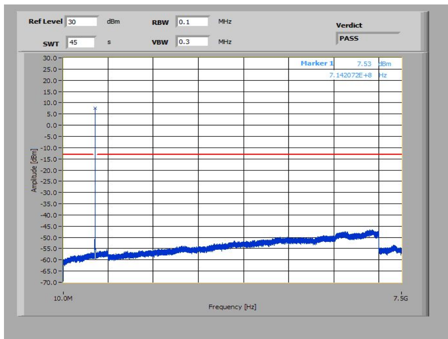
Plot 18: 3 MHz – 16-QAM - Highest Channel (10 MHz – 7.5 GHz)
