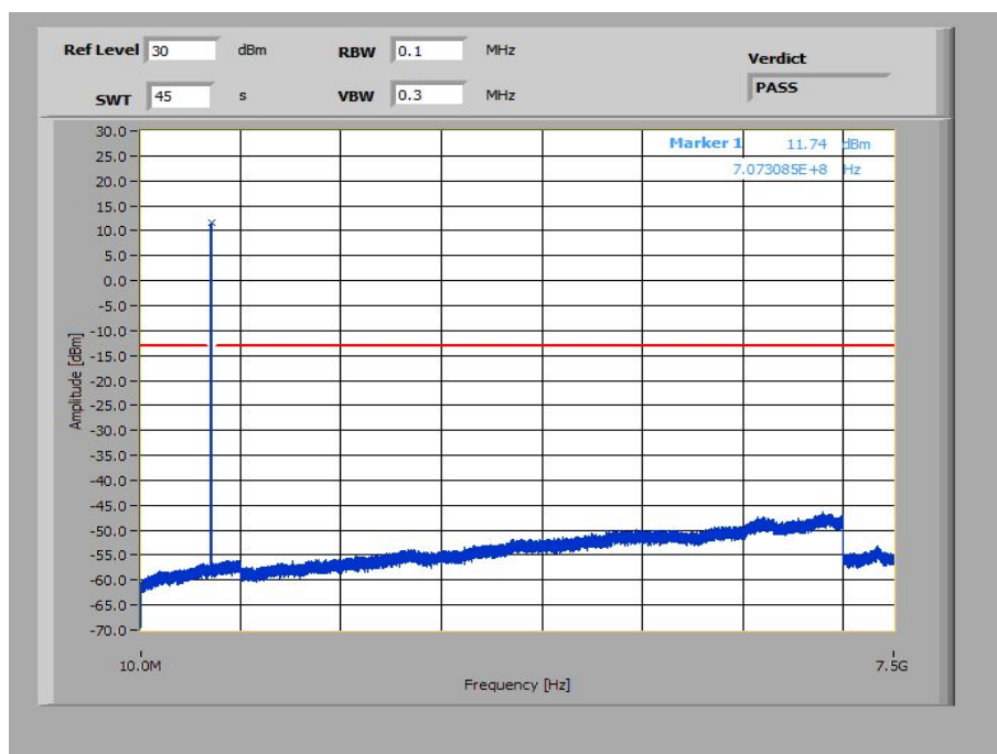
Plot 2: 1.4 MHz – QPSK - Middle Channel (10 MHz – 7.5 GHz)
