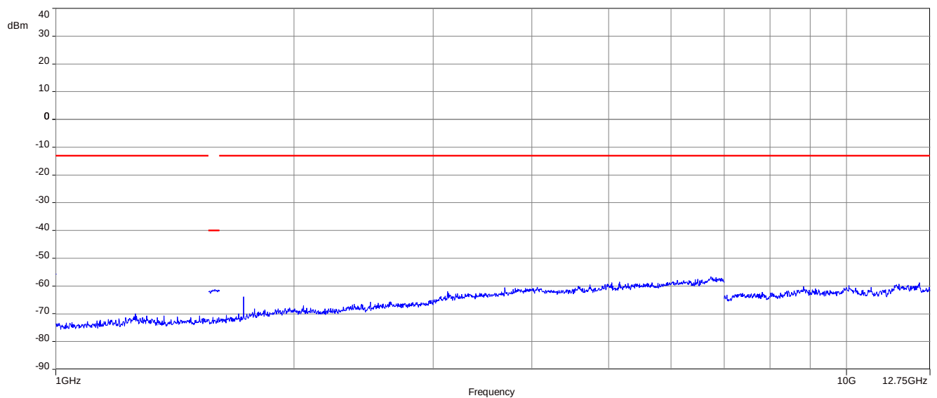
Plot 6: 16-QAM - Middle channel (1 GHz – 12.75 GHz)
