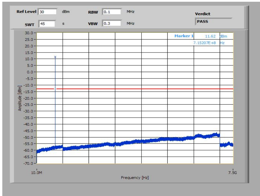
Plot 3: 1.4 MHz – QPSK - Highest Channel (10 MHz – 7.5 GHz)
