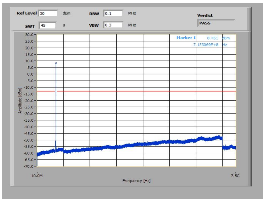
Plot 6: 3 MHz – QPSK - Highest Channel (10 MHz – 7.5 GHz)
