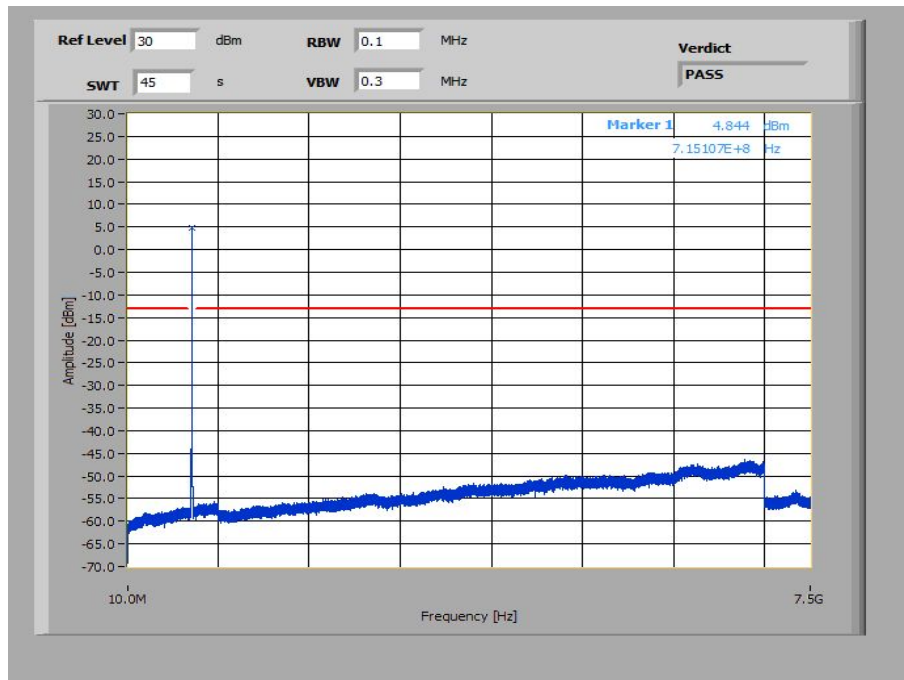
Plot 33: 5 MHz – 64-QAM - Highest Channel (10 MHz – 7.5 GHz)
