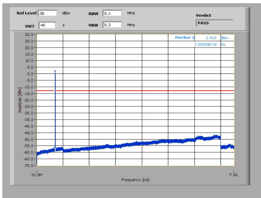
Plot 34: 10 MHz – 64-QAM - Lowest Channel (10 MHz – 7.5 GHz)
