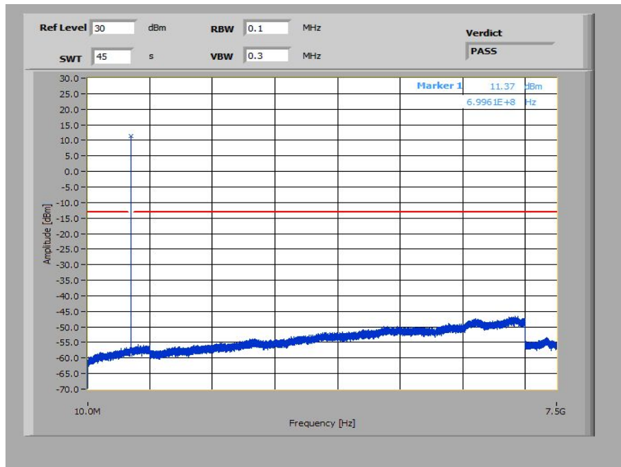
Plot 13: 1.4 MHz – 16-QAM - Lowest Channel (10 MHz – 7.5 GHz)
