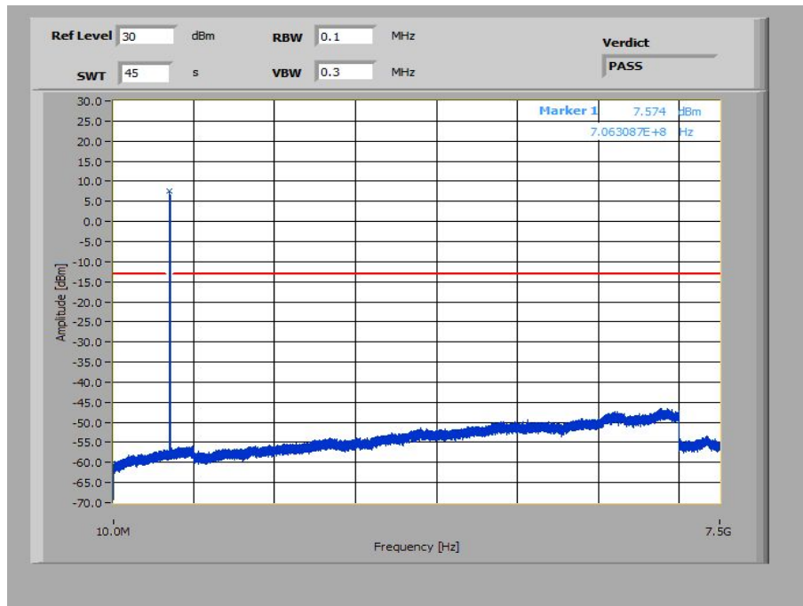
Plot 17: 3 MHz – 16-QAM - Middle Channel (10 MHz – 7.5 GHz)
