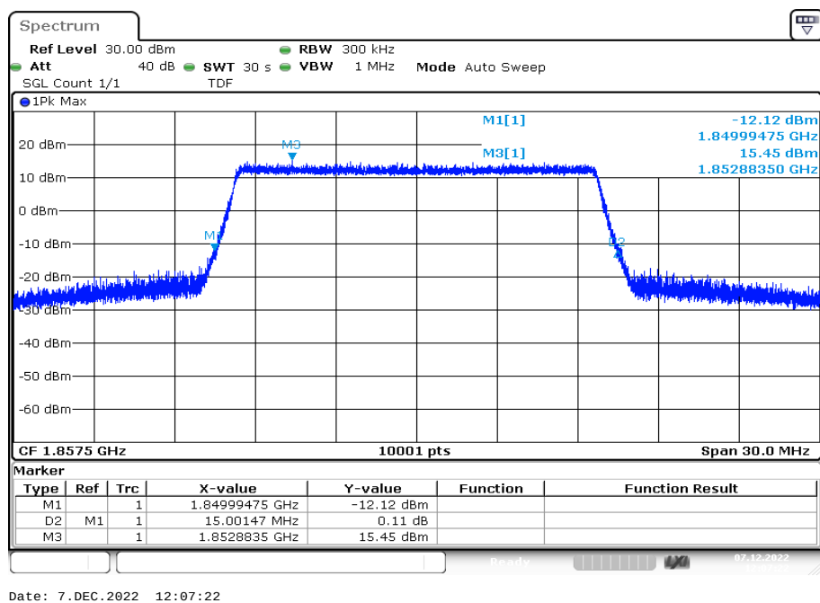
Plot 98: 15 MHz – 64-QAM - lowest channel (-26 dBc BW)
