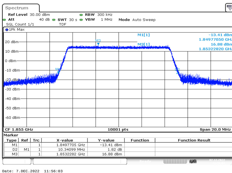
Plot 92: 10 MHz – 64-QAM - lowest channel (-26 dBc BW)
