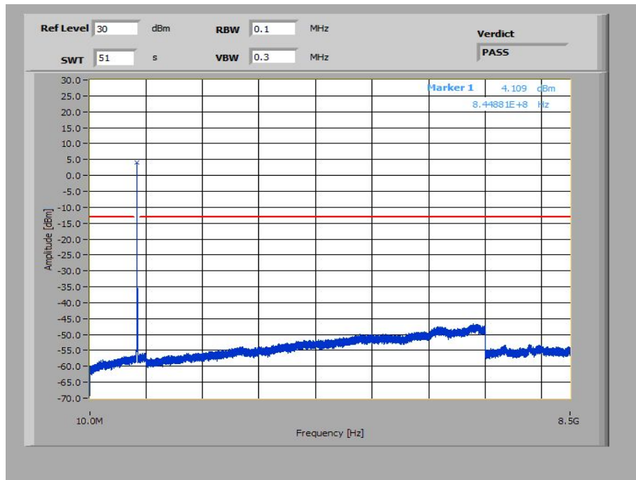
Plot 39: 5 MHz – 64-QAM - Highest Channel (10 MHz – 8.5 GHz)
