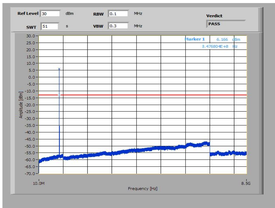
Plot 36: 3 MHz – 64-QAM - Highest Channel (10 MHz – 8.5 GHz)
