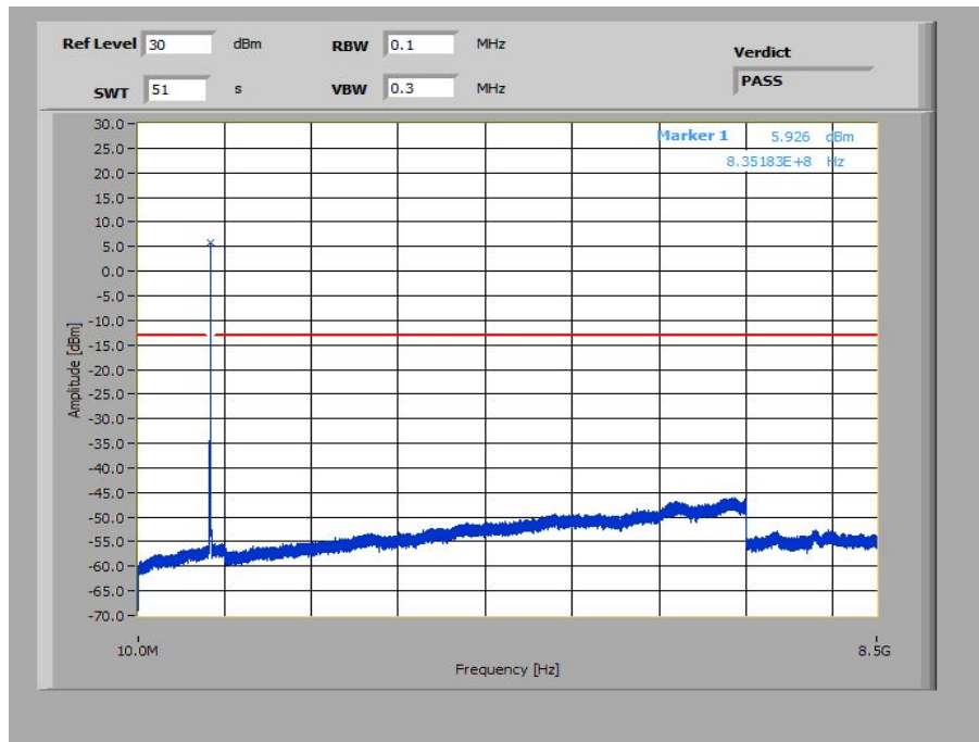
Plot 23: 5 MHz – 16-QAM - Middle Channel (10 MHz – 8.5 GHz)
