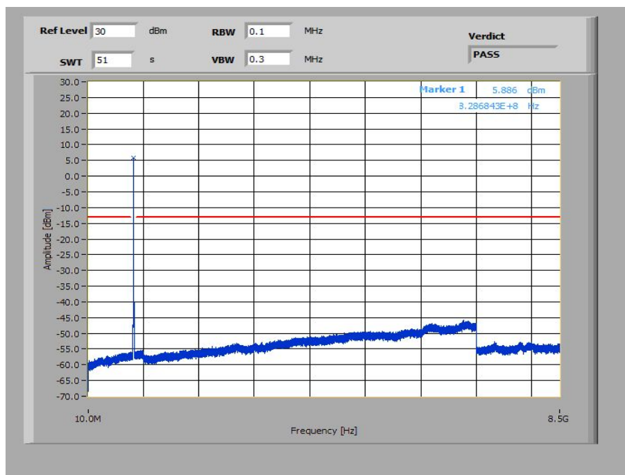
Plot 22: 5 MHz – 16-QAM - Lowest Channel (10 MHz – 8.5 GHz)
