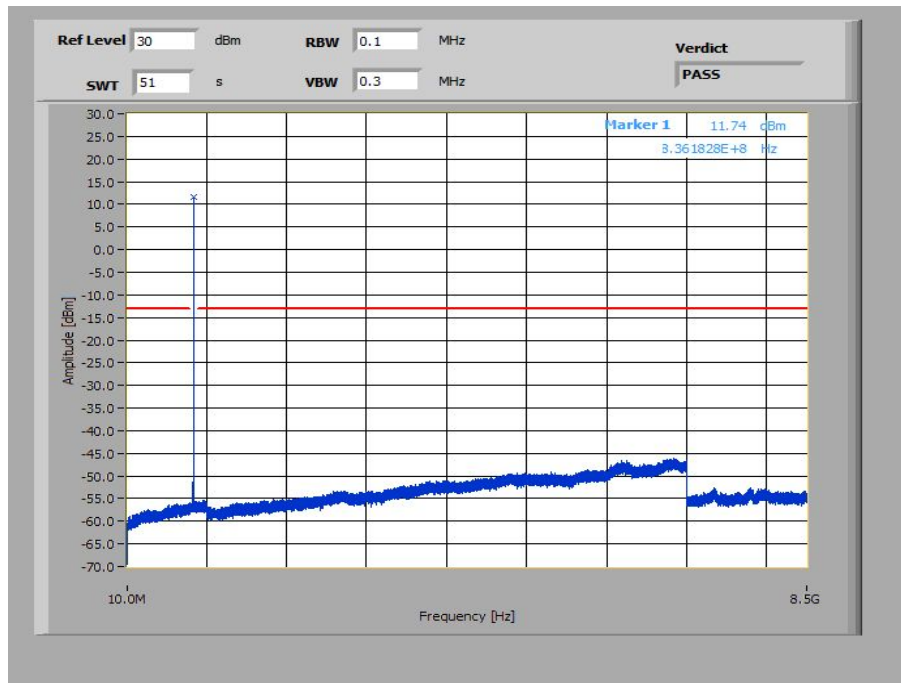
Plot 17: 1.4 MHz – 16-QAM - Middle Channel (10 MHz – 8.5 GHz)
