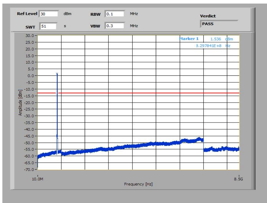
Plot 28: 15 MHz – 16-QAM - Lowest Channel (10 MHz – 8.5 GHz)
