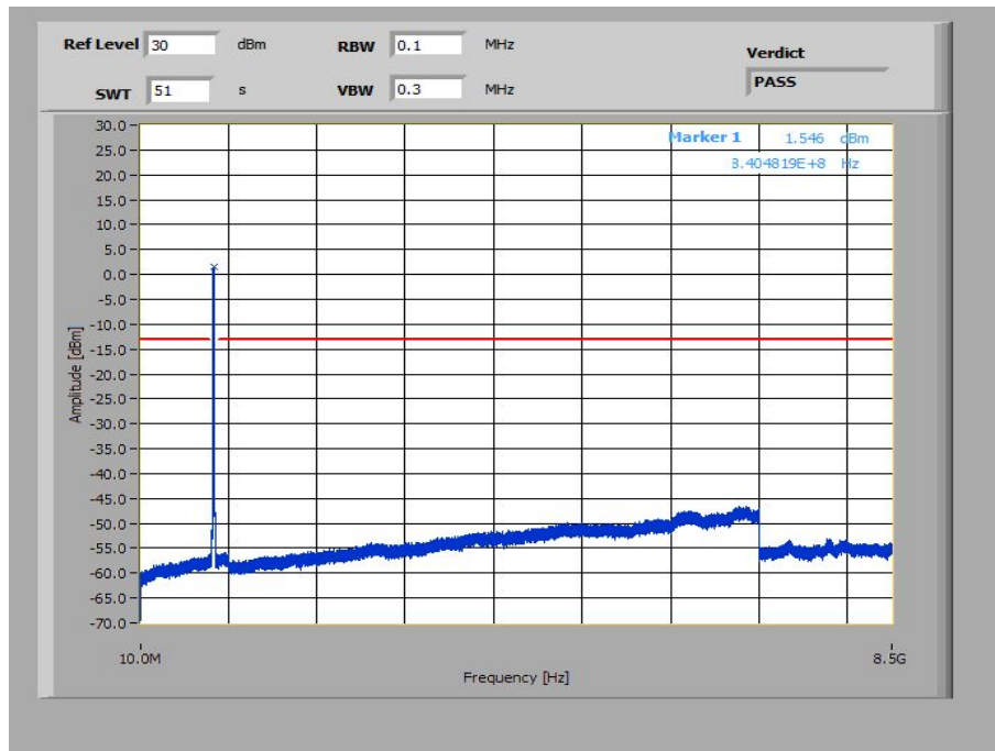
Plot 41: 10 MHz – 64-QAM - Middle Channel (10 MHz – 8.5 GHz)
