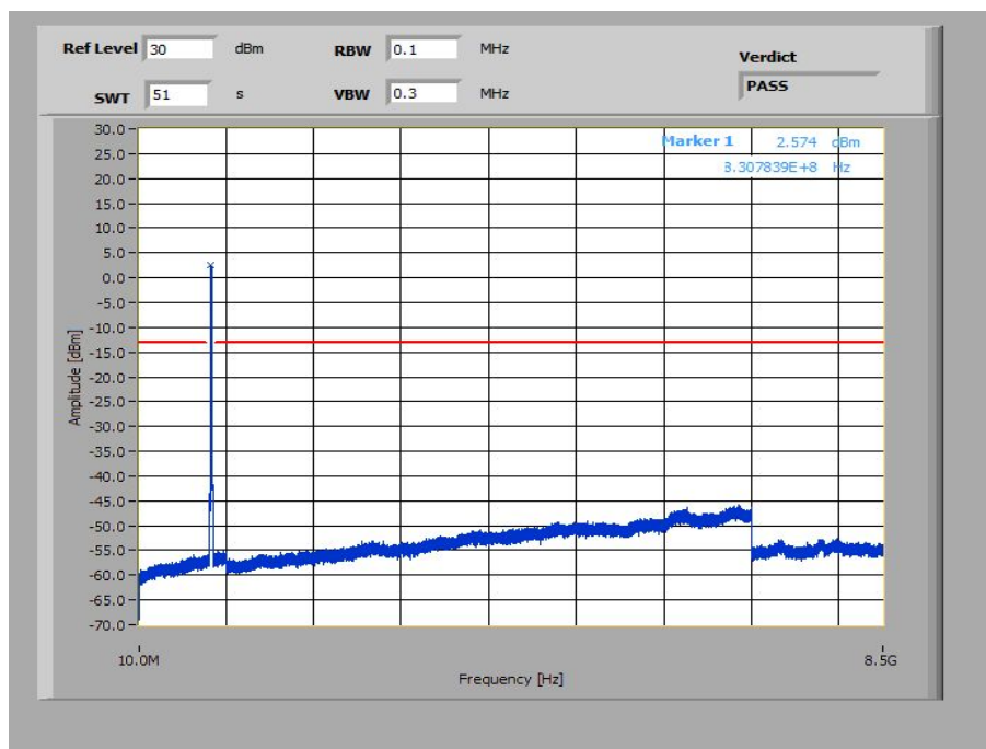
Plot 14: 15 MHz – QPSK - Middle Channel (10 MHz – 8.5 GHz)
