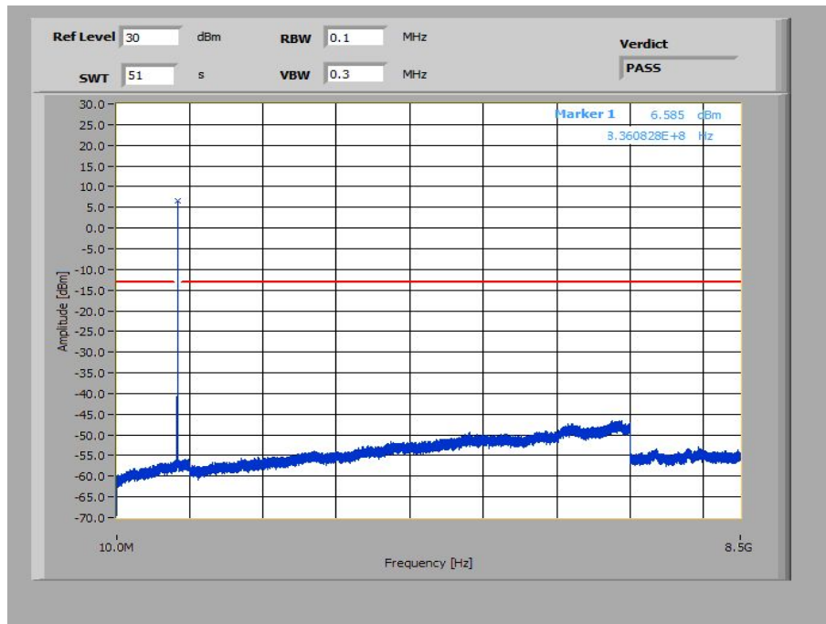
Plot 35: 3 MHz – 64-QAM - Middle Channel (10 MHz – 8.5 GHz)
