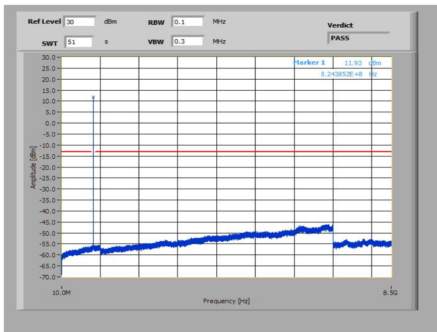
Plot 16: 1.4 MHz – 16-QAM - Lowest Channel (10 MHz – 8.5 GHz)
