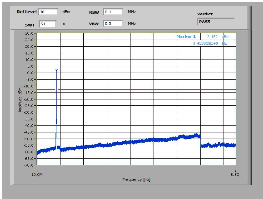
Plot 15: 15 MHz – QPSK - Highest Channel (10 MHz – 8.5 GHz)
