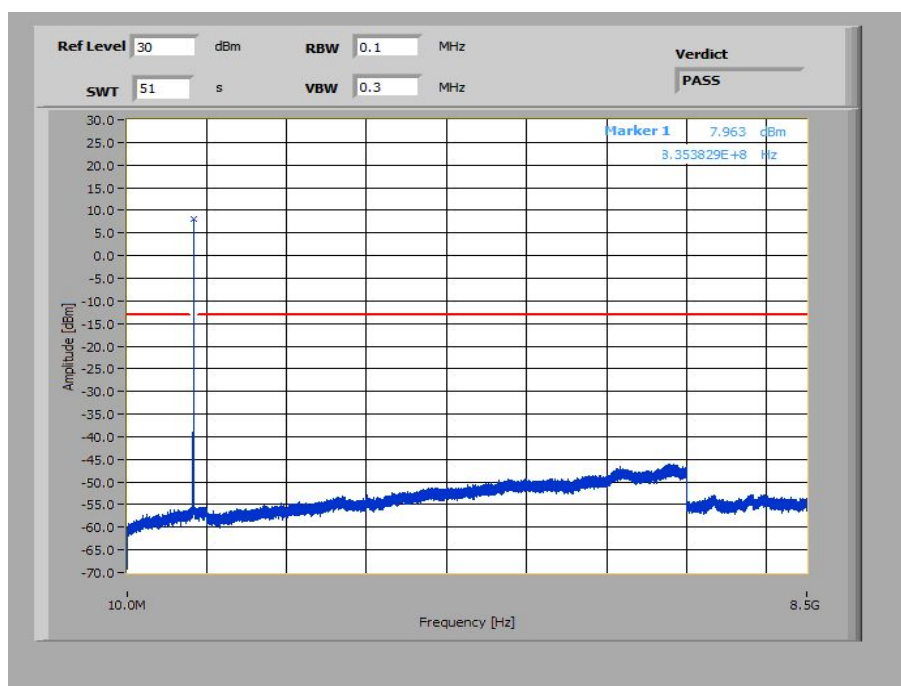
Plot 20: 3 MHz – 16-QAM - Middle Channel (10 MHz – 8.5 GHz)
