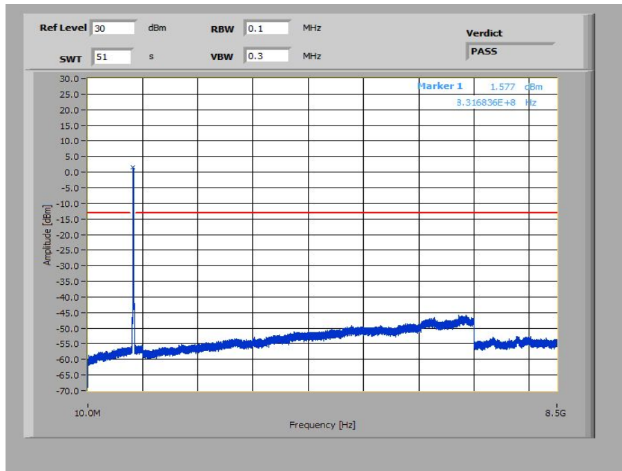
Plot 29: 15 MHz – 16-QAM - Middle Channel (10 MHz – 8.5 GHz)
