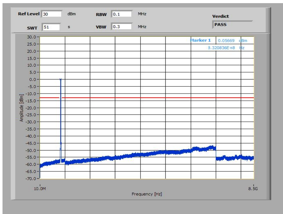
Plot 44: 15 MHz – 64-QAM - Middle Channel (10 MHz – 8.5 GHz)
