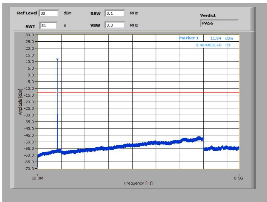
Plot 18: 1.4 MHz – 16-QAM - Highest Channel (10 MHz – 8.5 GHz)
