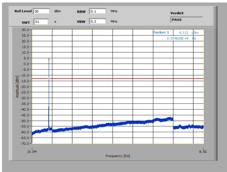
Plot 38: 5 MHz – 64-QAM - Middle Channel (10 MHz – 8.5 GHz)
