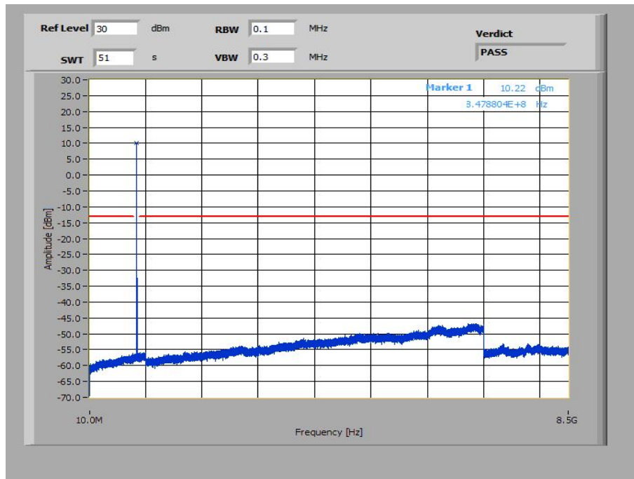
Plot 33: 1.4 MHz – 64-QAM - Highest Channel (10 MHz – 8.5 GHz)
