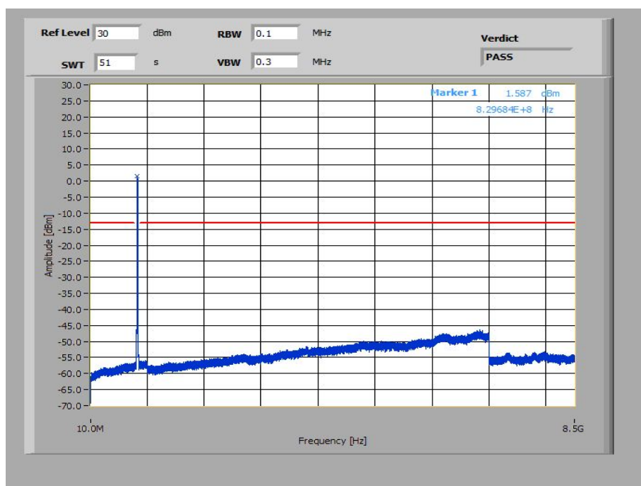
Plot 40: 10 MHz – 64-QAM - Lowest Channel (10 MHz – 8.5 GHz)
