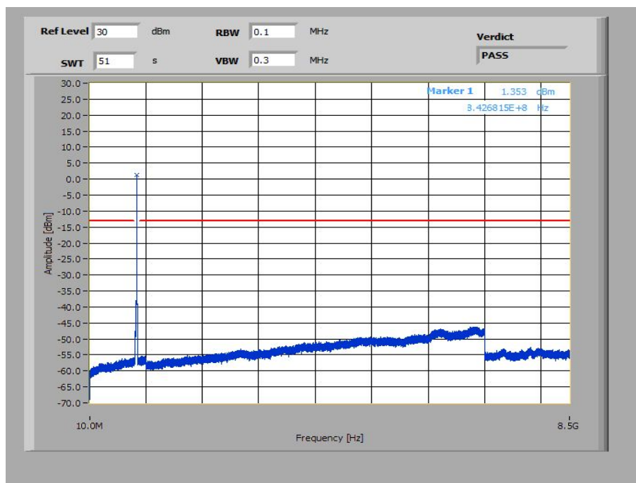
Plot 30: 15 MHz – 16-QAM - Highest Channel (10 MHz – 8.5 GHz)
