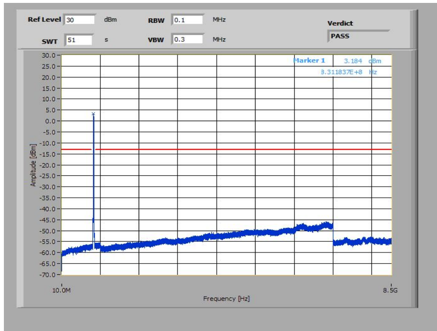
Plot 25: 10 MHz – 16-QAM - Lowest Channel (10 MHz – 8.5 GHz)
