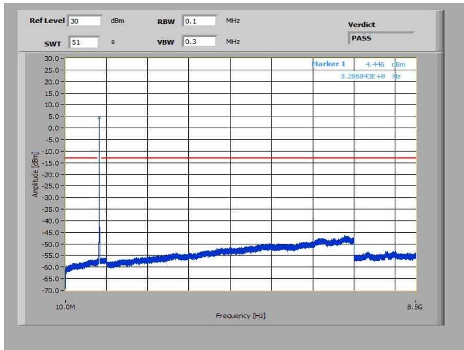
Plot 37: 5 MHz – 64-QAM - Lowest Channel (10 MHz – 8.5 GHz)
