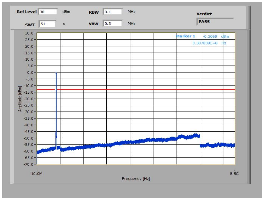
Plot 43: 15 MHz – 64-QAM - Lowest Channel (10 MHz – 8.5 GHz)
