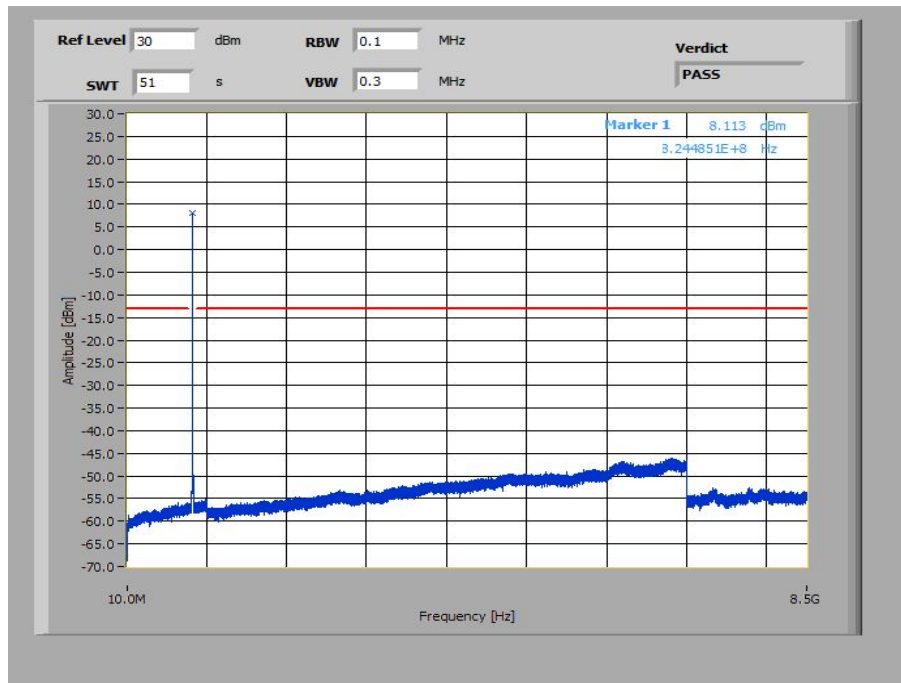
Plot 19: 3 MHz – 16-QAM - Lowest Channel (10 MHz – 8.5 GHz)
