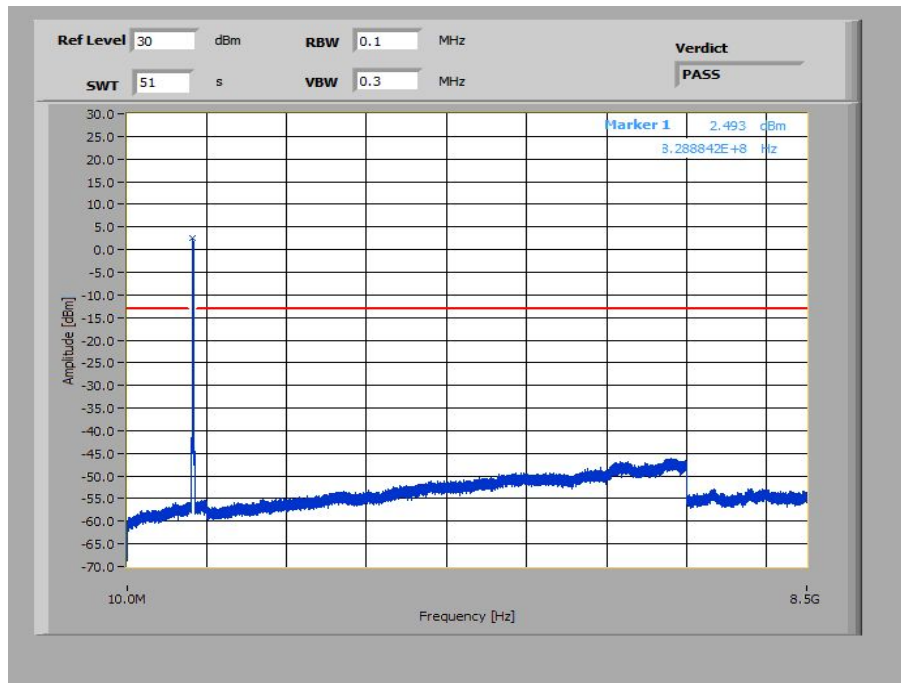
Plot 13: 15 MHz – QPSK - Lowest Channel (10 MHz – 8.5 GHz)
