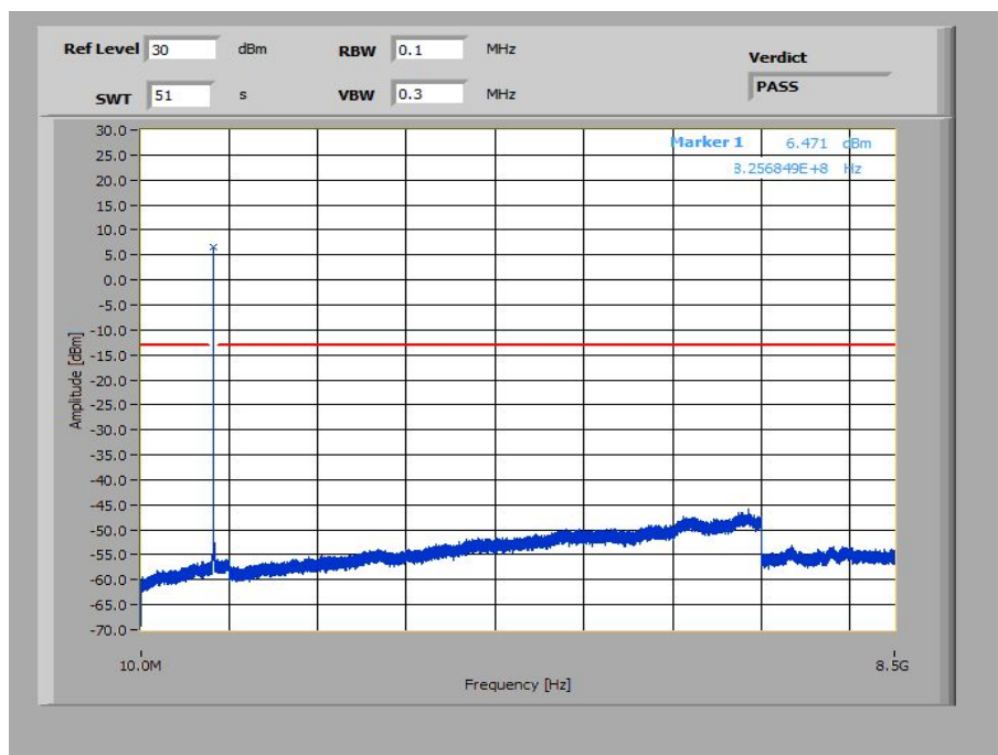
Plot 34: 3 MHz – 64-QAM - Lowest Channel (10 MHz – 8.5 GHz)
