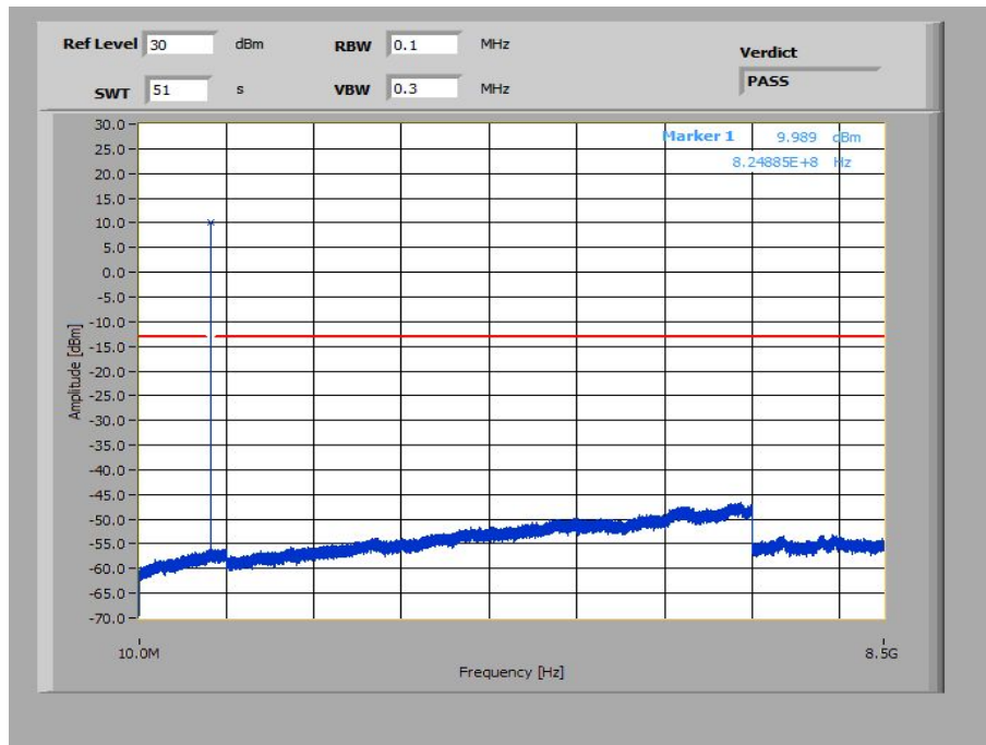
Plot 31: 1.4 MHz – 64-QAM - Lowest Channel (10 MHz – 8.5 GHz)
