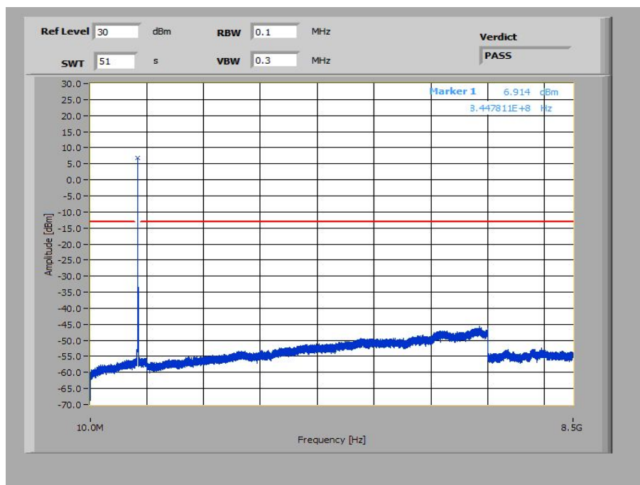
Plot 24: 5 MHz – 16-QAM - Highest Channel (10 MHz – 8.5 GHz)
