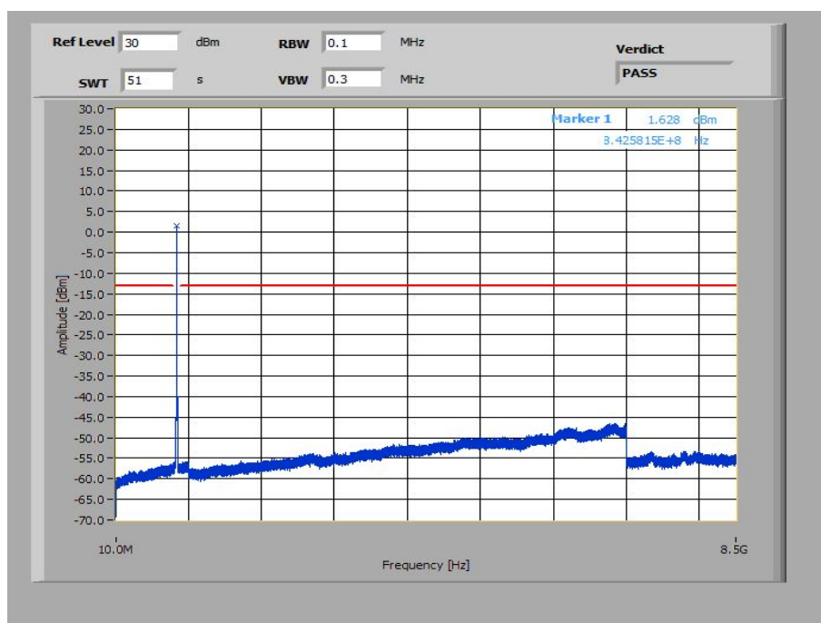
Plot 42: 10 MHz – 64-QAM - Highest Channel (10 MHz – 8.5 GHz)
