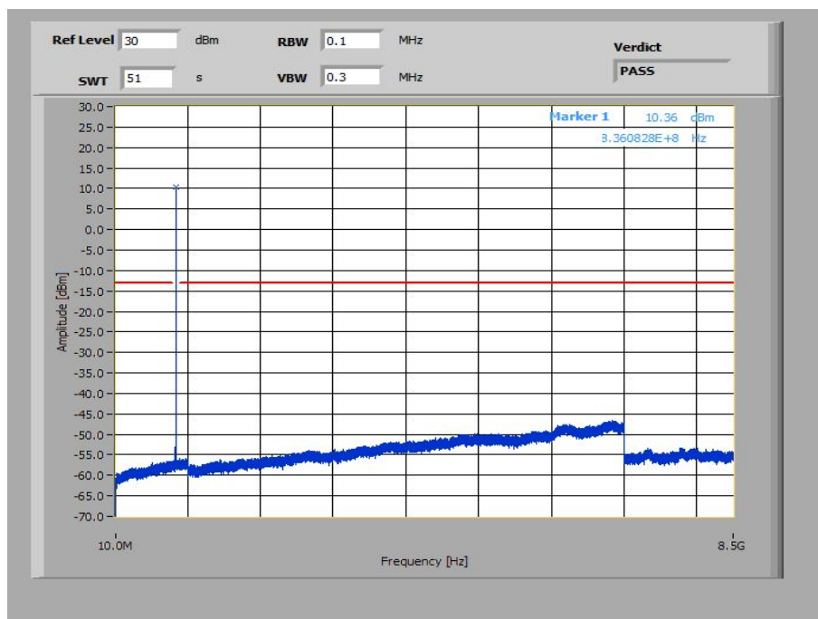
Plot 32: 1.4 MHz – 64-QAM - Middle Channel (10 MHz – 8.5 GHz)
