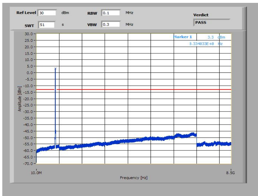
Plot 26: 10 MHz – 16-QAM - Middle Channel (10 MHz – 8.5 GHz)
