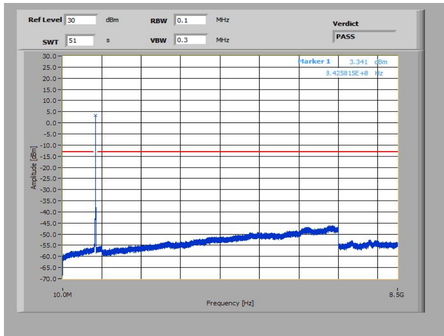
Plot 27: 10 MHz – 16-QAM - Highest Channel (10 MHz – 8.5 GHz)
