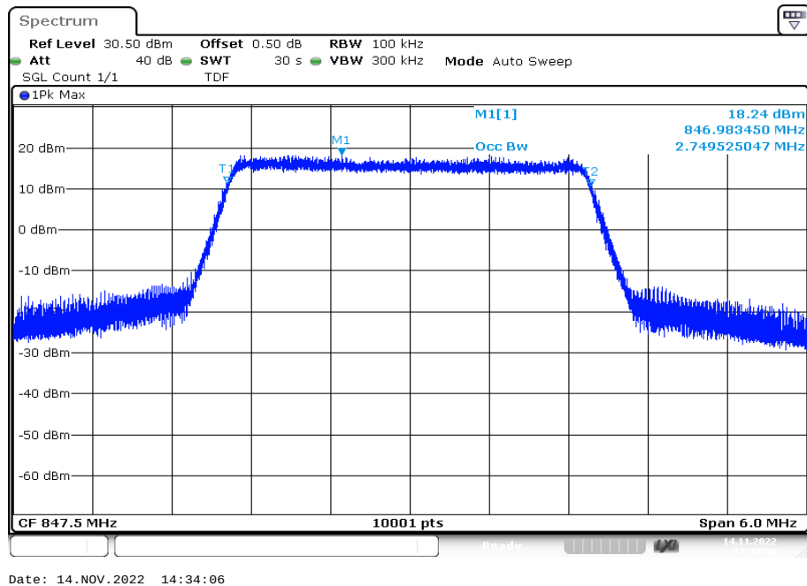
Plot 41: 3 MHz – 16-QAM - highest channel (99% - OBW)
