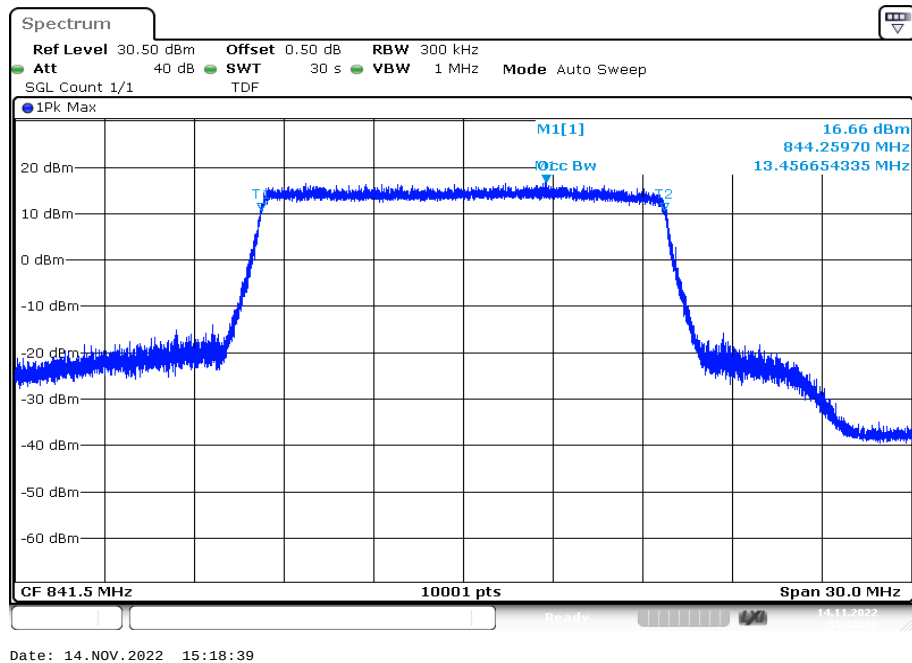
Plot 59: 15 MHz – 16-QAM - highest channel (99% - OBW)
