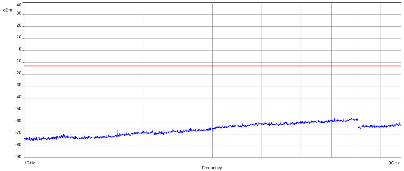
Plot 9: 64-QAM - Middle channel (1 GHz – 9 GHz)
