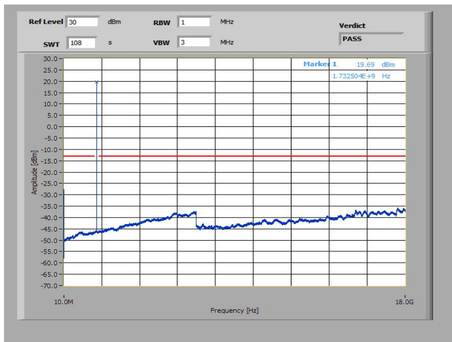
Plot 20: 1.4 MHz – 16-QAM - Middle Channel (10 MHz – 18 GHz)
