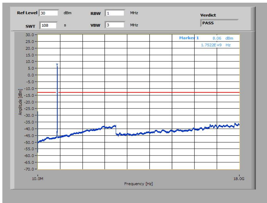
Plot 54: 20 MHz – 64-QAM - Highest Channel (10 MHz – 18 GHz)
