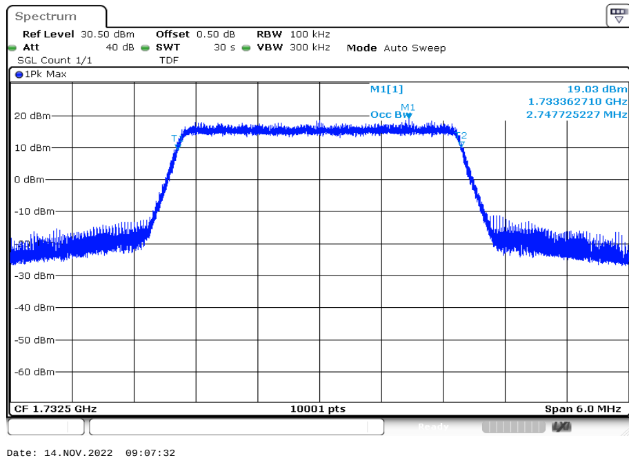
Plot 45: 3 MHz – 16-QAM - middle channel (99% - OBW)
